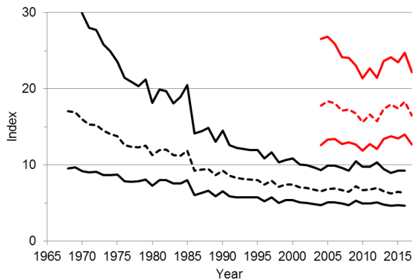
Figure 2. Abundance indices (dashed lines) and 95% credible intervals (solid lines) for the Pacific Coast population of band-tailed pigeons based on results from the North American Breeding Bird Survey (1968–2016) and Mineral Site Survey (2004–2017; scaled by dividing the index by 10).
