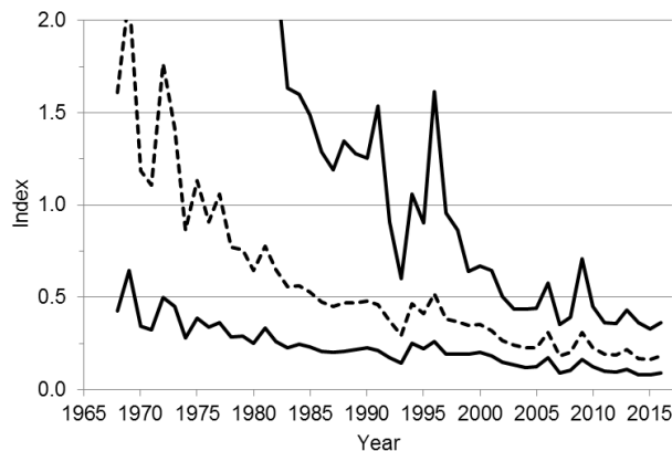
Figure 3. Abundance indices (dashed lines) and 95% credible intervals (solid lines) for the Interior population of band-tailed pigeons based on results from the North American Breeding Bird Survey, 1968–2016.
