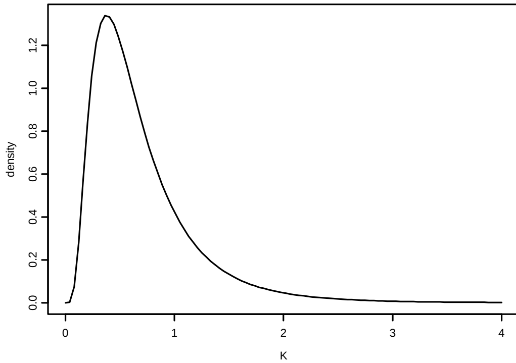
Fig. 8. Prior distribution of K in the logistic model for California-Oregon mallards.
