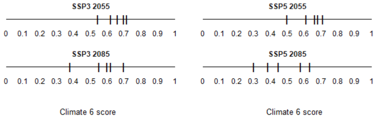
Figure A2. Comparison of projected future Climate 6 scores for Limnoperna fortunei in the contiguous United States for each of five global climate models under four combinations of Shared Socioeconomic Pathway (SSP) and time step. SSPs used (from left to right): SSP3, SSP5 (Karger et al. 2017, 2018; IPCC 2021). Time steps: 2055 (top row) and 2085 (bottom row). Climate source data from CHELSA (Karger et al. 2017, 2018); global climate models used: GFDL-ESM4, UKESM1-0-LL, MPI-ESM1-2-HR, IPSL-CM6A-LR, and MRI-ESM2-0.
