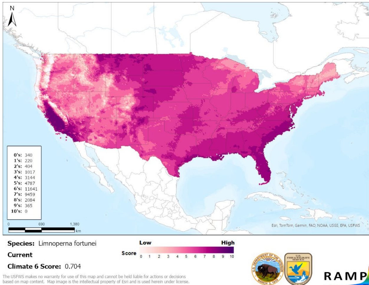
Figure 4. Map of RAMP (Sanders et al. 2023) climate matches for Limnoperna fortunei in the contiguous United States based on source locations reported by GBIF Secretariat (2023) and USGS (2025). Counts of climate match scores are tabulated on the left. 0/Pale Pink = Lowest match, 10/Dark Purple = Highest match.
