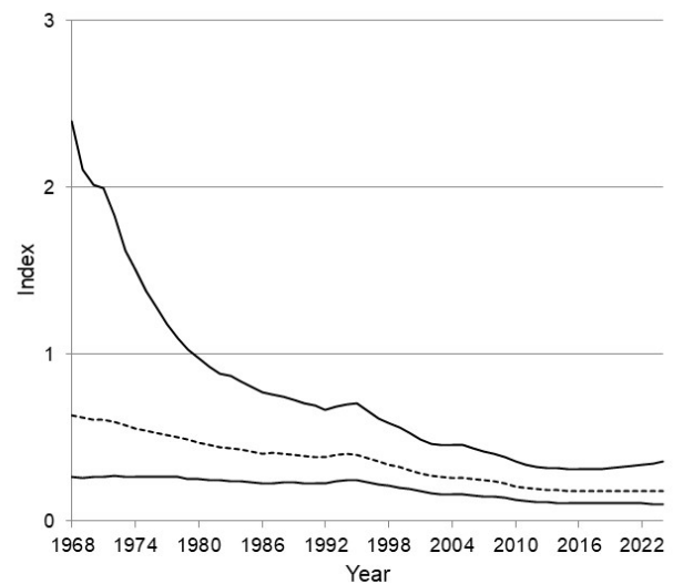
Figure 3. Abundance indices (dashed lines) and 95% credible intervals (solid lines) for the Interior population of band-tailed pigeons based on results from the North American Breeding Bird Survey, 1968–2024.
