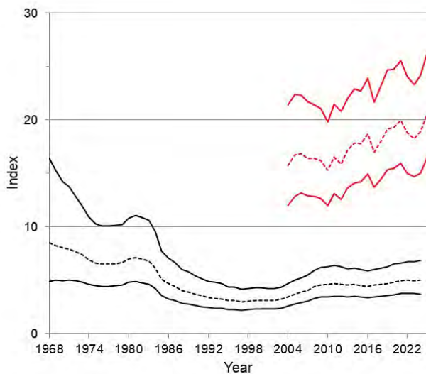
Figure 2. Abundance indices (dashed lines) and 95% credible intervals (solid lines) for the Pacific Coast population of band-tailed pigeons based on results from the North American Breeding Bird Survey (1968–2024, black lines) and Mineral Site Survey (2004–2025, red lines; scaled by dividing the index by 10).
