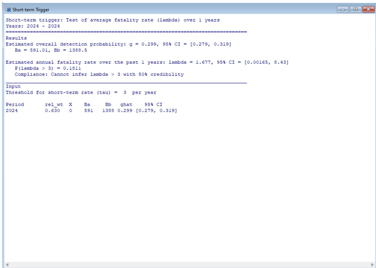
Appendix F27. Screen shot of Evidence of Absence (v2.0.7) Graphical User Interface, Multiple Years Module for estimation of northern long-eared bat rolling average detection probability and short-term adaptive management trigger test. Inputs are based on values reported in the main text.
