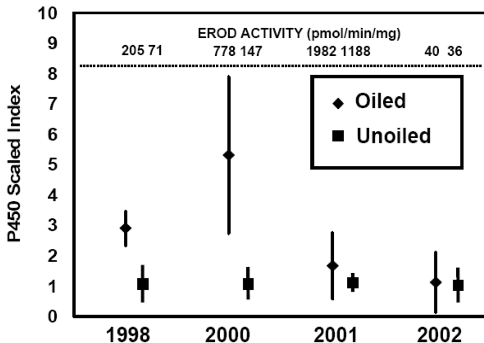
Figure 1. Cytochrome P450 (as measured by EROD activity) in harlequin ducks from oiled and unoiled areas of Prince William Sound, Alaska. The values above the dotted line are the average EROD activity reported from the lab. The figure scales the EROD data, setting the unoiled area at 1 for each year, to illustrate the change in the ratio of oiled:unoiled over time. From Elser (2005).
