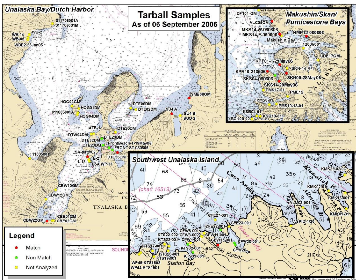
Figure 3. Results of source allocation of Tarball Samples in the vicinity of the Selendang Ayu .
