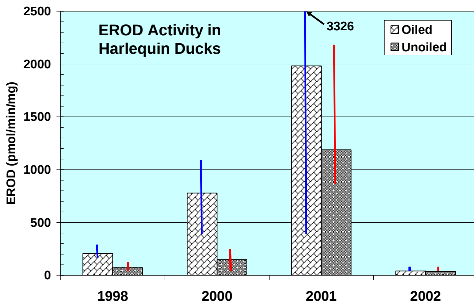
Figure 2. Mean EROD activity in tissue of harlequin ducks from oiled and unoiled locations in Prince William Sound between 1998 and 2002. This presentation shows the large inter-annual variation in EROD activity in ducks from oiled and unoiled locations.
