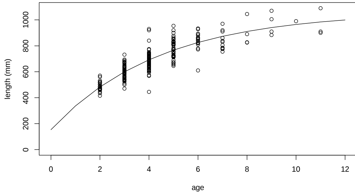
Figure 5: Predicted length-at-age of Gulf Striped Bass brood fish using a von Bertalanffy model. Growth parameters include ( L_{\infty}= 1059.43 , K= 0.23 , t_0= -0.691 ). Open circles represent collected length-at-age of Gulf Striped Bass. Line represents the predicted length-at-age for Gulf Striped Bass.
