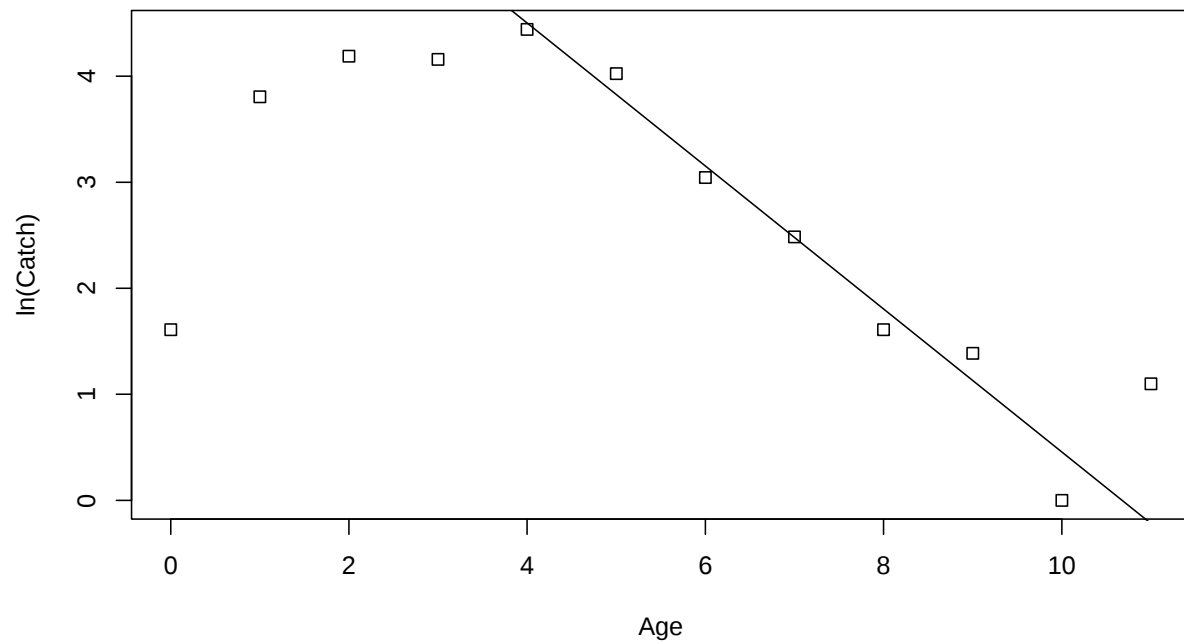
Figure 3. Log catch-at-age relation (catch-curve) of Gulf Striped Bass brood fish collected from the tailrace of the Jim Woodruff Lock and Dam, George Andrews Lock and Dam, and sections of the Flint River. Line represents the linear relation of peak catch-at-age, which was used as an estimation of total instantaneous mortality ( Z ).
