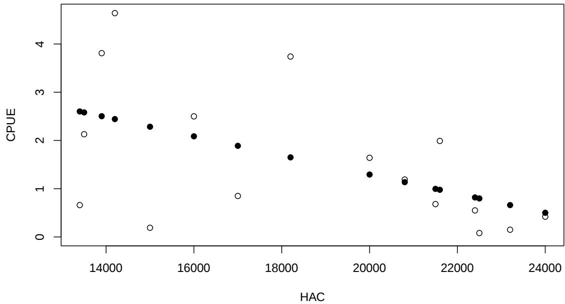
Figure 2. Linear relation between catch-per-unit-effort (CPUE) of age-0 Gulf Striped Bass and Hydrilla aerial counts (HAC) in Lake Seminole ( P= 0.03 ; r^2= 0.27 ). Open circles (○) represent individual catch-per-unit-effort of age-0 Gulf Striped Bass and the corresponding Hydrilla aerial counts. Shaded circles (●) represent the linear relation between catch-per-unit effort of age-0 Gulf Striped Bass and Hydrilla aerial counts.
