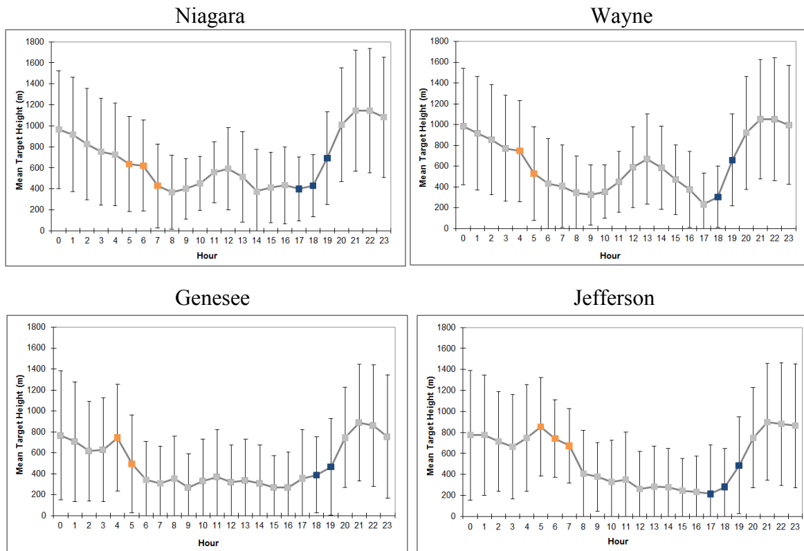
Figure 36. Hourly mean target height (m) during spring 2013 in Niagara, Wayne, Genesee, and Jefferson counties, New York. The orange and blue markers indicate the hours of sunrise and sunset, respectively. Due to differences in the survey locations and times, the hours of sunrise and sunset were not identical for all sites across the season. The error bars represent one standard deviation.
