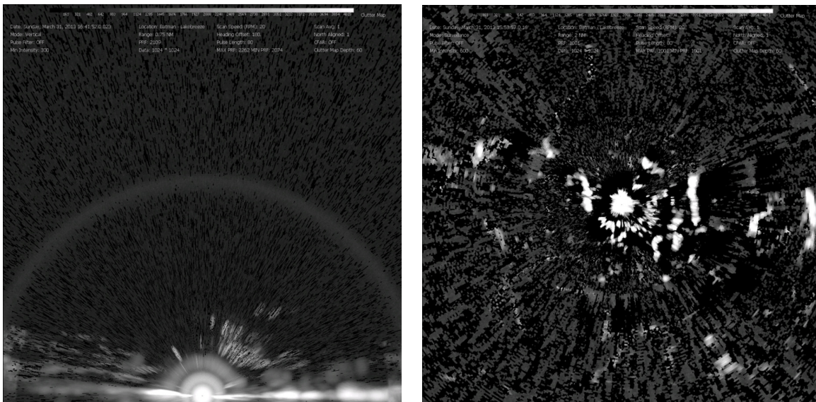
Figure 4. Vertical (left) and horizontal (right) clutter maps from Niagara (top) and Wayne (bottom) counties, New York. Examples of side lobes are the rings of white on the vertical radar; some are partial rings while others connect fully. The side lobes can vary in intensity (how bright they are) as well as how thick the band is.
