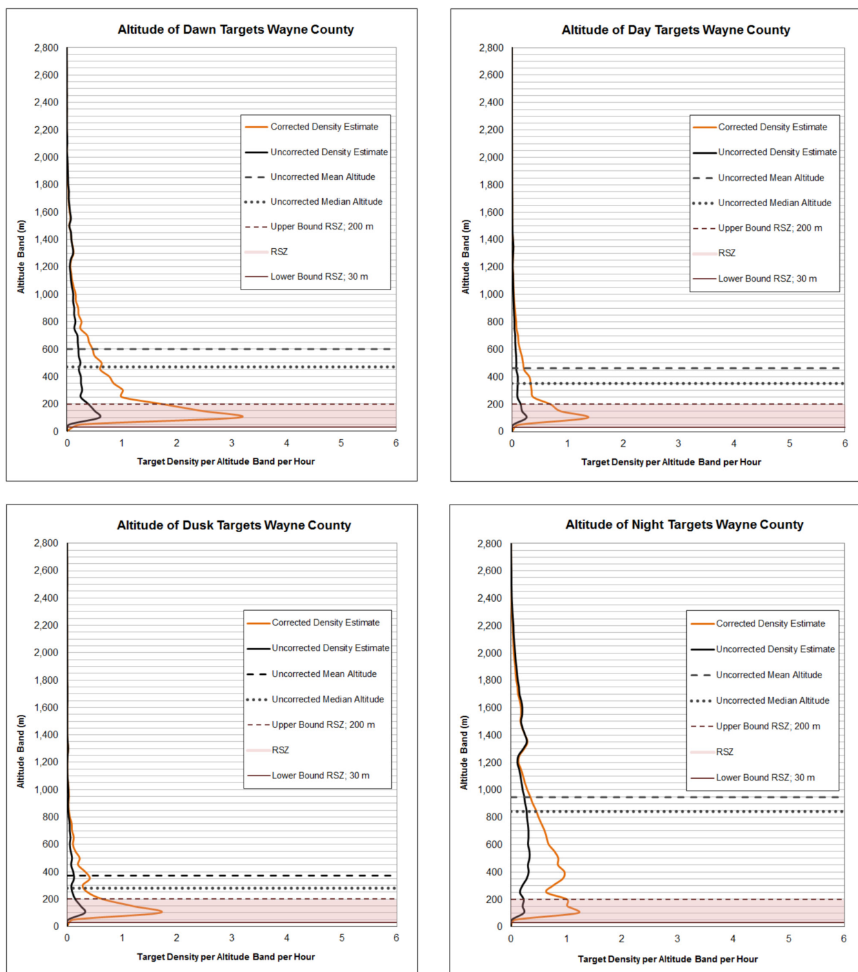
Figure 25. Altitude profiles of targets in Wayne County, New York. The corrected lines (orange) depict the target density (targets/1,000,000 m 3 ) per 50-m altitude band per hour after adjusting for the structure of the sample volume. The uncorrected lines (black) depict the target density per 50-m altitude band per hour assuming a uniform volume distribution (i.e., the volume of each band is equal to the total volume divided by the number of bands). The red band represents the rotor-swept zone (RSZ) from 30 to 200 m. The x-axis represents the target density (targets/1,000,000 m 3 ) per 50-m altitude band. The y-axis labels represent the top of each attitude band in meters.
