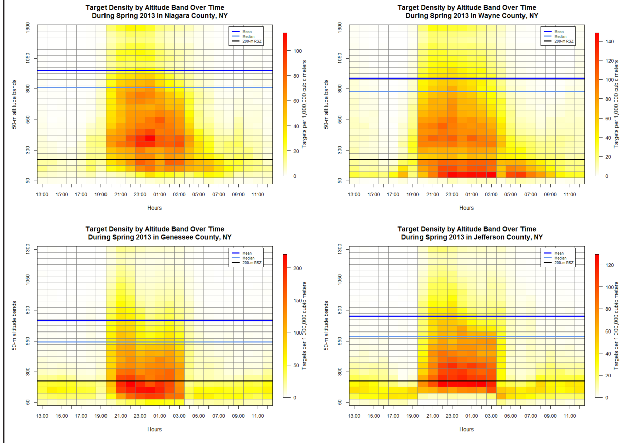
Figure 35. These graphs present the density of targets that occurred within each 50-m altitude band in Niagara, Wayne, Genesee, and Jefferson counties, New York, in spring 2013 over each of the 24 hours in a day. Please note the different scales for each of the heat maps. Deep red areas on one graph may be equivalent in density to yellow areas on another heat map. This is at least partially due to differences in detection ability due to clutter and target movement direction which make comparisons between sites difficult. Dark blue lines represent the mean altitude and light blue lines represent the median altitude across all hours. The black lines represent the top of the 200-m rotor-swept zone. The graphs only extend up to 1300 m and not to the full height of the radar scan to better show detail of the lower altitude bands.
