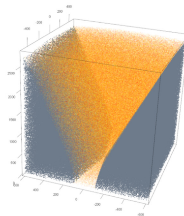
Figure 7. Graphical representation of the structural volume of the vertical scanning radar within the standard front. In this graphic, the radar unit is located at the origin, and the radar beam extends to 500 m on either side of the radar unit (x-axis) and up to a maximum height of 2,800 m (z-axis). The y-axis represents the spread of the radar beam as it extends away from the origin. The orange semi-transparent points represent the volume contained by the structure of the radar beam. The dark gray points represent the volume that is within the box but is not included in the volume of the radar beam.
