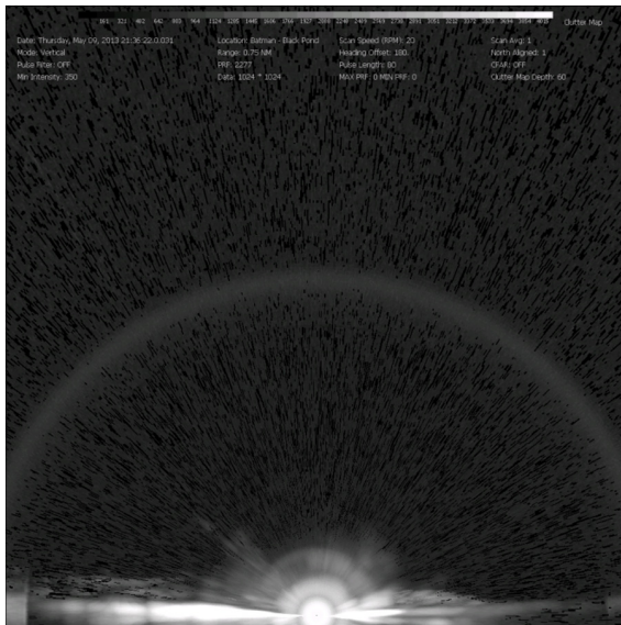
Figure 5. Vertical (left) and horizontal (right) clutter maps from Genesee (top) and Jefferson (bottom) counties, New York. Examples of side lobes are the rings of white on the vertical radar, some are partial rings while others connect fully. The side lobes can vary in intensity (how bright they are) as well as how thick the band is.
