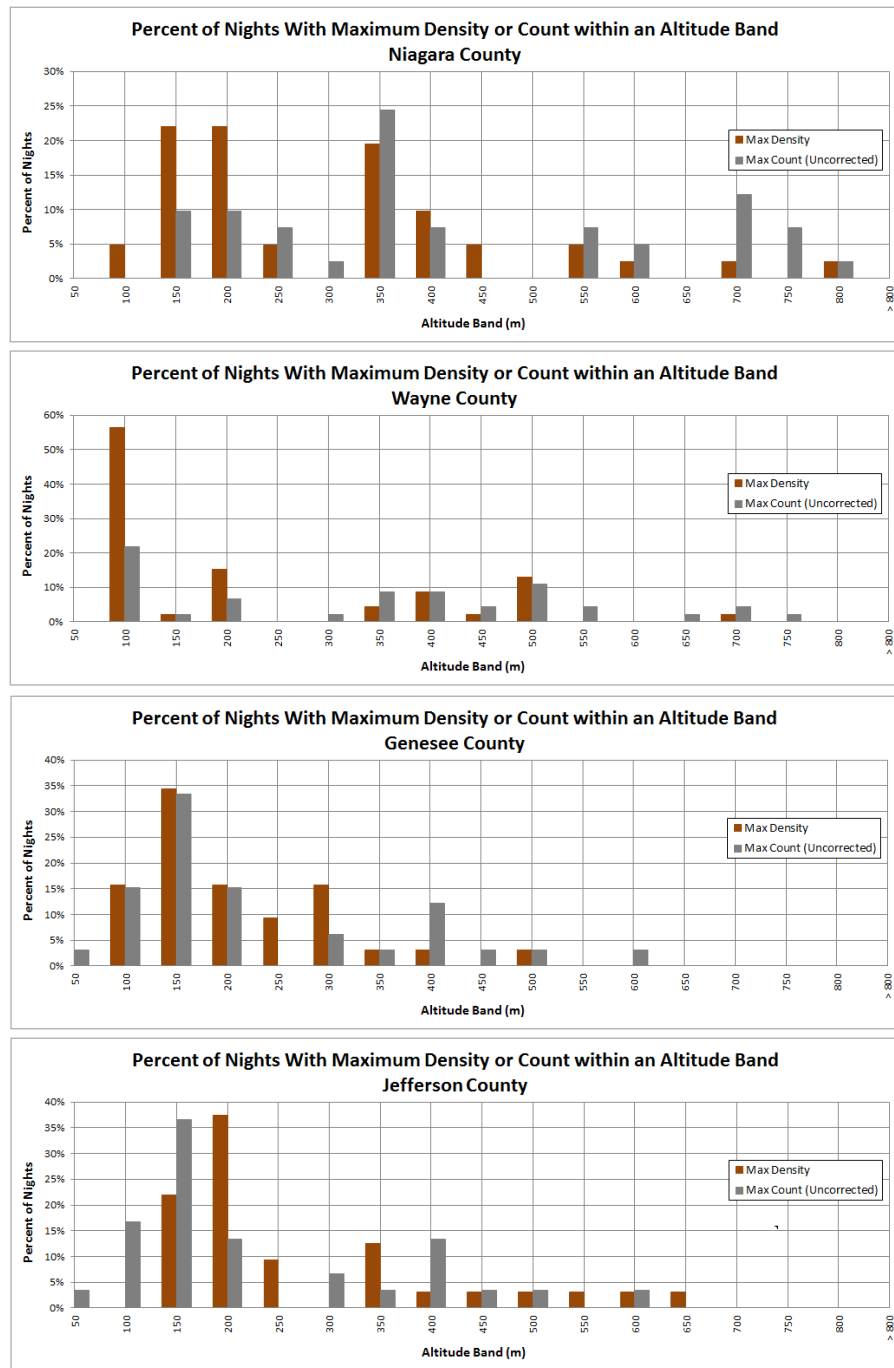
Figure 33. These graphs present the proportion of nights when the maximum density (targets/1,000,000 m 3 /altitude band) or count (targets/altitude band) occurred within each 50-m altitude band in Niagara, Wayne, Genesee, and Jefferson counties, New York, in spring 2013. The x-axis labels represent the top of each altitude band.
