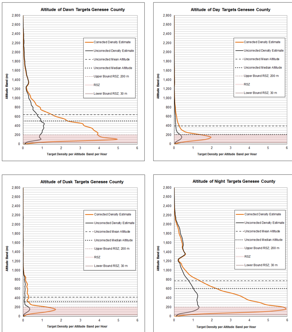
Figure 26. Altitude profiles of targets in Genesee County, New York. The corrected lines (orange) depict the target density (targets/1,000,000 m 3 ) per 50-m altitude band per hour after adjusting for the structure of the sample volume. The uncorrected lines (black) depict the target density per 50-m altitude band per hour assuming a uniform volume distribution (i.e., the volume of each band is equal to the total volume divided by the number of bands). The red band represents the rotor-swept zone (RSZ) from 30 to 200 m. The x-axis represents the target density (targets/1,000,000 m 3 ) per 50-m altitude band. The y-axis labels represent the top of each altitude band in meters.
