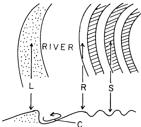
Figure 5. A meander bend and cross section showing levee (L) and ridge (R) and swale (S) topography so common on modern and relict surfaces. Pioneer and successional plant species anchor the newly formed sandy ridges leading to even more deposition at each high water episode. Normal helicoidal currents (C) conduct sediments up the bar slope.
