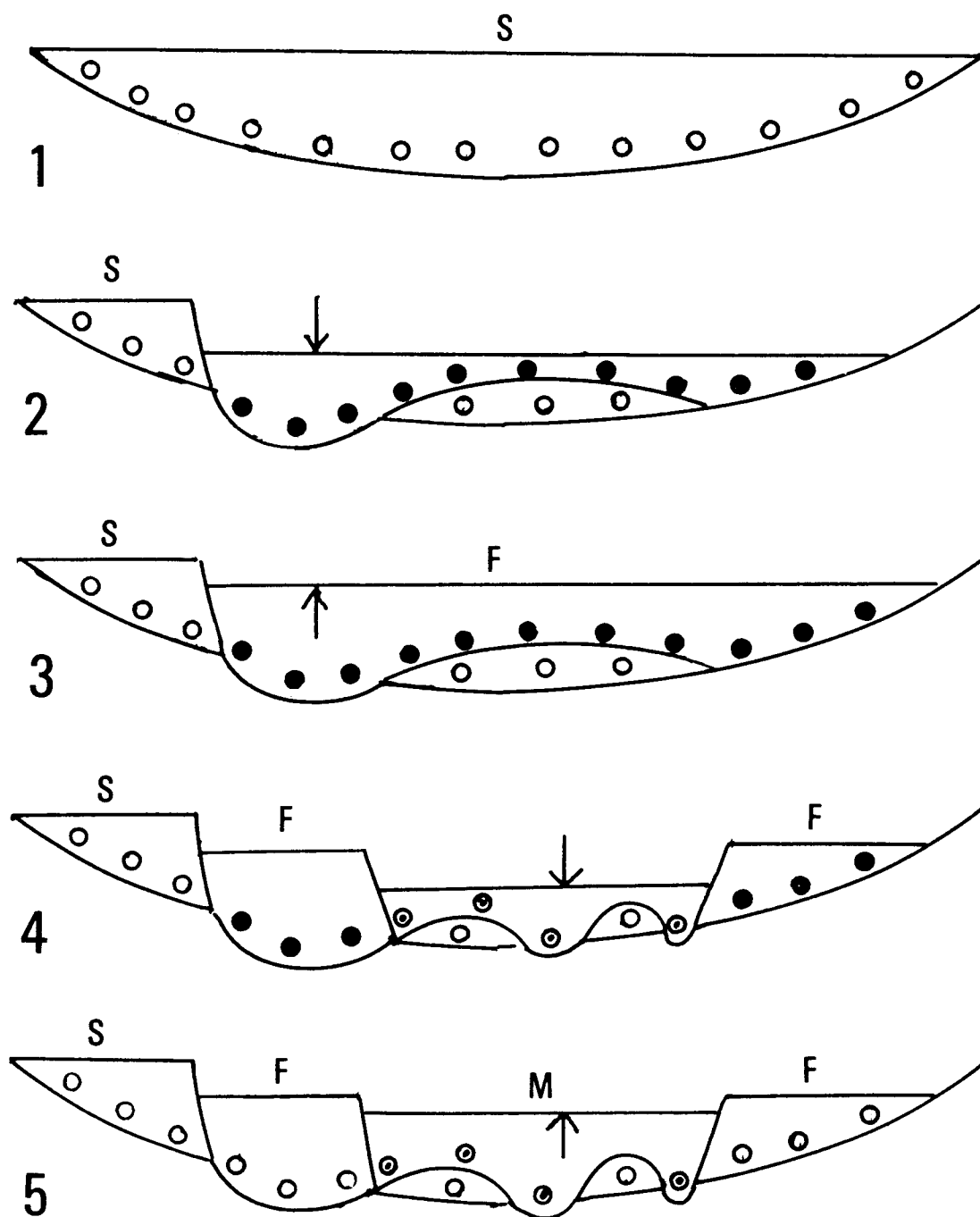
Figure 8. Development of present-day relict and modern floodplain surfaces. (1) Sangamon (S) interglacial stage. (2) Entrenchment (scouring) during waxing Altonian substage. (3) Farmlandian (F) interglacial with substage alluviation filling in the former entrenched valley. (4) Entrenchment during waxing Woodfordian substage. Remaining Farmlandian (F) deposits are also known as Deweyville (or Terrace I). (5) Post-Woodfordian alluviation forming modern day Holocene floodplain surface (M) about 4-5,000 years ago. Drawings highly modified from Saucier and Fleetwood (1970).
