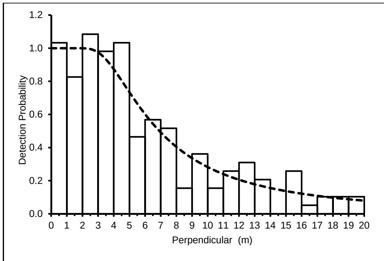
Figure 13. Observed detections (histogram) and the resulting detection function (smooth curve) for live tortoises with MCL \geq 180\text{mm} found by GBI. This curve uses only the 166 observations found within 20 m of the line.
