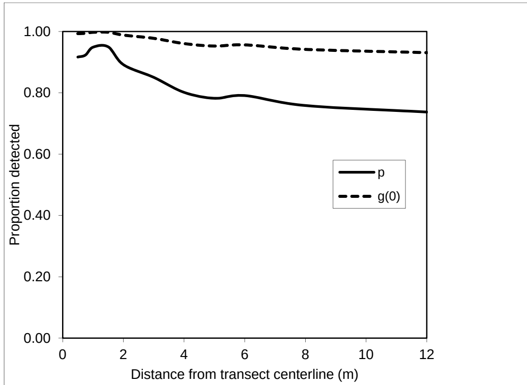
Figure 16. Detection pattern for the leader ( p ) and by the team ( g(0) ) based on all observations out to a given distance ( x ) from the centerline in 2011. Note convergence of g(0) on 1.0 as x goes to 0.
