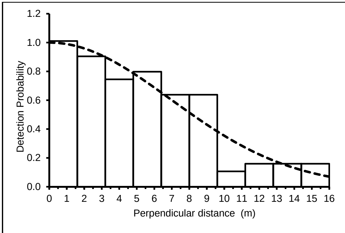
Figure 15. Observed detections (histogram) and the resulting detection function (smooth curve) for live tortoises with MCL \geq 180 mm found by Kiva. This curve uses only the 100 observations found within 16 m of the line.
