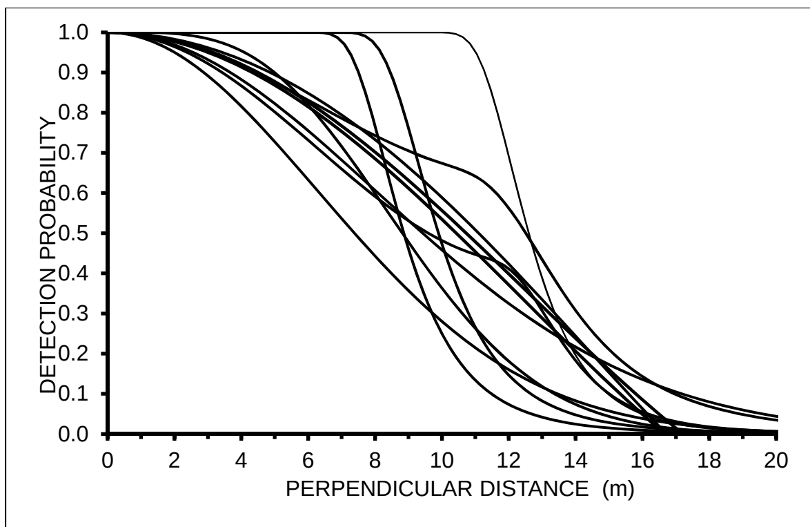
Figure 6. Detection curves for each of the 2011 GBI teams during training. Curves are based on 16 km trials with approximately 100 detections.
