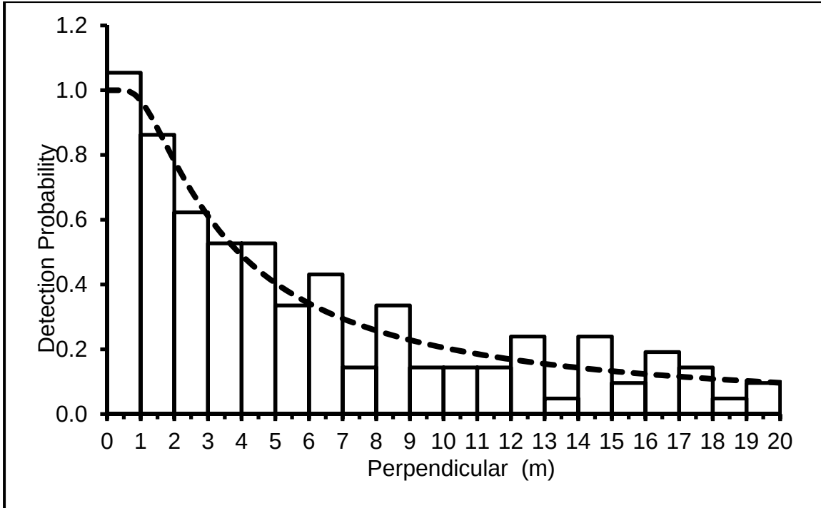
Figure 14. Observed detections (histogram) and the resulting detection function (smooth curve) for live tortoises with MCL \geq 180 mm found by IWS. This curve uses only the 133 observations found within 20 m of the line.
