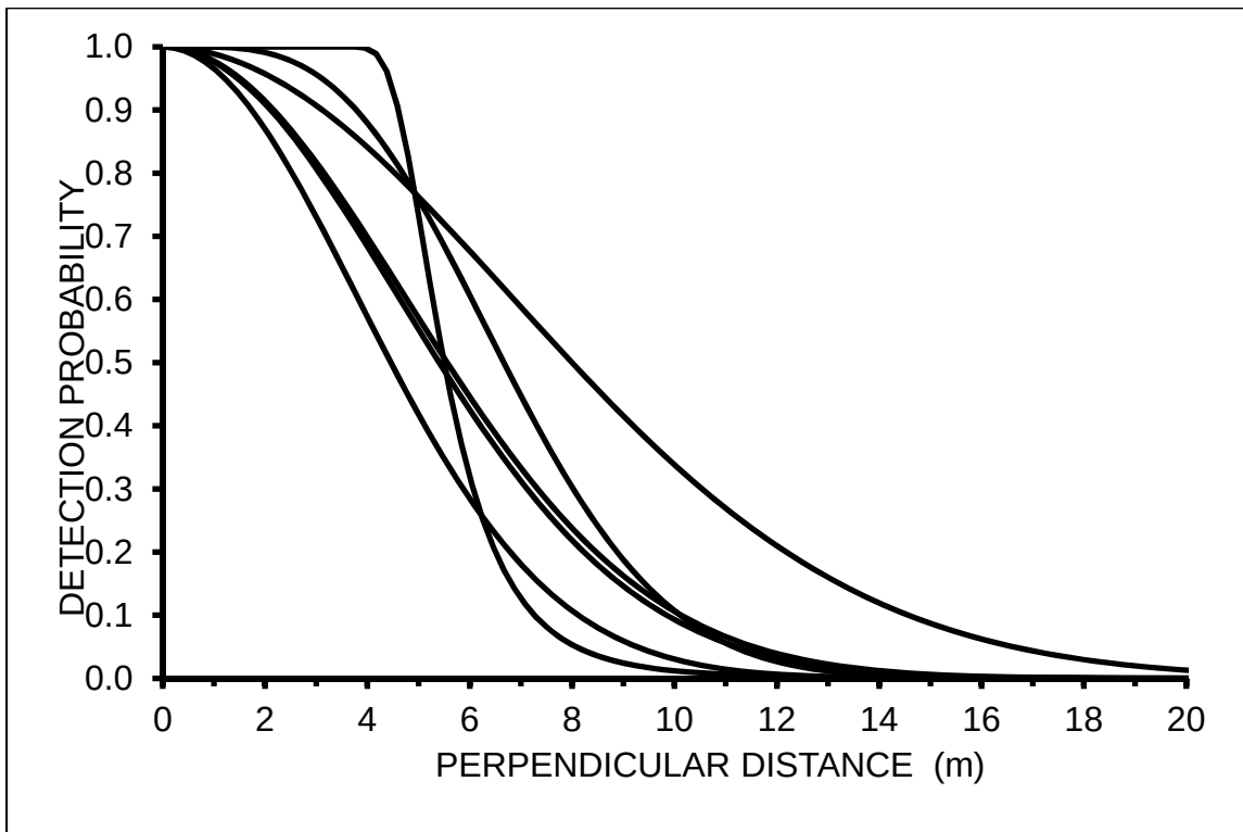
Figure 8. Detection curves for each of the 2011 Kiva trainee teams. Curves are based on 16 km trials with approximately 100 detections.
