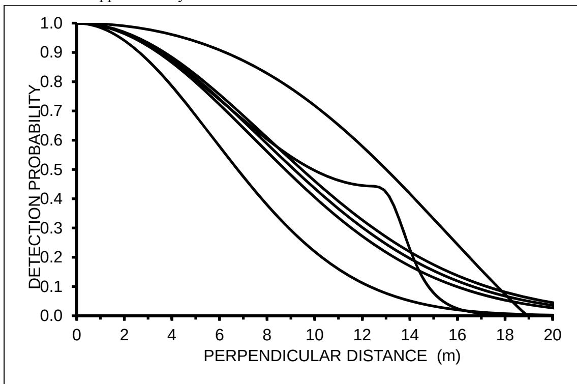
Figure 7. Detection curves for each of the 2011 IWS trainee teams. Curves are based on 16 km trials with approximately 100 detections.
