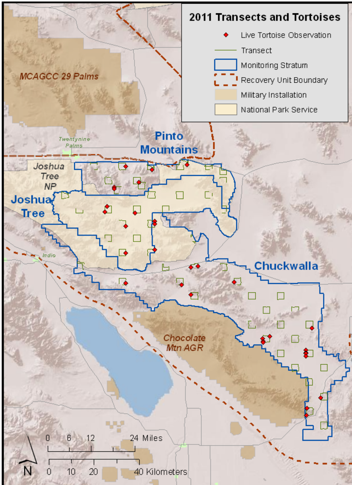
Figure 12. Distribution of distance sampling transects and live tortoise observations in the western portion of the Colorado Desert Recovery Unit (Pinto Mountains, Joshua Tree, and Chuckwalla monitoring strata). Chocolate Mountain AGR was not surveyed in 2011.
