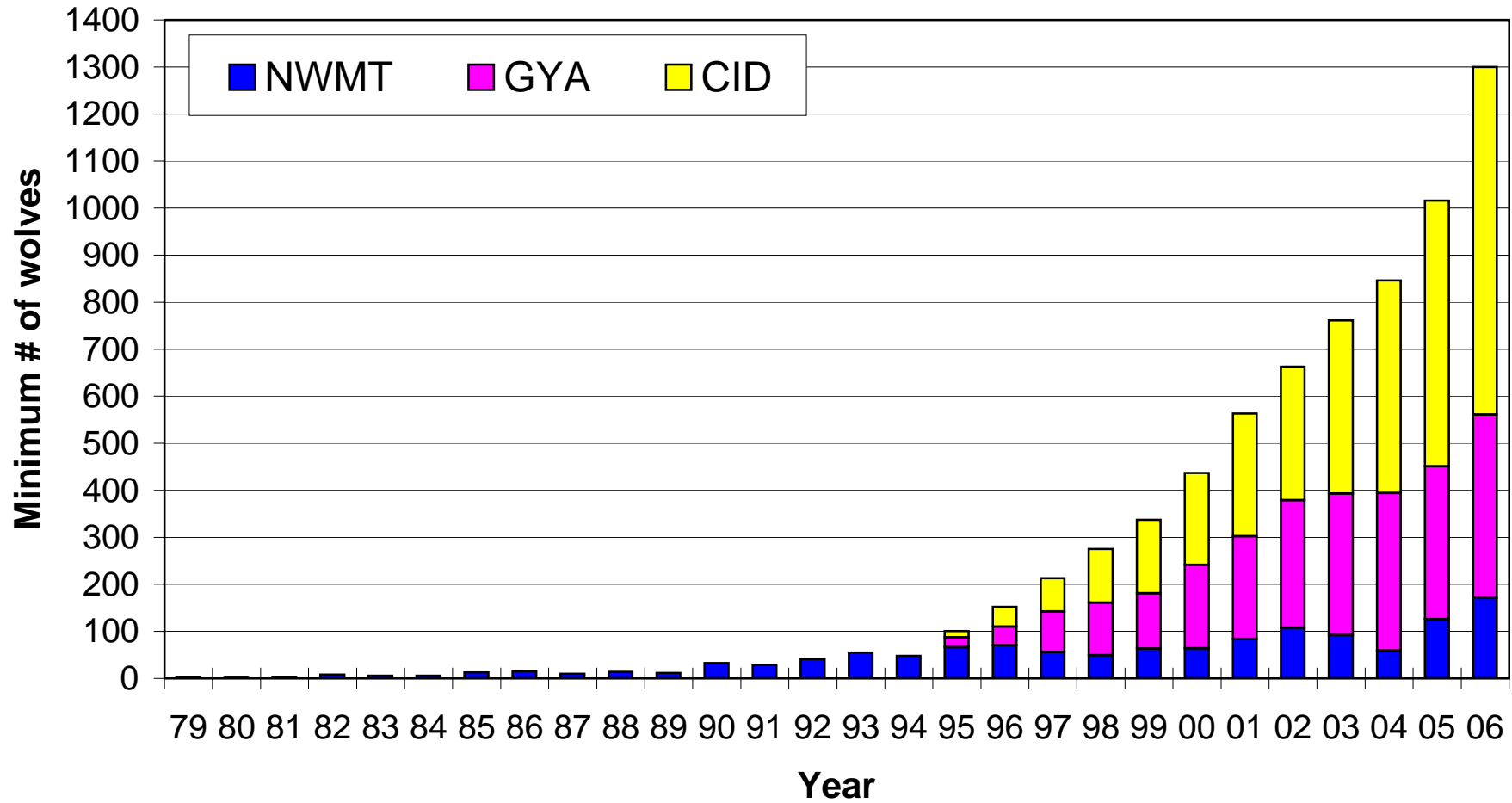
Figure 5. Northern Rocky Mountain Wolf Population Trends, by Recovery Area 1979-2006
