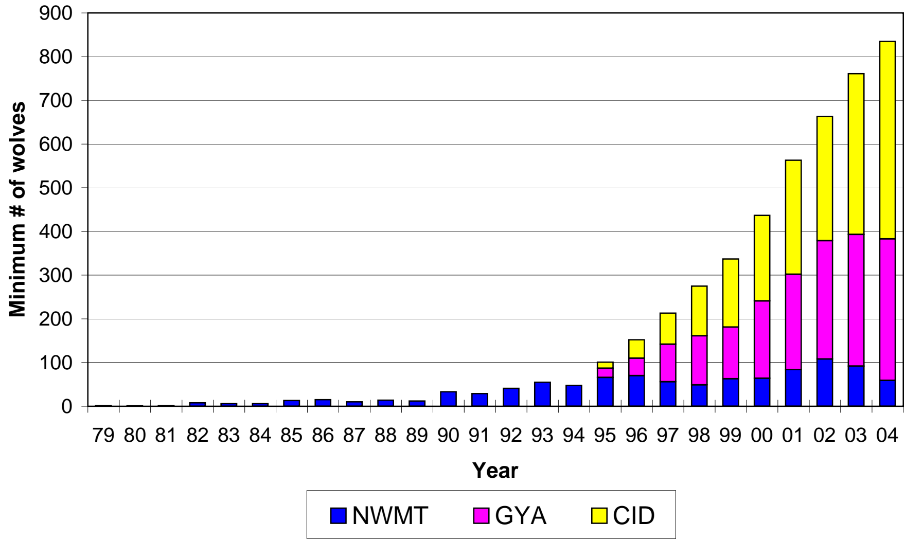
Figure 5. Northern Rocky Mountain Wolf Population Trends 1979-2004, by Recovery Area
