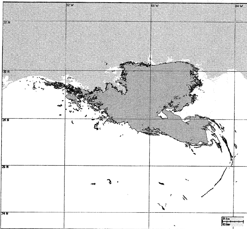
Figure 1. Cumulative potential surface floating oil extent of the DWHOS. (Figure derived from compositing April, May, June, and July 2010 radar shape files available on the NOAA ERMA website. Note that radar images with noted anomalies were not included in composite.) Summary of Historical Shelf and Offshore Plankton Data
