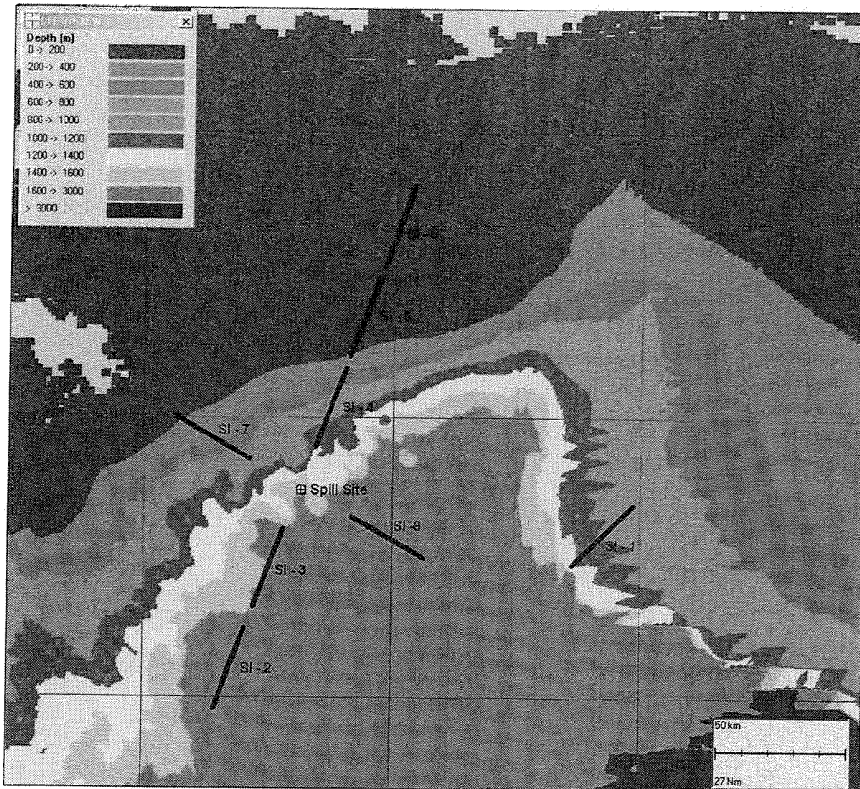
Figure 2. Sipper transects shown as black lines over bathymetry. Transects are 18 NM each.
