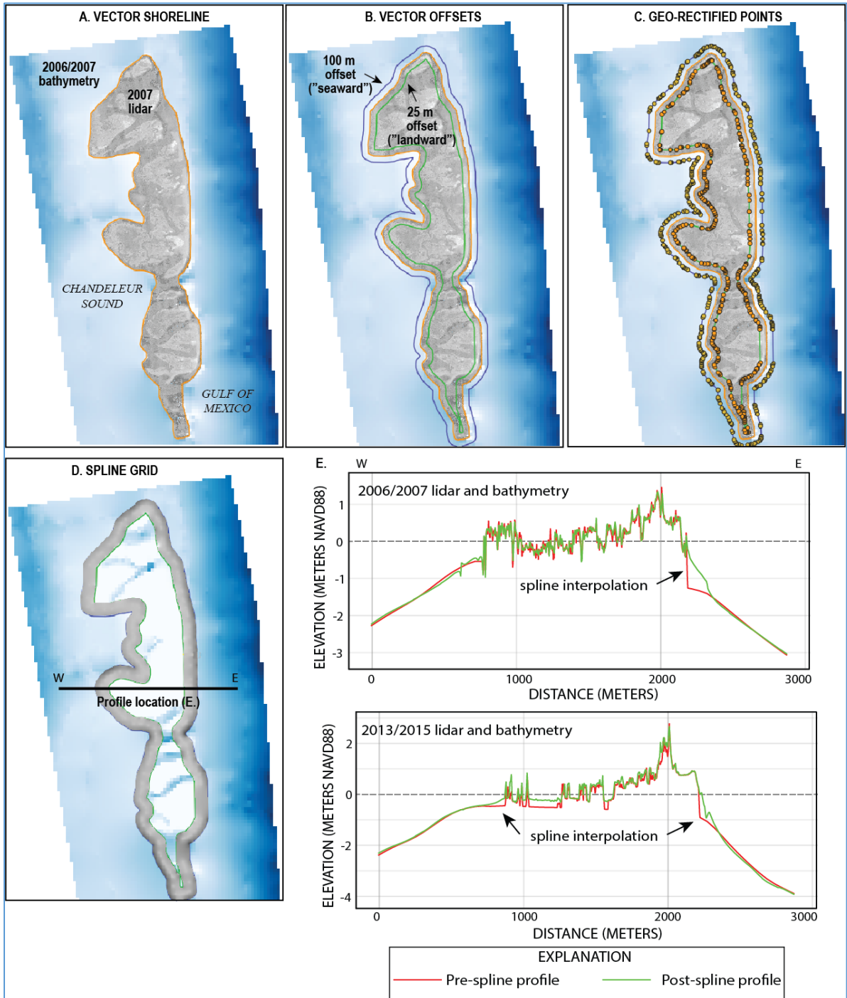
Figure 9. Visualization showing the processing steps utilized to add interpolated points across the topographic to bathymetric transition using a spline method, which resulted in a more natural representation of the transition in the resulting DEM (Flocks et al. IN PRESS).
