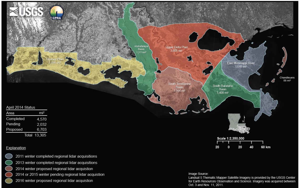
Figure 7. USGS NGP recent southern Louisiana topographic LiDAR data acquisitions.
