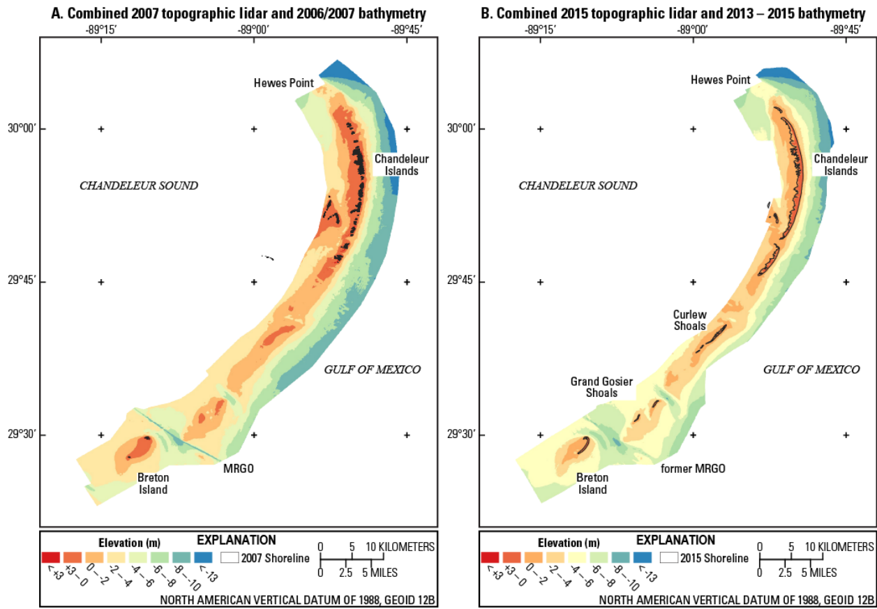
Figure 8. Topobathymetric DEM for the 2006 – 2007 (A) and 2013 – 2015 (B) time periods created by combining the topographic (LiDAR), bathymetric, and spline interpolated data points (Flocks et al. IN PRESS).
