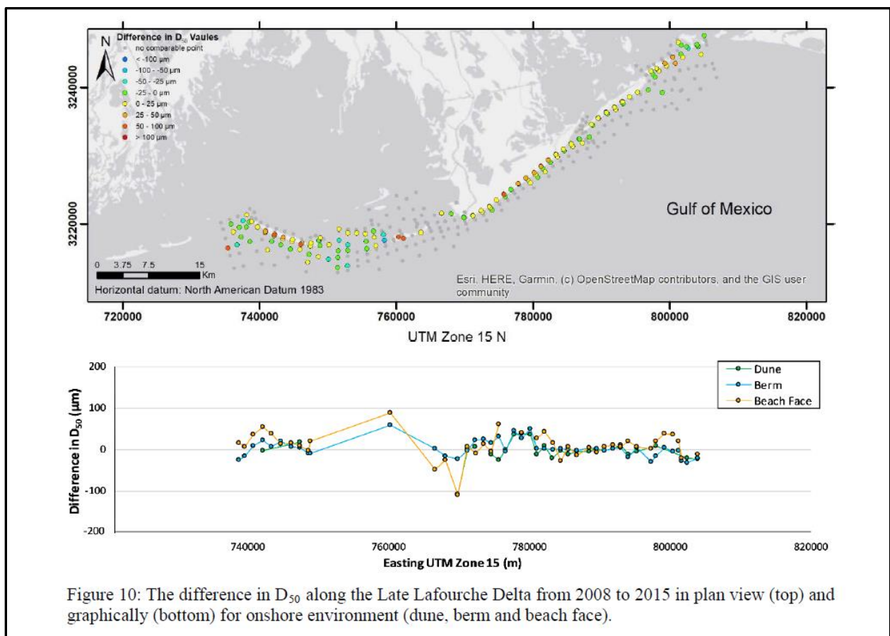
Figure 10. Grain size changes along the Late Lafourche Delta region with specific changes in the Dune, Berm, and Beach face (Georgiou et al. 2019).
