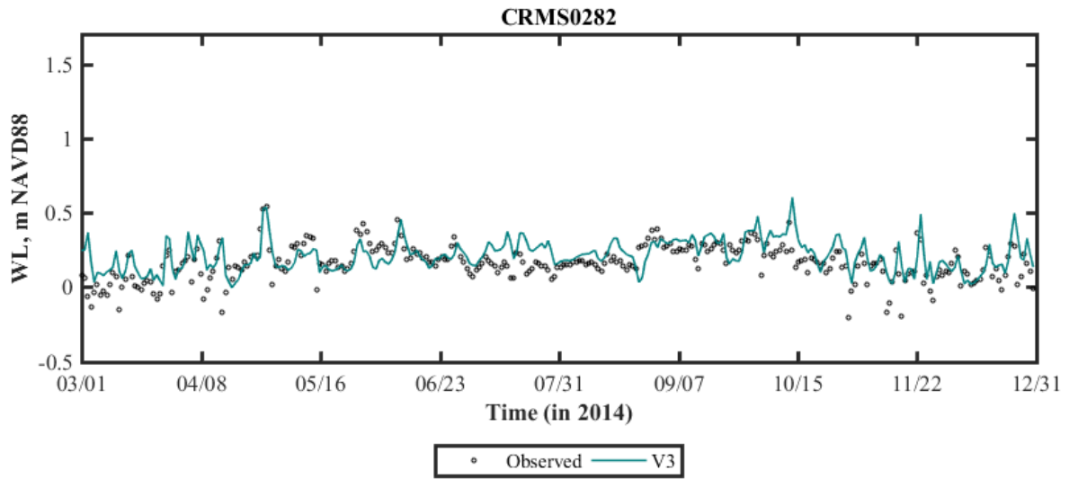
Figure B 3.V3 Basinwide model calibration of daily water level (WL) at CRMS0282 (Grand Bayou community), in Barataria Basin (2014).
