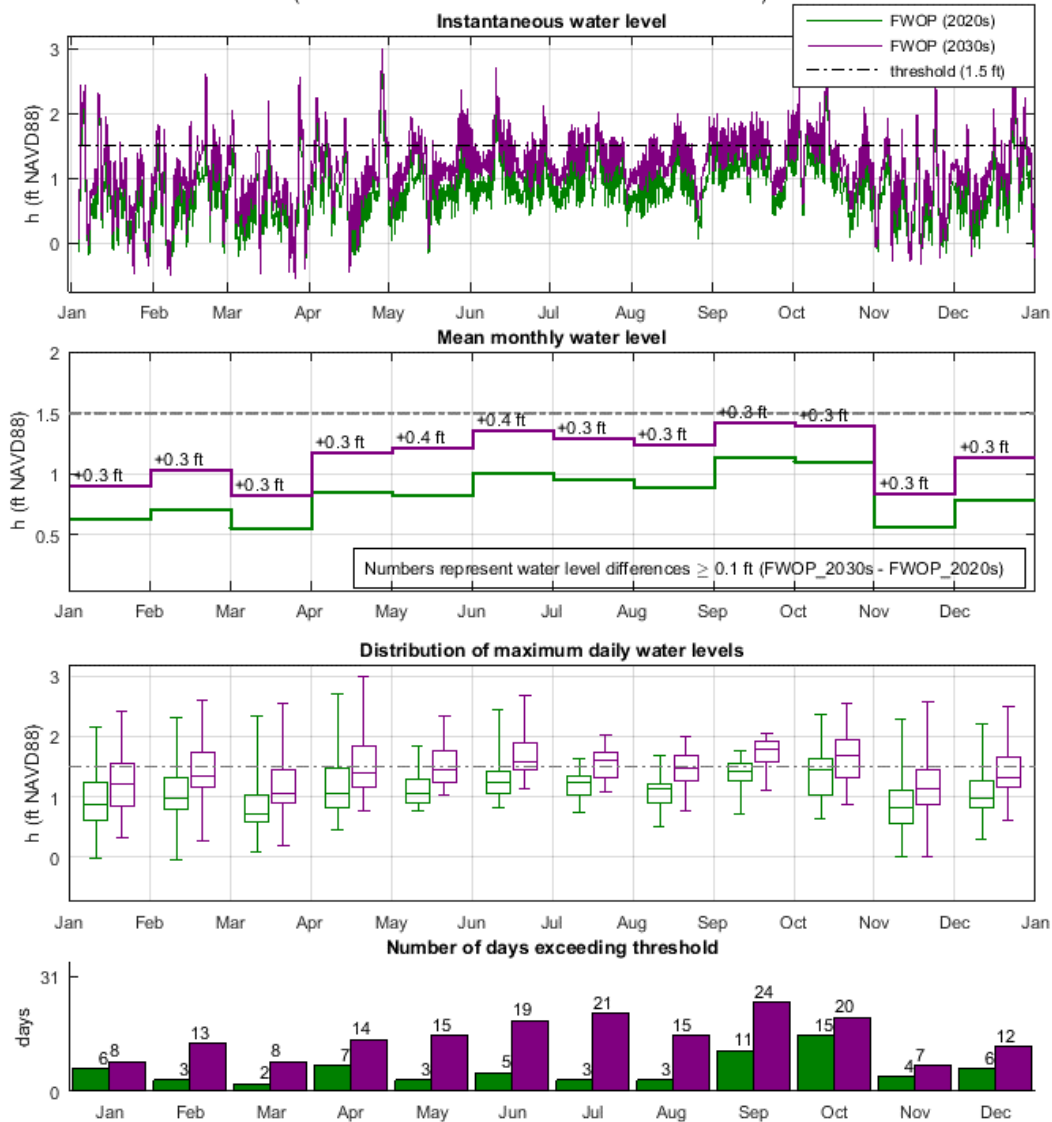
Figure 15: WSE analysis for Grand Bayou, FWOP for the first decade (2020s, in green) and the second decade (2030s, in purple), using the hydrograph of year 2011. The top-most plot shows instantaneous water level (h). The second-from-the-top plot shows mean monthly water level (h). The third-from-the-top plot shows the distribution of maximum daily water levels (h) in box and whiskers plot format. The bottom plot shows the number of days exceeding the WSE threshold used for this community. Water level is referenced to NAVD88 (GEOID12A).
