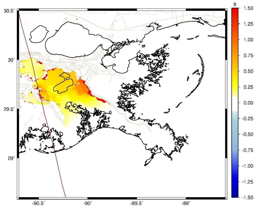
Figure 4-4. Peak water level difference for 2040 Applicant’s Preferred Alternative Completely Open less 2040 Applicant’s Preferred Alternative during 4 percent AEP event (Storm 011) in June water level conditions.
