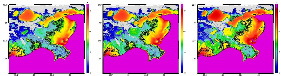
Figure 3-13. No Action Alternative maximum wave height for storm 101, 4 percent AEP storm, year 2020 (left), year 2040 (middle), year 2070 (right).
