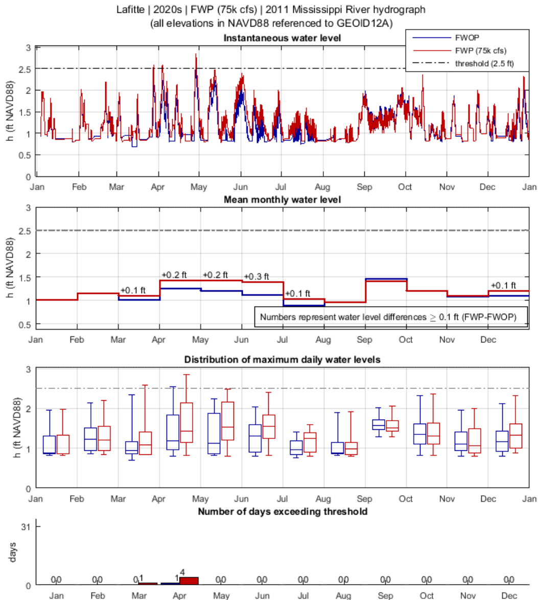
Figure 18: Analysis of diversion impact on WSEs in Lafitte during the 2020s, FWOP and FWP (75k cfs), using the river hydrograph of year 2011. The top-most plot shows instantaneous water level (h). The second-from-the-top plot shows mean monthly water level (h). The third-from-the-top plot shows the distribution of maximum daily water levels (h) in box and whiskers plot format. The bottom plot shows the number of days exceeding the WSE threshold used for this community. Water level is referenced to NAVD88 (GEOID12A).
