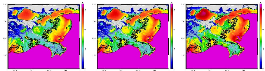
Figure 3-19. No Action Alternative maximum wave height for storm 245, 1 percent AEP storm, year 2020 (left), year 2040 (middle), year 2070 (right).
