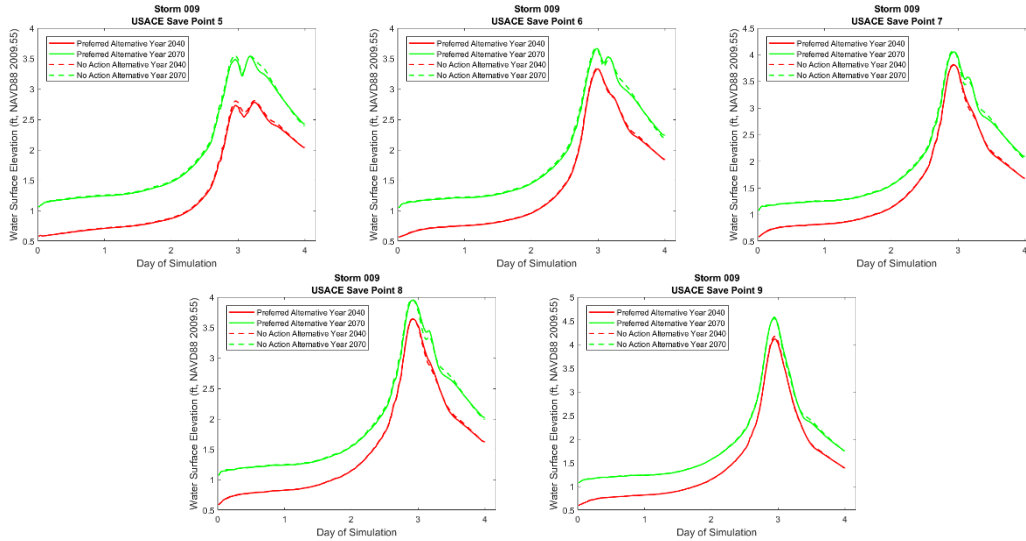
Figure 3-65. Hydrographs at selected save points near the LGM for storm 009, 1 percent AEP storm, showing water surface elevation for the No Action Alternative (red hashed 2040, green hashed 2070) and Applicant’s Preferred Alternative (red solid 2040, green solid 2070).
