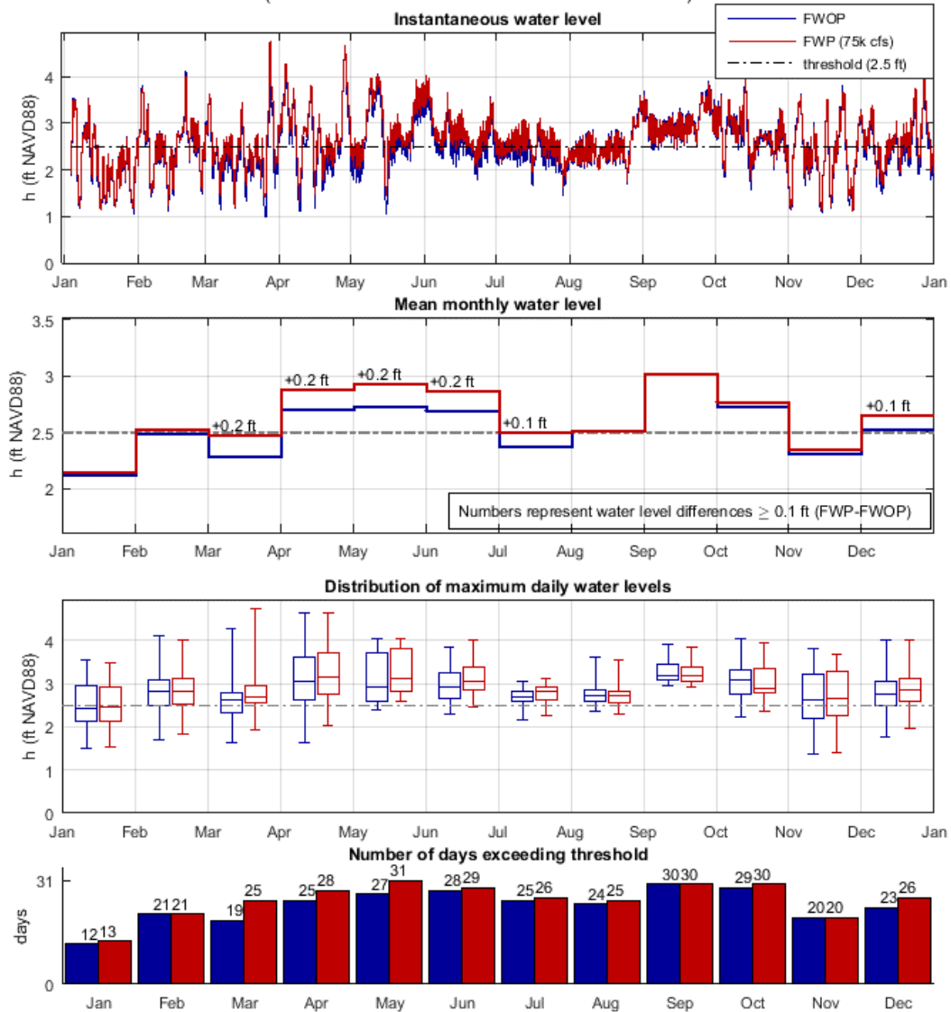
Figure 24. Analysis of diversion impact on WSEs in Lafitte during the 2060s, FWOP and FWP (75k cfs), using the river hydrograph of year 2011. The top-most plot shows instantaneous water level (h). The second-from-the-top plot shows mean monthly water level (h). The third-from-the-top plot shows the distribution of maximum daily water levels (h) in box and whiskers plot format. The bottom plot shows the number of days exceeding the WSE threshold used for this community. Water level is referenced to NAVD88 (GEOID12A).
