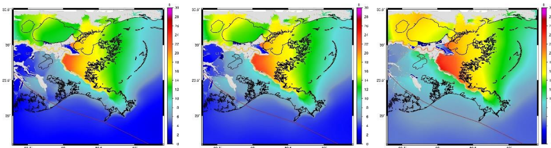
Figure 3-22. No Action Alternative maximum water surface elevation for storm Isaac, year 2020 (left), year 2040 (middle), year 2070 (right).
