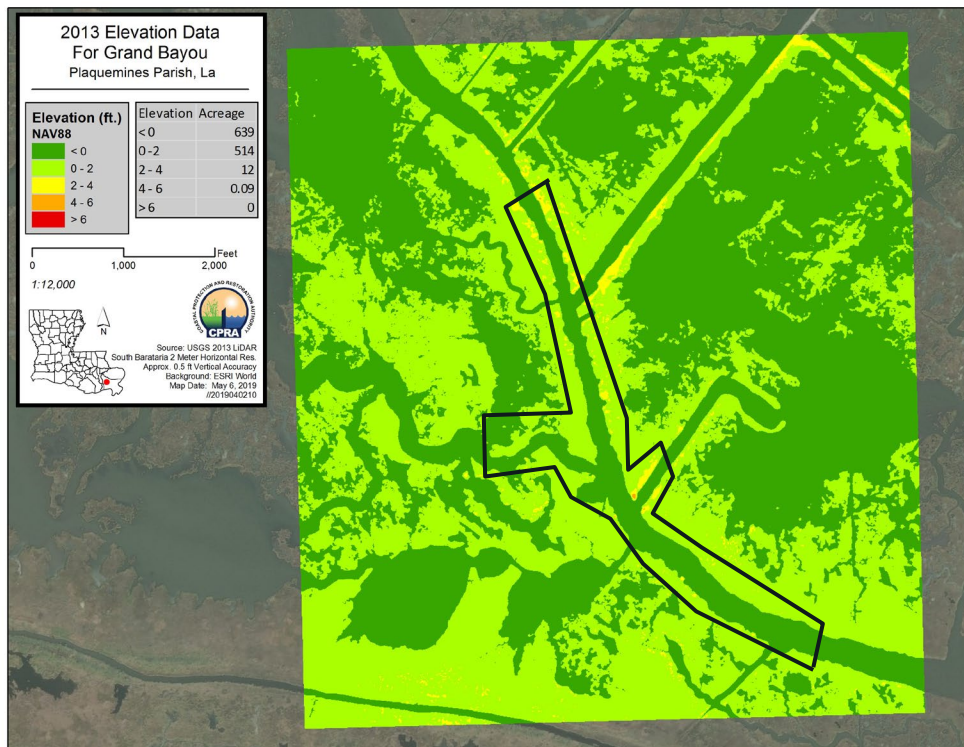
Figure A 4. USGS 2013 LiDAR (DEM) showing ground elevations at Grand Bayou and area (in black) where communities are located. The ground elevations within the populated area are largely in the range +0-2 ft NAVD88.
