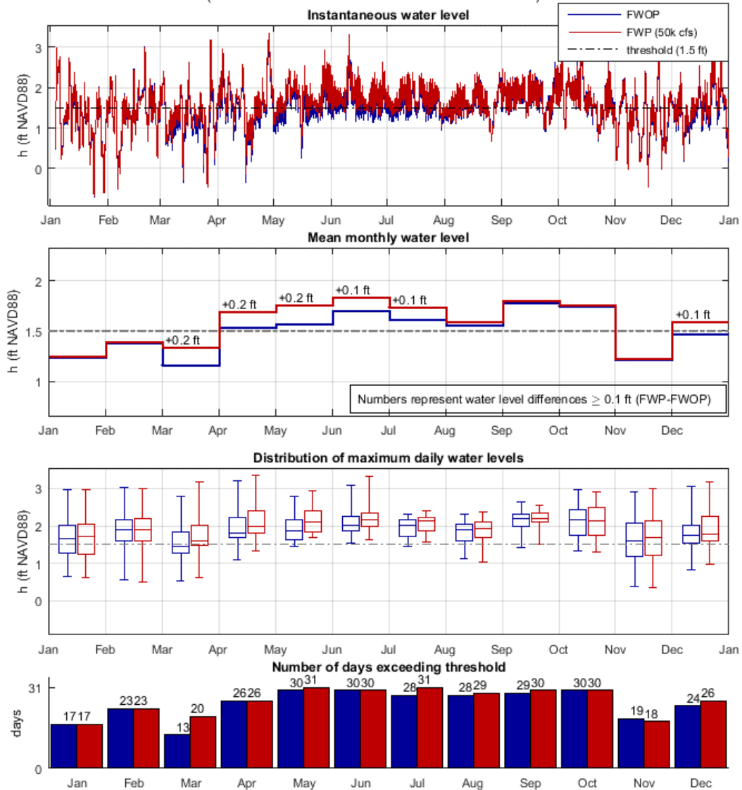
Figure C 6: Analysis of diversion impact on WSEs at Grand Bayou during the 2040s, FWOP and FWP (50k cfs), using the river hydrograph of year 2011. The top-most plot shows instantaneous water level (h). The second-from-the-top plot shows mean monthly water level (h). The third-from-the-top plot shows the distribution of maximum daily water levels (h) in box and whiskers plot format. The bottom plot shows the number of days exceeding the WSE threshold used for this community. Water level is referenced to NAVD88 (GEOID12A).
