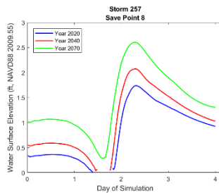
Figure 3-37. No Action Alternative Hydrographs at a save point near Lafitte for storm 257, 4 percent AEP storm, showing water surface elevation for year 2020 (blue), year 2040 (red), year 2070 (green).
