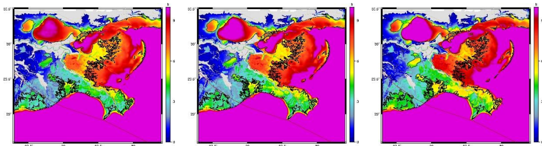
Figure 3-23. No Action Alternative maximum wave height for storm Isaac, year 2020 (left), year 2040 (middle), year 2070 (right).
