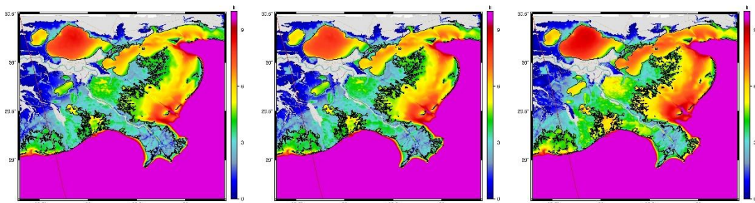
Figure 3-5. No Action Alternative maximum wave height for storm 011, 4 percent AEP storm, year 2020 (left), year 2040 (middle), year 2070 (right).
