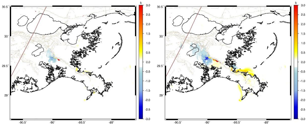
Figure 3-53. Maximum wave height difference between the Applicant's Preferred Alternative and the No Action Alternative for storm 160, 1 percent AEP storm, year 2040 (left), year 2070 (right).
