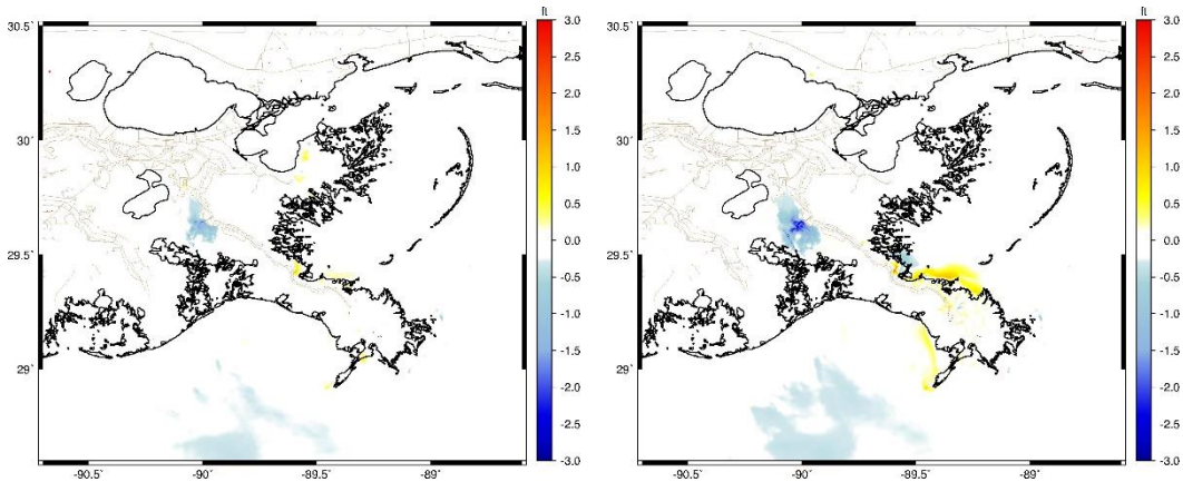
Figure 3-55. Maximum wave height difference between the Applicant's Preferred Alternative and the No Action Alternative for storm 239, 4 percent AEP storm, year 2040 (left), year 2070 (right).
