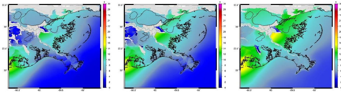
Figure 3-12. No Action Alternative maximum water surface elevation for storm 101, 4 percent AEP storm, year 2020 (left), year 2040 (middle), year 2070 (right).
