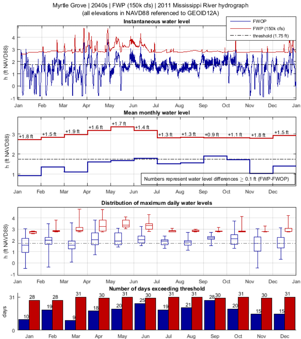
Figure C 14: Analysis of diversion impact on WSEs in Myrtle Grove during the 2040s, FWOP and FWP (150k cfs), using the river hydrograph of year 2011. The top-most plot shows instantaneous water level (h). The second-from-the-top plot shows mean monthly water level (h). The third-from-the-top plot shows the distribution of maximum daily water levels (h) in box and whiskers plot format. The bottom plot shows the number of days exceeding the WSE threshold used for this community. Water level is referenced to NAVD88 (GEOID12A).
