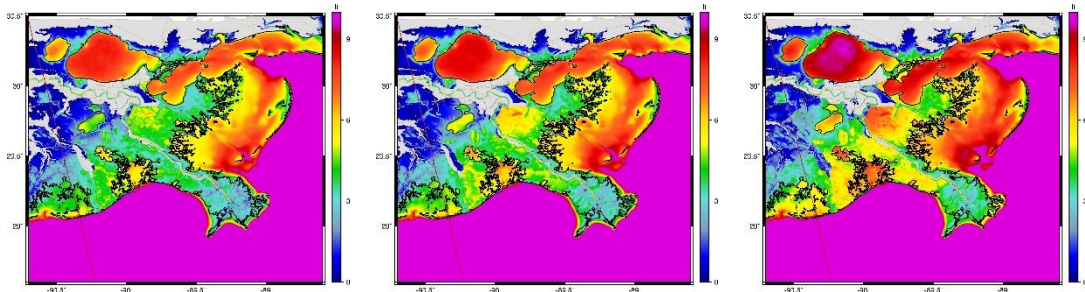
Figure 3-9. No Action Alternative maximum wave height for storm 014, 1 percent AEP storm, year 2020 (left), year 2040 (middle), year 2070 (right).
