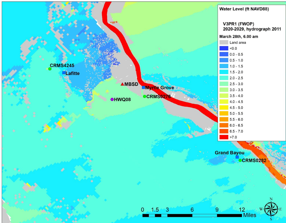
Figure 28: Instantaneous WSE (water level) for FWOP (V3PR1) during a wind driven peak event (Peak 1) during the 2020s.
