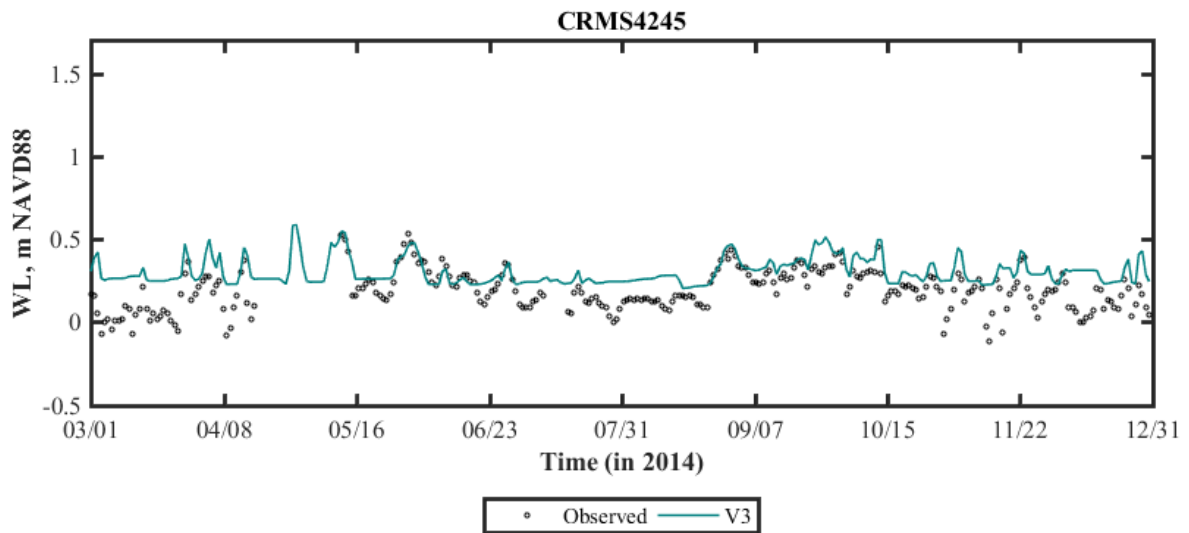
Figure B 2.V3 Basinwide model calibration of daily water level (WL) at CRMS4245 (Lafitte community), in Barataria Basin (2014).
