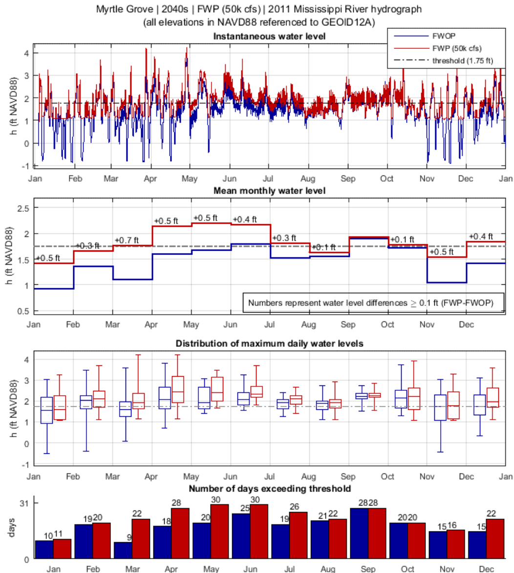
Figure C 4: Analysis of diversion impact on WSEs in Myrtle Grove during the 2040s, FWOP and FWP (50k cfs), using the river hydrograph of year 2011. The top-most plot shows instantaneous water level (h). The second-from-the-top plot shows mean monthly water level (h). The third-from-the-top plot shows the distribution of maximum daily water levels (h) in box and whiskers plot format. The bottom plot shows the number of days exceeding the WSE threshold used for this community. Water level is referenced to NAVD88 (GEOID12A).
