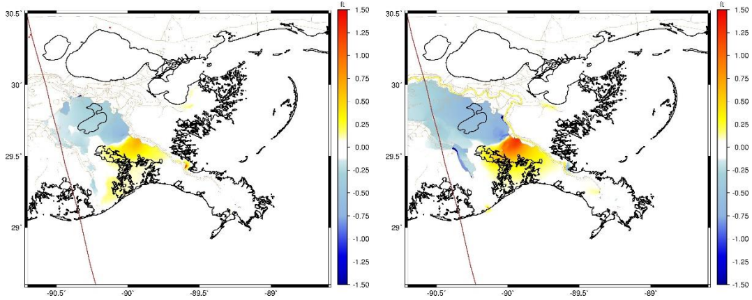
Figure 3-44. Maximum water surface elevation difference between the Applicant's Preferred Alternative and the No Action Alternative storm 011 slow, 4 percent AEP storm, year 2040 (left), year 2070 (right).
