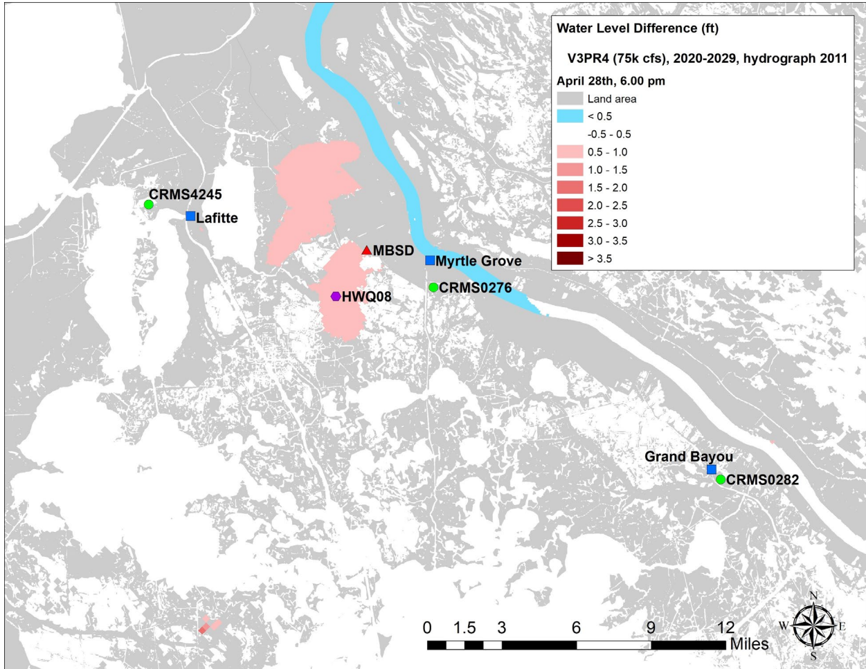
Figure 31: Difference in instantaneous WSEs for FWOP (V3PR1) and FWP (V3PR4, 75k cfs) during a wind driven peak event during the 2020s, 2011 hydrograph on April 28 th , 2011 at 6 pm.
