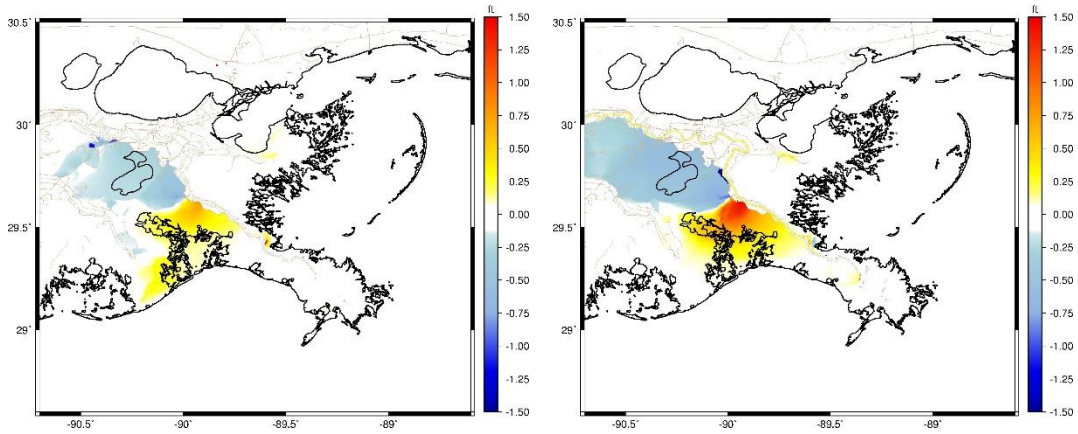
Figure 3-40. Maximum water surface elevation difference between the Applicant’s Preferred Alternative and the No Action Alternative for storm 009, 1 percent AEP storm, year 2040 (left), year 2070 (right).
