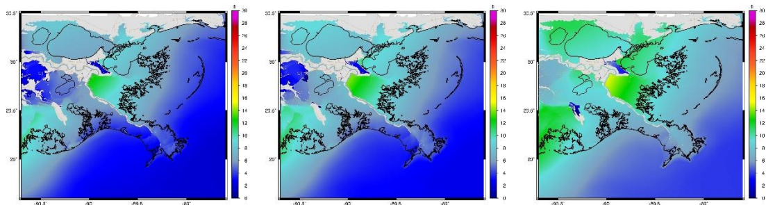
Figure 3-16. No Action Alternative maximum water surface elevation for storm 239, 4 percent AEP storm, year 2020 (left), year 2040 (middle), year 2070 (right).
