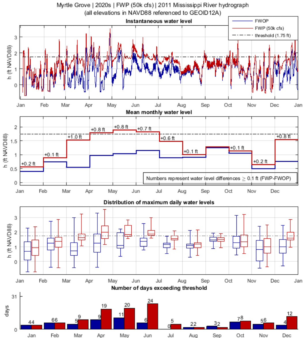
Figure C 1: Analysis of diversion impact on WSEs in Myrtle Grove during the 2020s, FWOP and FWP (50k cfs), using the river hydrograph of year 2011. The top-most plot shows instantaneous water level (h). The second-from-the-top plot shows mean monthly water level (h). The third-from-the-top plot shows the distribution of maximum daily water levels (h) in box and whiskers plot format. The bottom plot shows the number of days exceeding the WSE threshold used for this community. Water level is referenced to NAVD88 (GEOID12A).
