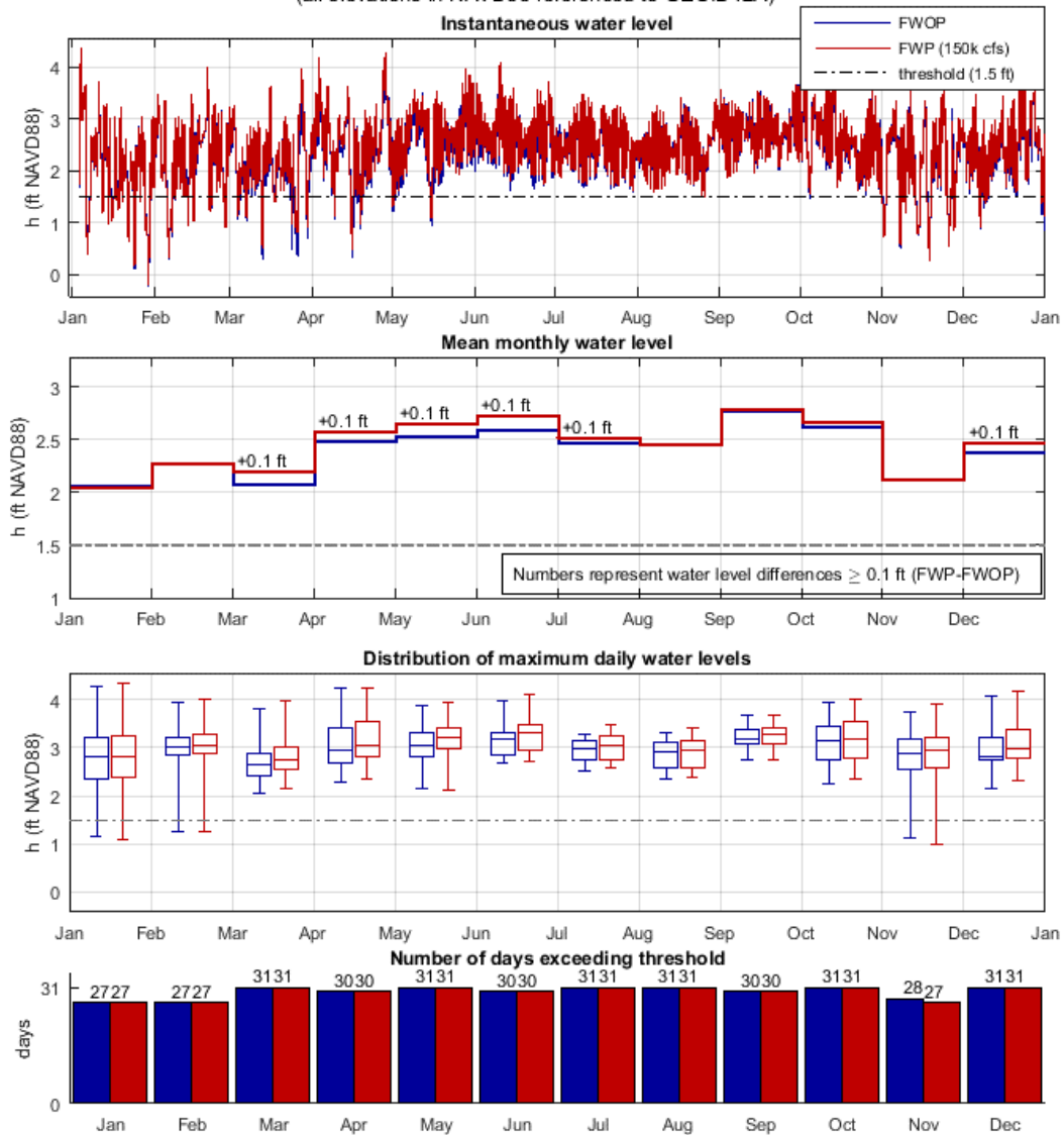
Figure C 19: Analysis of diversion impact on WSEs in Grand Bayou during the 2060s, FWOP and FWP (150k cfs), using the river hydrograph of year 2011. The top-most plot shows instantaneous water level (h). The second-from-the-top plot shows mean monthly water level (h). The third-from-the-top plot shows the distribution of maximum daily water levels (h) in box and whiskers plot format. The bottom plot shows the number of days exceeding the WSE threshold used for this community. Water level is referenced to NAVD88 (GEOID12A).
