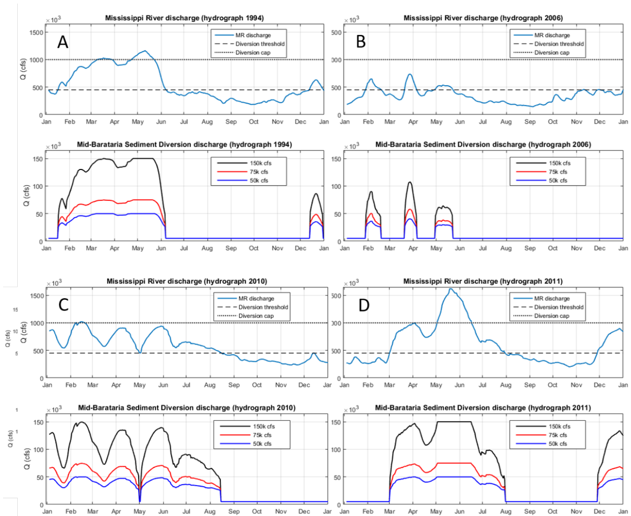
Figure 2: Mississippi River hydrographs (top of each graphs) and MBSD discharge for the 50k, 75k and 150k cfs diversion capacities (bottom of each graph) for 1994 (A), 2006 (B), 2010 (C), and 2011 (D)
