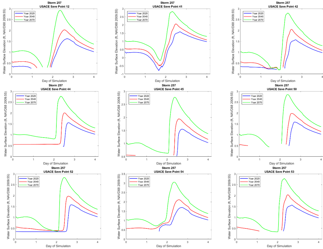
Figure 3-34. No Action Alternative Hydrographs at selected save points along the WBV for storm 257, 4 percent AEP storm, showing water surface elevation for year 2020 (blue), year 2040 (red), year 2070 (green).
