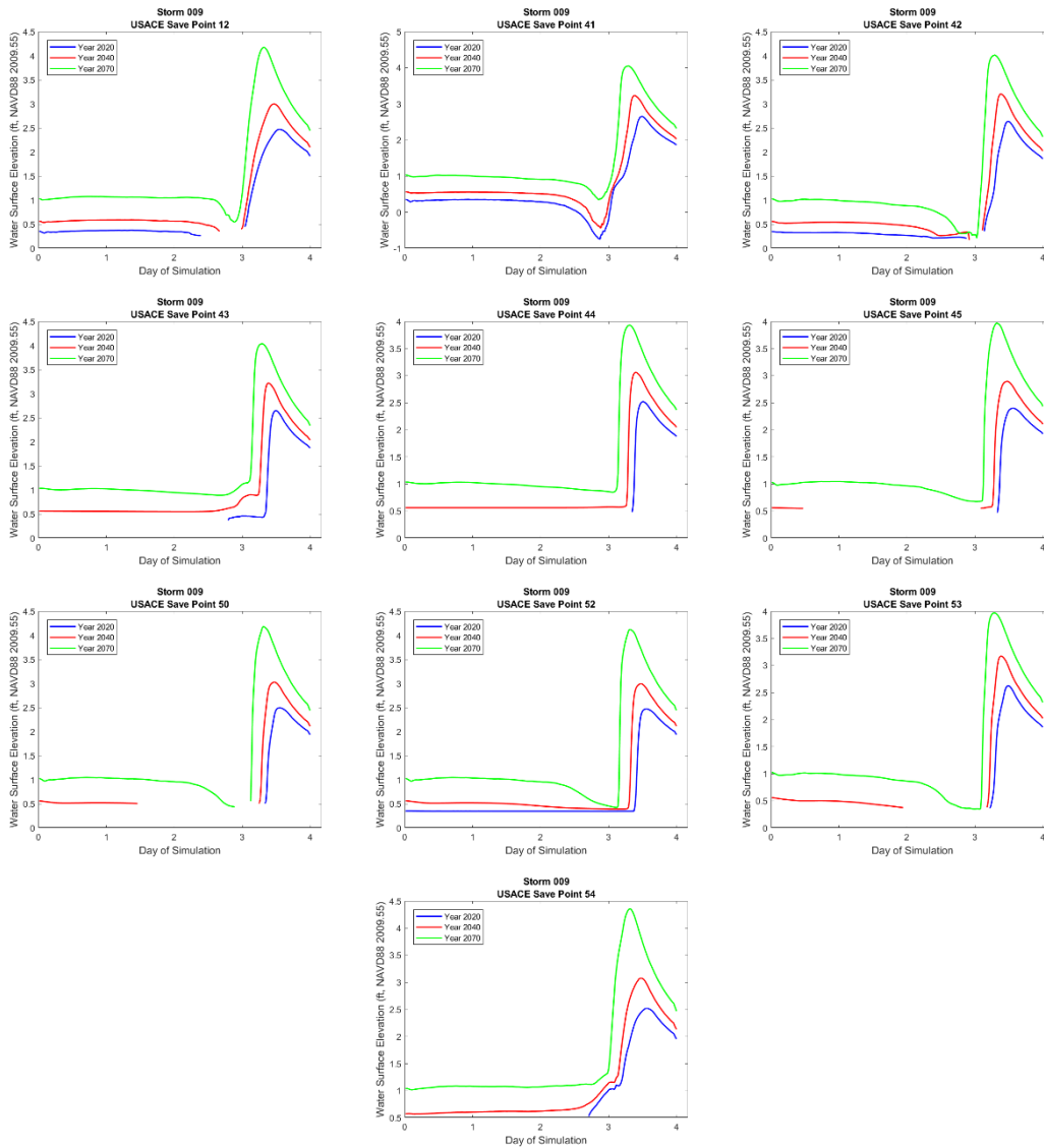
Figure 3-26. No Action Alternative Hydrographs at selected save points along the WBV for storm 009, 1 percent AEP storm, showing water surface elevation for year 2020 (blue), year 2040 (red), year 2070 (green).
