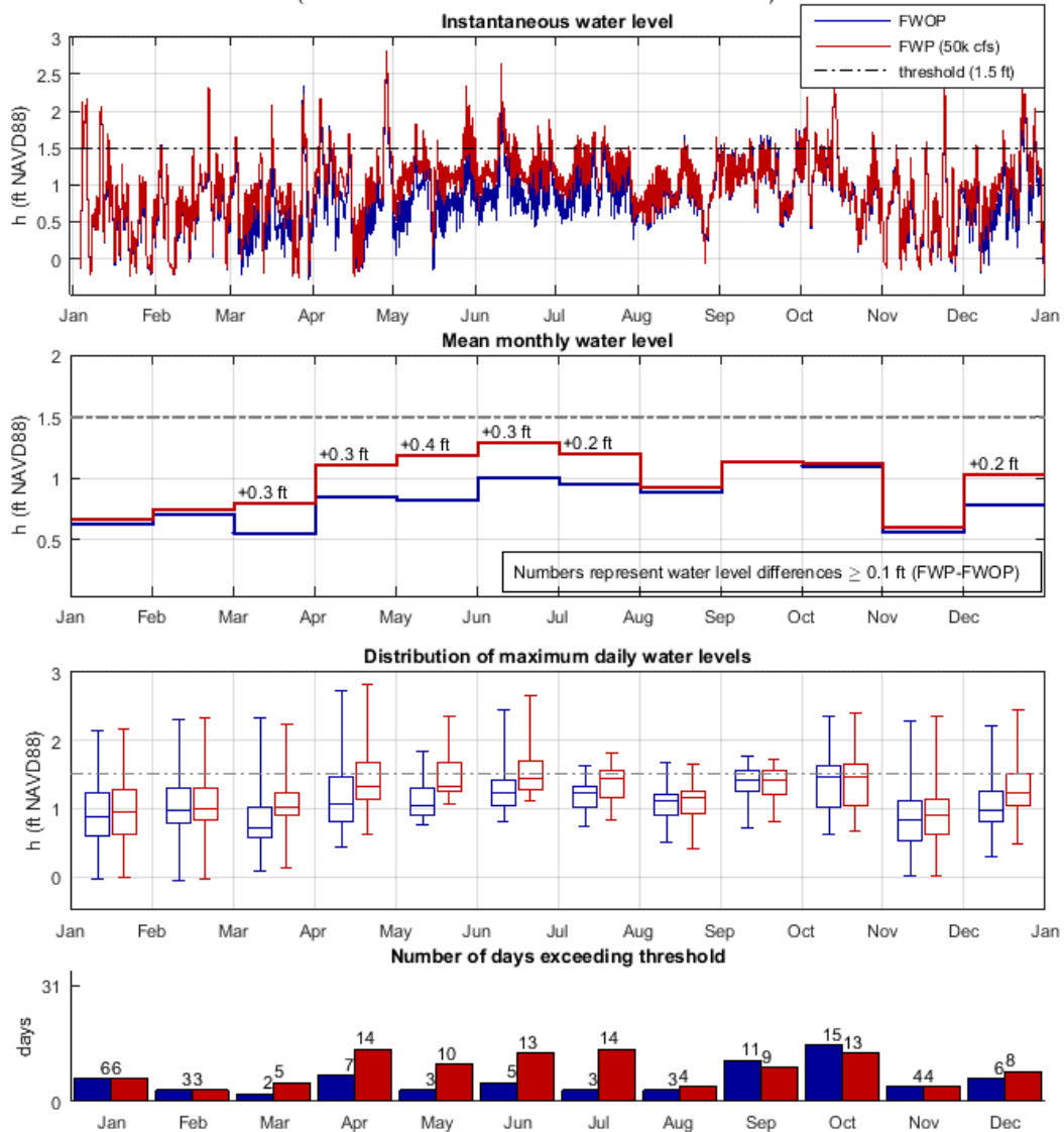
Figure C 3: Analysis of diversion impact on WSEs at Grand Bayou during the 2020s, FWOP and FWP (50k cfs), using the river hydrograph of year 2011. The top-most plot shows instantaneous water level (h). The second-from-the-top plot shows mean monthly water level (h). The third-from-the-top plot shows the distribution of maximum daily water levels (h) in box and whiskers plot format. The bottom plot shows the number of days exceeding the WSE threshold used for this community. Water level is referenced to NAVD88 (GEOID12A).
