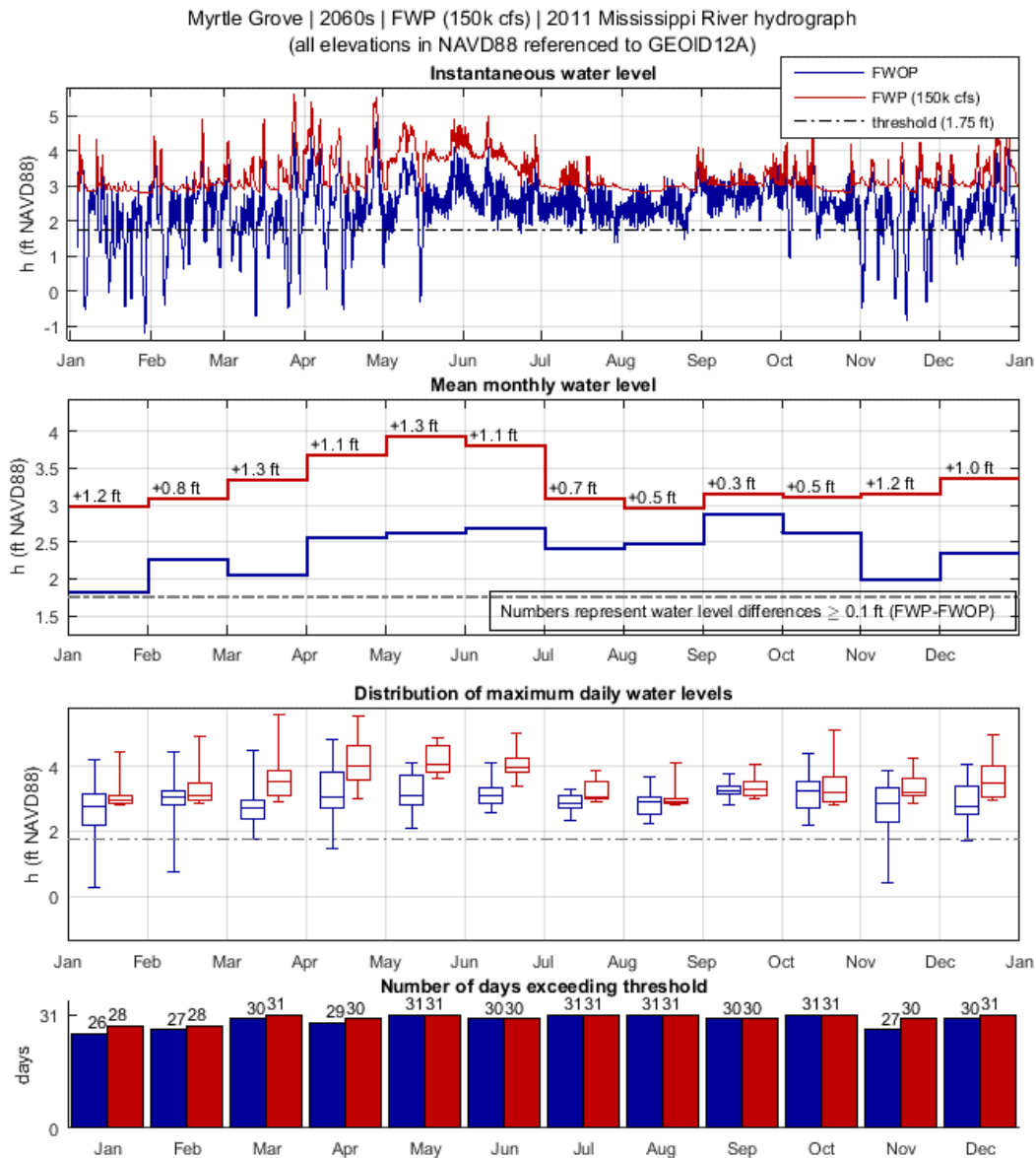
Figure C 17: Analysis of diversion impact on WSEs in Myrtle Grove during the 2060s, FWOP and FWP (150k cfs), using the river hydrograph of year 2011. The top-most plot shows instantaneous water level (h). The second-from-the-top plot shows mean monthly water level (h). The third-from-the-top plot shows the distribution of maximum daily water levels (h) in box and whiskers plot format. The bottom plot shows the number of days exceeding the WSE threshold used for this community. Water level is referenced to NAVD88 (GEOID12A).
