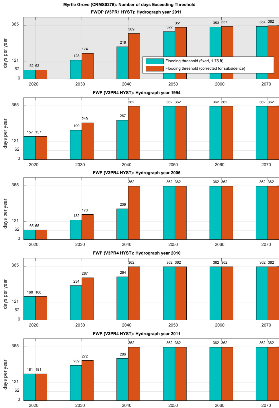
Figure 33: Analysis of the threshold exceedance rates in Myrtle Grove over time. Number of days exceeding the fixed WSE threshold elevation (green) and the corrected threshold elevation (orange). The figure consists of the 2011 FWOP results for reference (grey background) and the 1994, 2006, 2010 and 2011 FWP results (white background).
