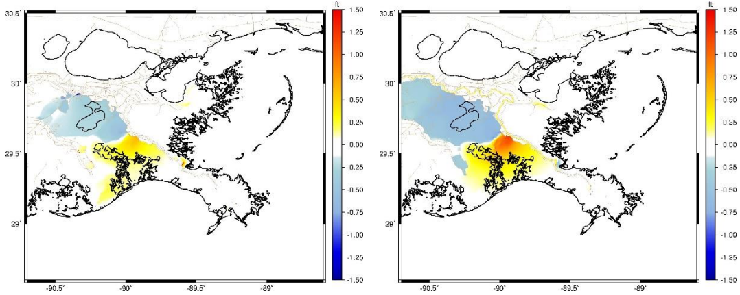
Figure 3-56. Maximum water surface elevation difference between the Applicant's Preferred Alternative and the No Action Alternative storm 245, 1 percent AEP storm, year 2040 (left), year 2070 (right).
