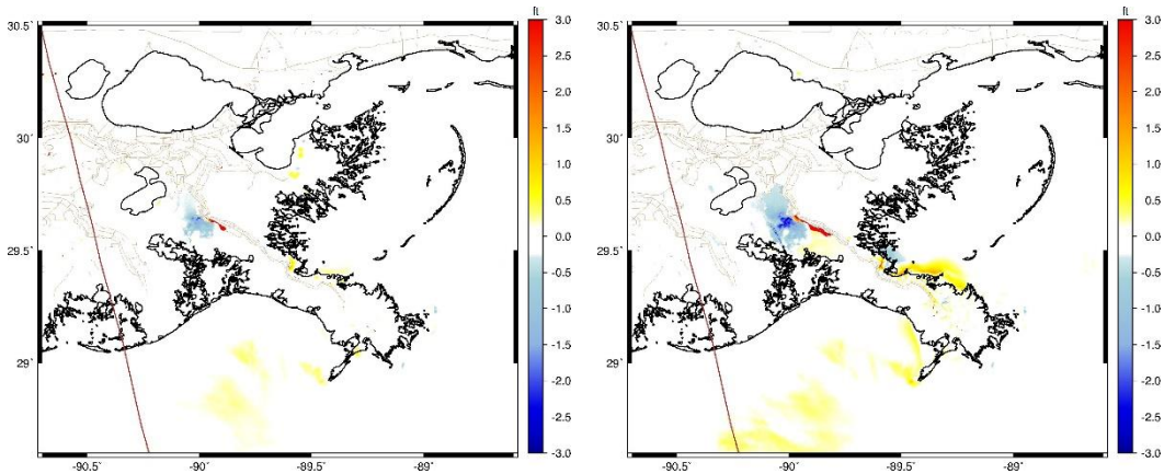
Figure 3-47. Maximum wave height difference between the Applicant's Preferred Alternative and the No Action Alternative for storm 014, 1 percent AEP storm, year 2040 (left), year 2070 (right).
