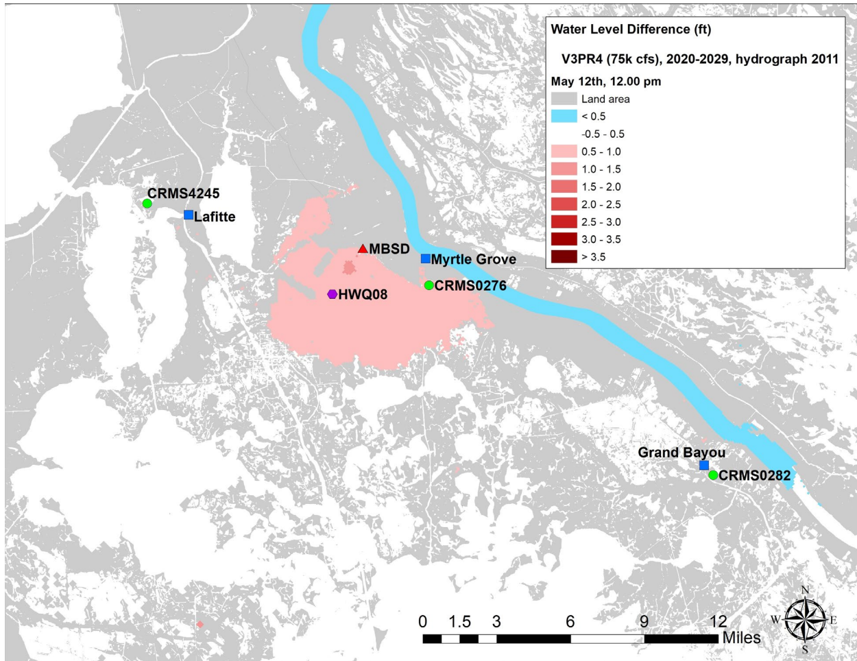
Figure 32: Difference in instantaneous WSEs for FWOP (V3PR1) and FWP (V3PR4, 75k cfs) during a wind driven peak event during the 2020s, on May 12 th , 2011 at noon.
