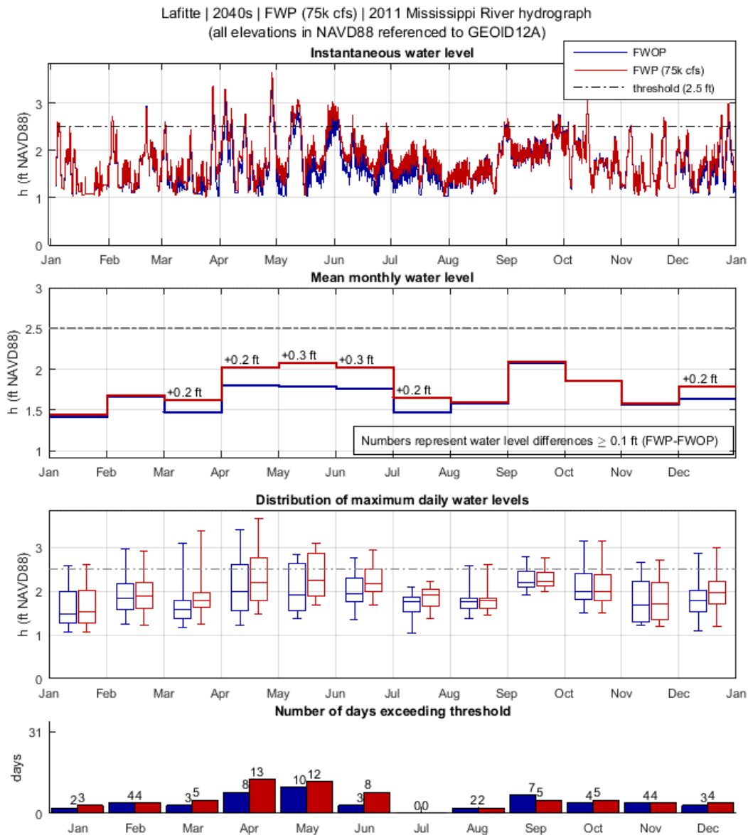
Figure 21: Analysis of diversion impact on WSEs in Lafitte during the 2040s, FWOP and FWP (75k cfs), using the river hydrograph of year 2011. The top-most plot shows instantaneous water level (h). The second-from-the-top plot shows mean monthly water level (h). The third-from-the-top plot shows the distribution of maximum daily water levels (h) in box and whiskers plot format. The bottom plot shows the number of days exceeding the WSE threshold used for this community. Water level is referenced to NAVD88 (GEOID12A).
