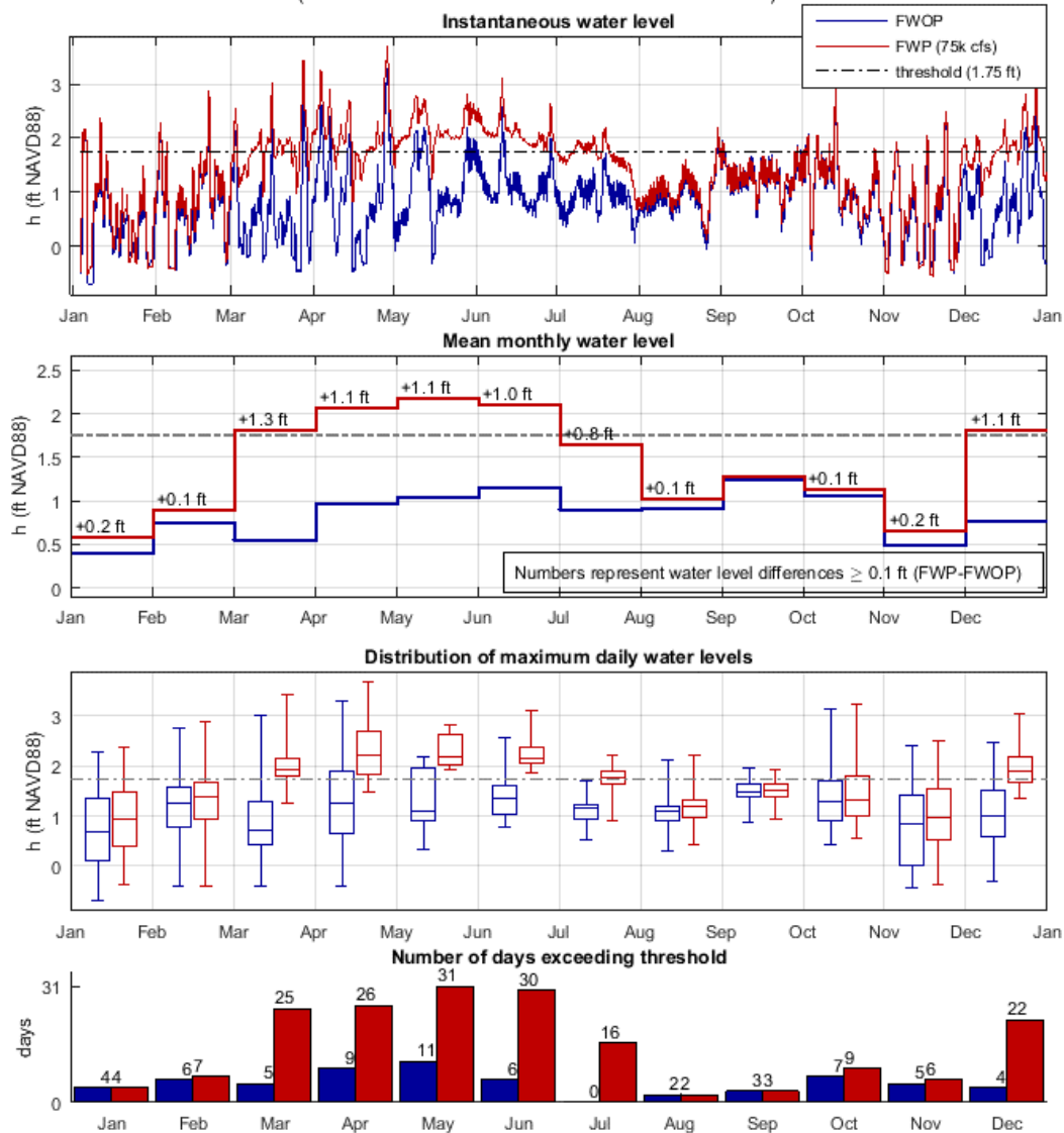
Figure 17: Analysis of diversion impact on WSEs in Myrtle Grove during the 2020s, FWOP and FWP (75k cfs), using the river hydrograph of year 2011. The top-most plot shows instantaneous water level (h). The second-from-the-top plot shows mean monthly water level (h). The third-from-the-top plot shows the distribution of maximum daily water levels (h) in box and whiskers plot format. The bottom plot shows the number of days exceeding the WSE threshold used for this community. Water level is referenced to NAVD88 (GEOID12A).
