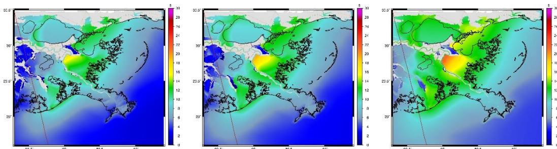
Figure 3-8. No Action Alternative maximum water surface elevation for storm 014, 1 percent AEP storm, year 2020 (left), year 2040 (middle), year 2070 (right).
