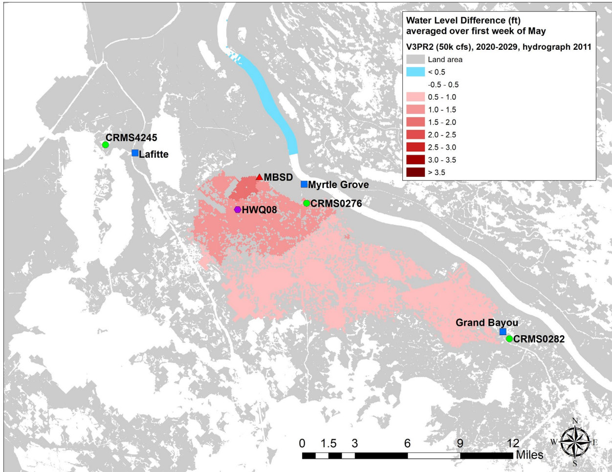
Figure C 10: Average water level difference between FWOP (V3PR1) and FWP (V3PR2, 50k cfs) for the first week of May (in the 2020s), when the diversion is at maximum capacity (50k cfs). 2011 hydrograph.
