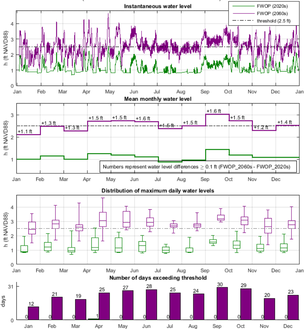
Figure 14: WSE analysis for Lafitte, FWOP for the first decade (2020s, in green) and the fifth decade (2060s, in purple), using the hydrograph of year 2011. The top-most plot shows instantaneous water level (h). The second-from-the-top plot shows mean monthly water level (h). The third-from-the-top plot shows the distribution of maximum daily water levels (h) in box and whiskers plot format. The bottom plot shows the number of days exceeding the WSE threshold used for this community. Water level is referenced to NAVD88 (GEOID12A).
