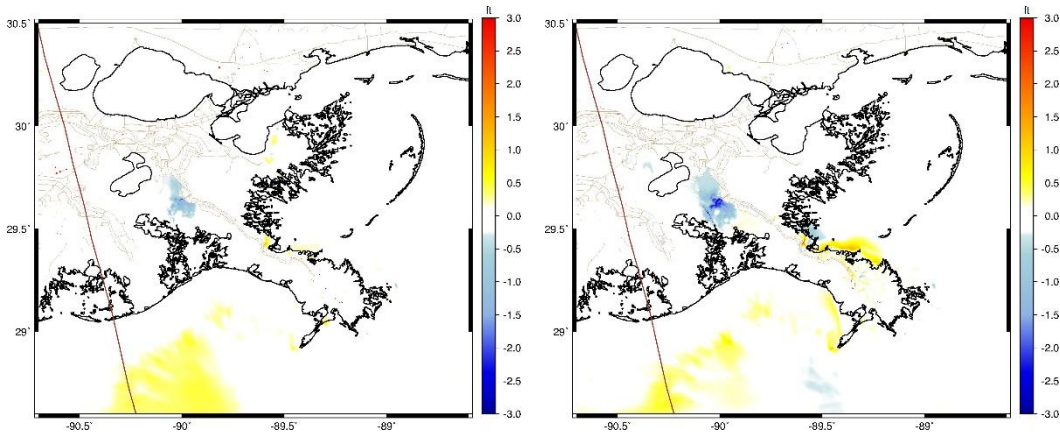
Figure 3-43. Maximum wave height difference between the Applicant's Preferred Alternative and the No Action Alternative for storm 011, 4 percent AEP storm, year 2040 (left), year 2070 (right).
