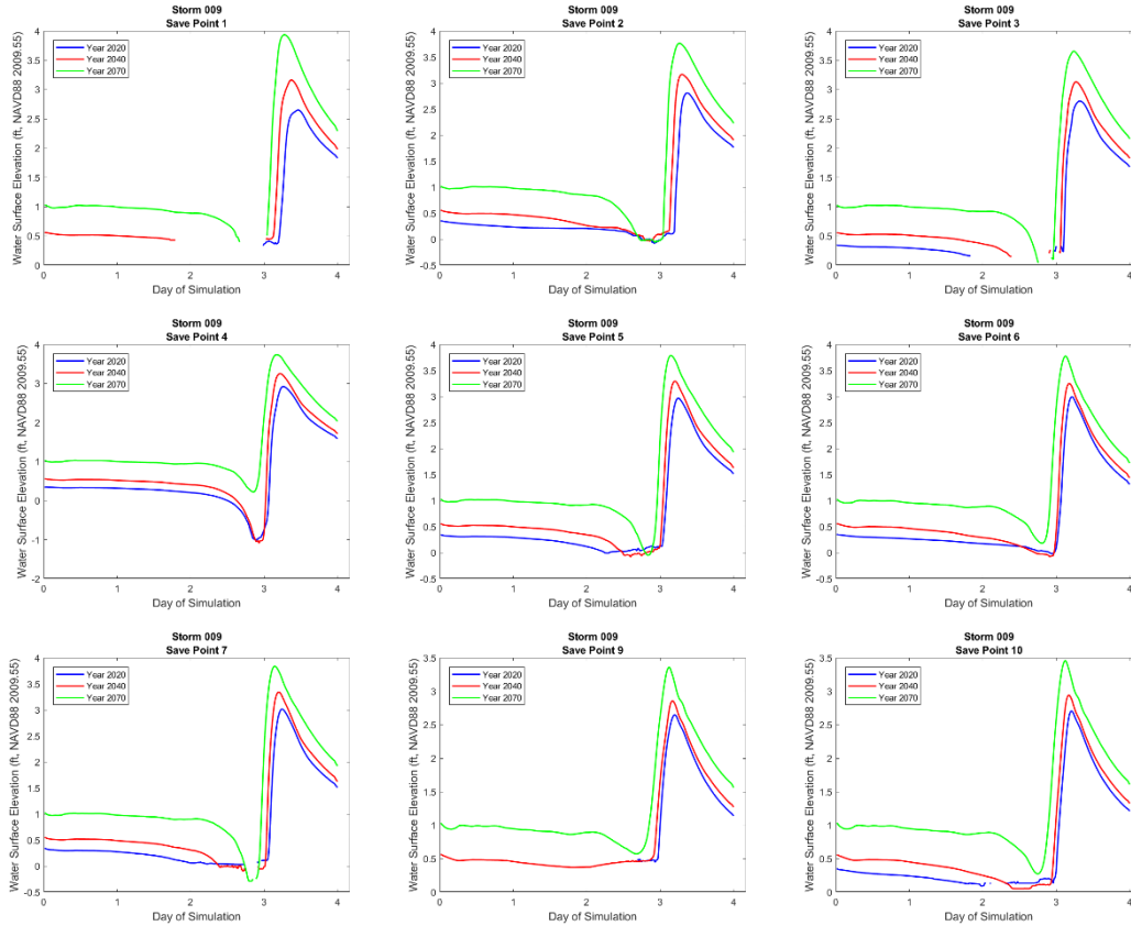
Figure 3-24. No Action Alternative Hydrographs at selected save points along the NOV-NFL for storm 009, 1 percent AEP storm, showing water surface elevation for year 2020 (blue), year 2040 (red), year 2070 (green).
