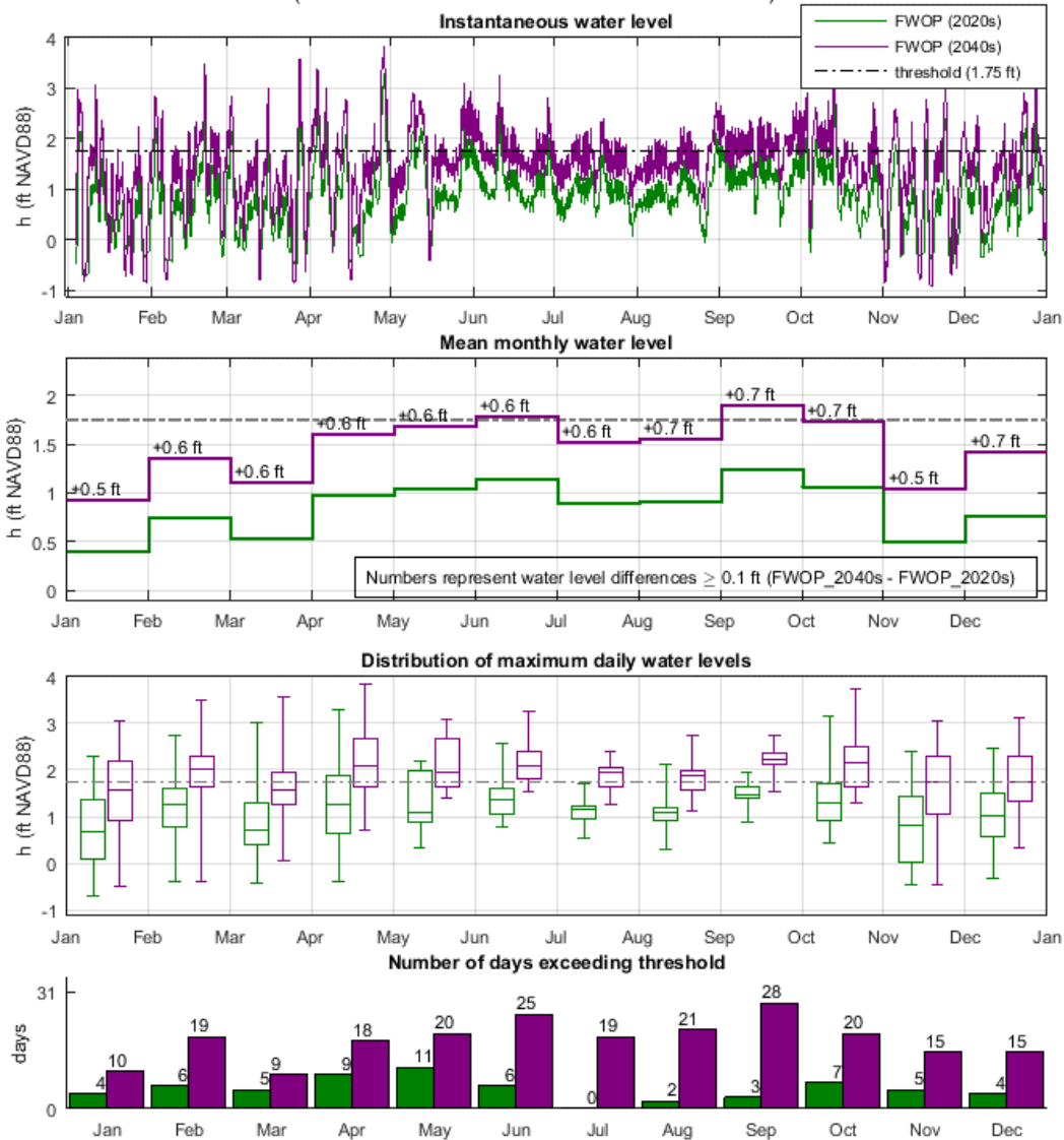
Figure 12: WSE analysis for Myrtle Grove, FWOP for the first decade (2020s, in green) and the third decade (2040s, in purple), using the hydrograph of year 2011. The top-most plot shows instantaneous water level (h). The second-from-the-top plot shows mean monthly water level (h). The third-from-the-top plot shows the distribution of maximum daily water levels (h) in box and whiskers plot format. The bottom plot shows the number of days exceeding the WSE threshold used for this community. Water level is referenced to NAVD88 (GEOID12A).
