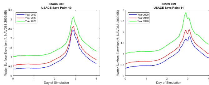
Figure 3-28. No Action Alternative Hydrographs at selected save points near Grand Isle for storm 009, 1 percent AEP storm, showing water surface elevation for year 2020 (blue), year 2040 (red), year 2070 (green).
