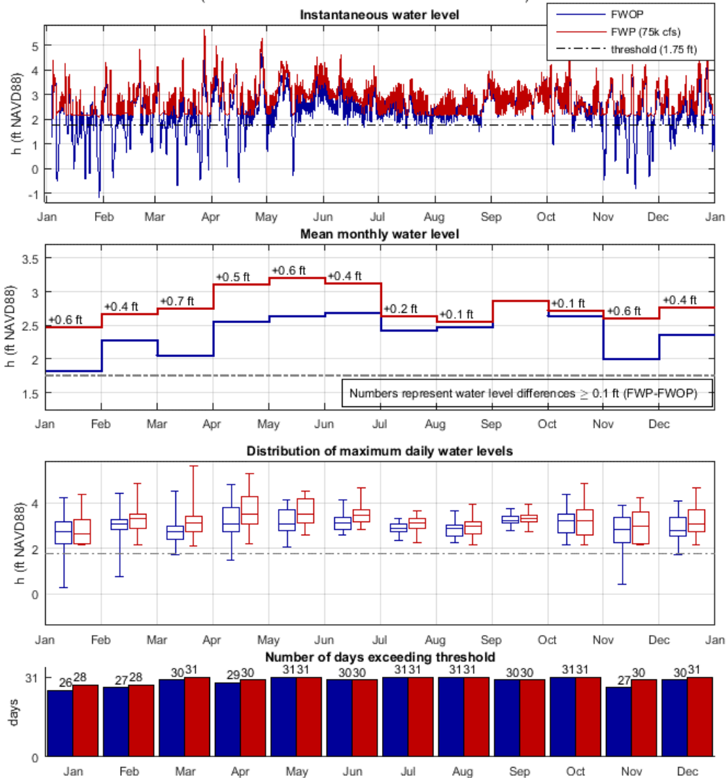
Figure 23. Analysis of diversion impact on WSEs in Myrtle Grove during the 2060s, FWOP and FWP (75k cfs), using the river hydrograph of year 2011. The top-most plot shows instantaneous water level (h). The second-from-the-top plot shows mean monthly water level (h). The third-from-the-top plot shows the distribution of maximum daily water levels (h) in box and whiskers plot format. The bottom plot shows the number of days exceeding the WSE threshold used for this community. Water level is referenced to NAVD88 (GEOID12A).
