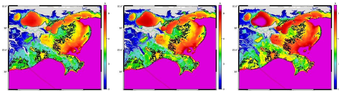
Figure 3-11. No Action Alternative maximum wave height for storm 093, 1 percent AEP storm, year 2020 (left), year 2040 (middle), year 2070 (right).
