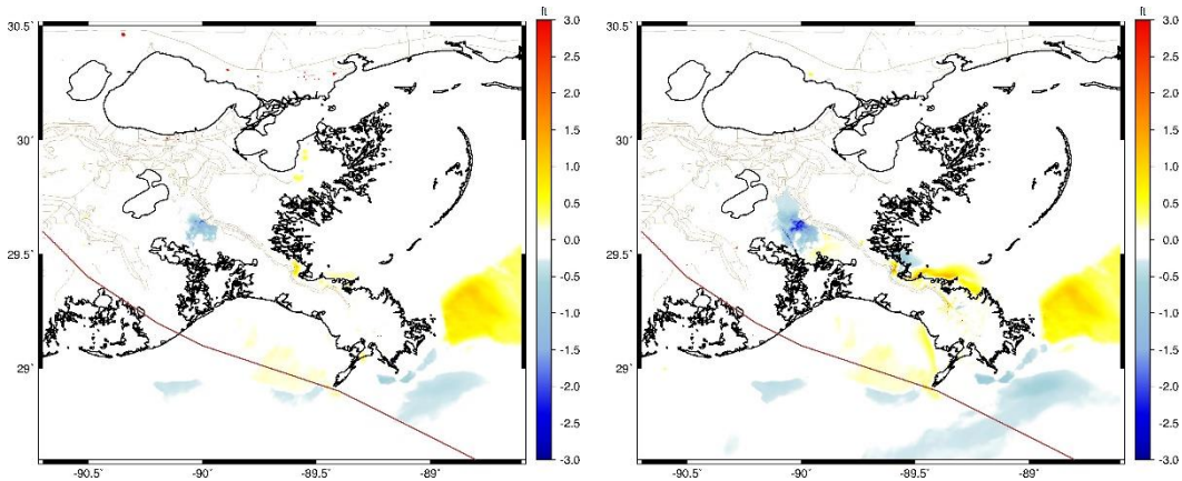
Figure 3-61. Maximum wave height difference between the Applicant's Preferred Alternative and the No Action Alternative for storm Isaac, year 2040 (left), year 2070 (right).
