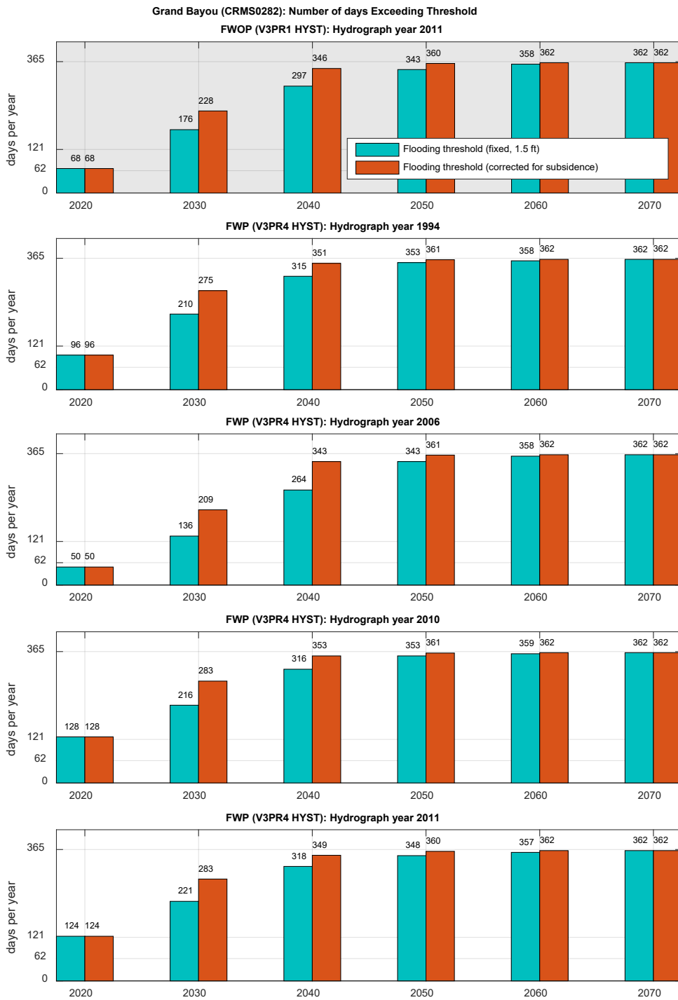
Figure 35: Analysis of the threshold exceedance rates in Grand Bayou over time. Number of days exceeding the fixed WSE threshold elevation (green) and the corrected threshold elevation (orange). The figure consists of the 2011 FWOP results for reference (grey background) and the 1994, 2006, 2010 and 2011 FWP results (white background).
