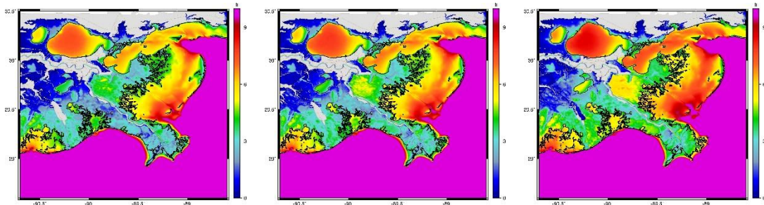
Figure 3-21. No Action Alternative maximum wave height for storm 257, 4 percent AEP storm, year 2020 (left), year 2040 (middle), year 2070 (right).
