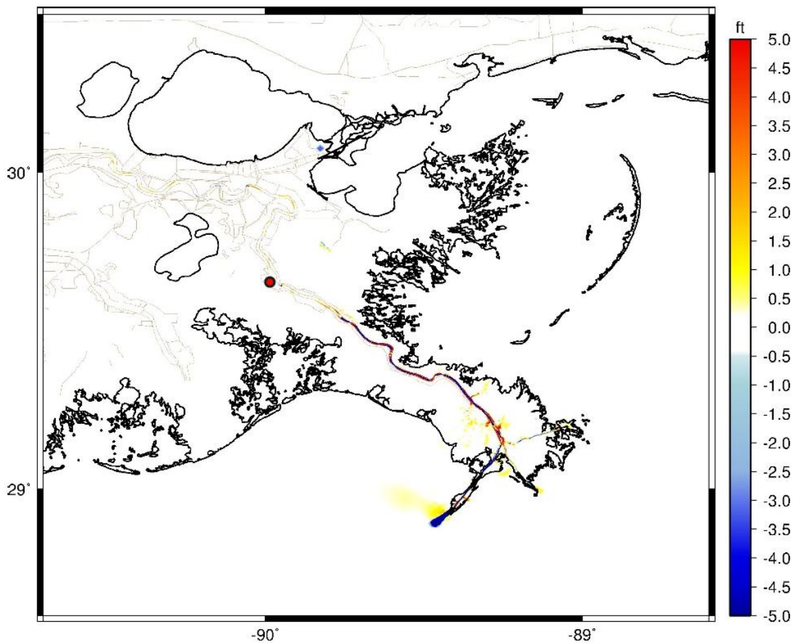
Figure 2-7. Topography and Bathymetry Differences between the 2017 Master Plan Model and the Mid-Barataria Sediment Diversion Model Year 2020.
