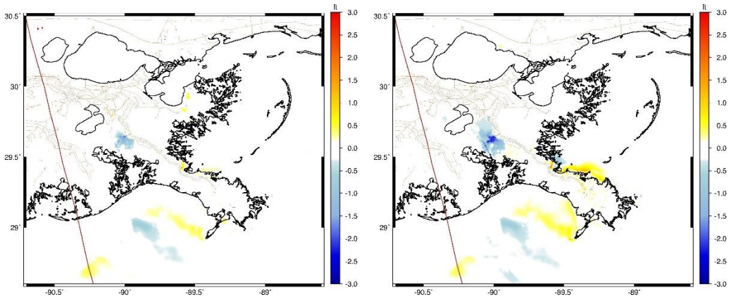
Figure 3-45. Maximum wave height difference between the Applicant's Preferred Alternative and the No Action Alternative for storm 011 slow, 4 percent AEP storm, year 2040 (left), year 2070 (right).
