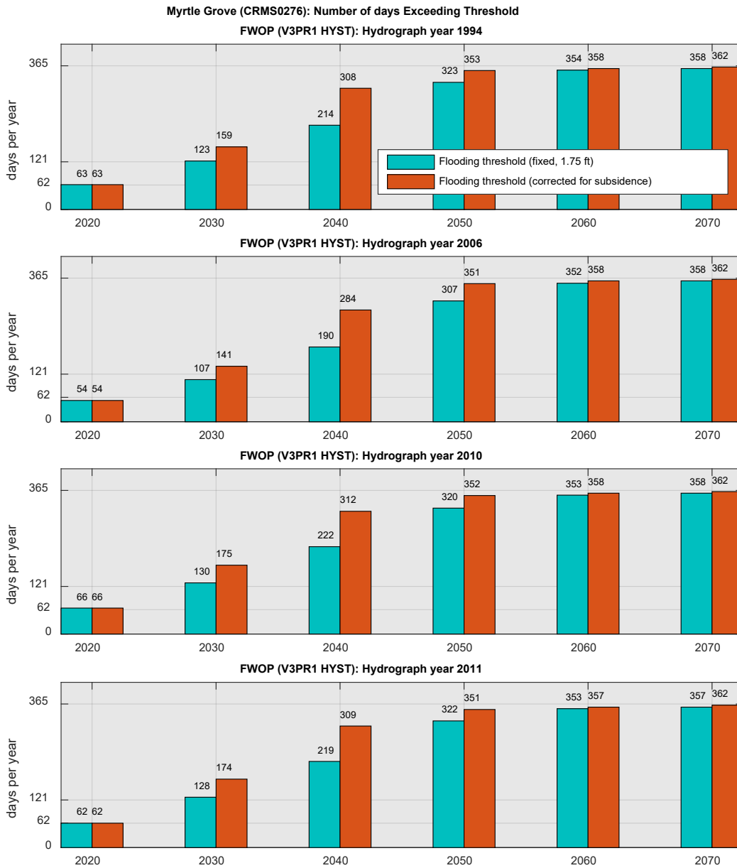
Figure 8: Analysis of the threshold exceedance rates in Myrtle Grove over time, FWOP simulation, all hydrographs. Annual number of days exceeding the fixed WSE threshold elevation (green) and the threshold elevation corrected for subsidence (orange).
