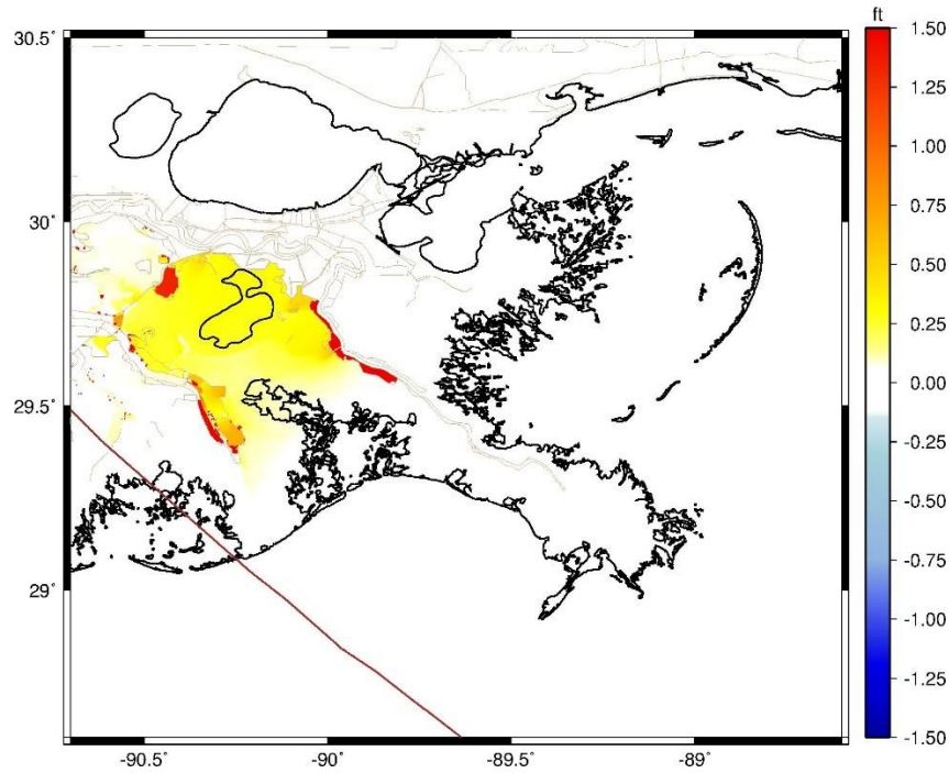
Figure 4-3. Peak water level difference for 2040 Applicant’s Preferred Alternative Partially Open less 2040 Applicant’s Preferred Alternative during 1 percent AEP event (Storm 093) in September water level conditions.
