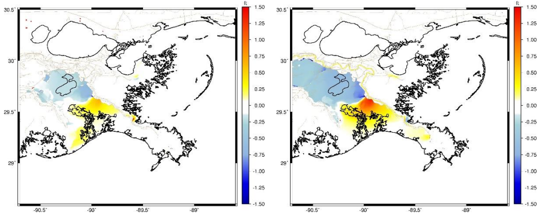
Figure 3-50. Maximum water surface elevation difference between the Applicant's Preferred Alternative and the No Action Alternative storm 101, 4 percent AEP storm, year 2040 (left), year 2070 (right).
