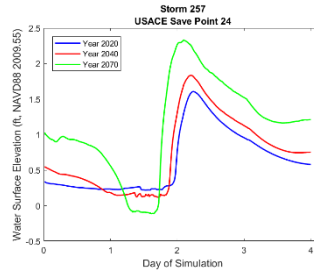
Figure 3-39. No Action Alternative Hydrographs at save point near Grand Bayou for storm 257, 4 percent AEP storm, showing water surface elevation for year 2020 (blue), year 2040 (red), year 2070 (green).
