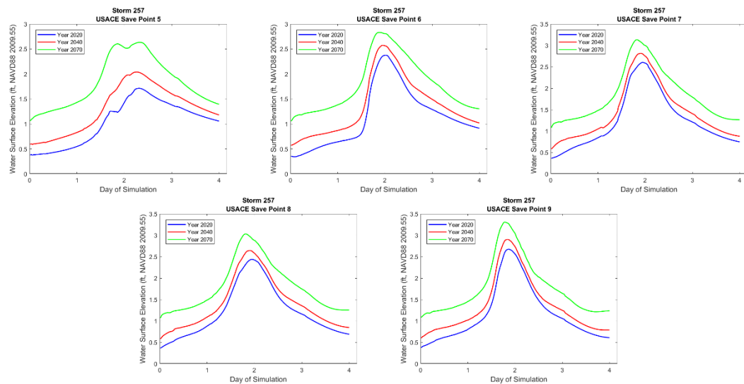
Figure 3-35. No Action Alternative Hydrographs at selected save points near the LGM for storm 257, 4 percent AEP storm, showing water surface elevation for year 2020 (blue), year 2040 (red), year 2070 (green).
