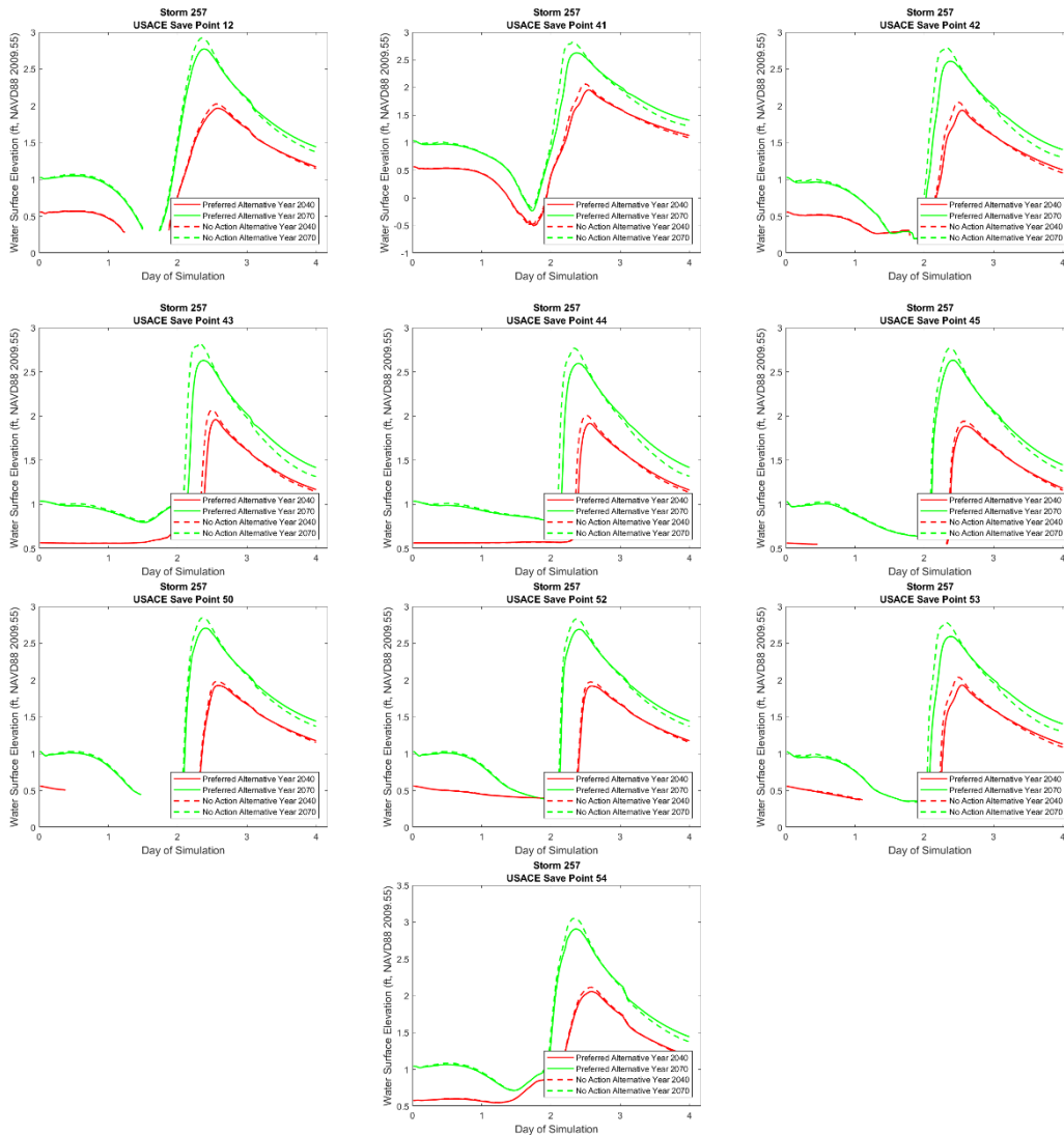
Figure 3-72. Hydrographs at selected save points along the WBV for storm 257, 4 percent AEP storm, showing water surface elevation for the No Action Alternative (red hashed 2040, green hashed 2070) and Applicant’s Preferred Alternative (red solid 2040, green solid 2070).
