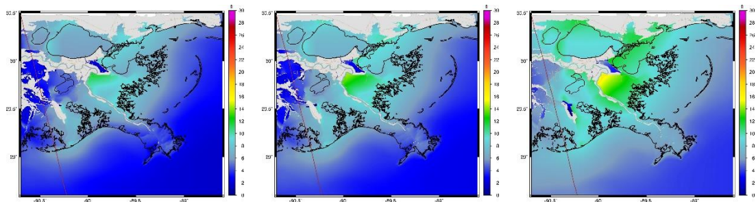
Figure 3-4. No Action Alternative maximum water surface elevation for storm 011, 4 percent AEP storm, year 2020 (left), year 2040 (middle), year 2070 (right).
