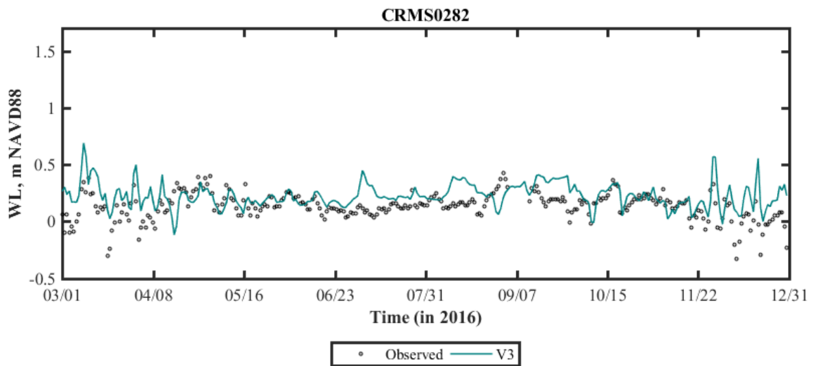
Figure B 6.V3 Basinwide model validation of daily water level (WL) at CRMS0282 (Grand Bayou community), in Barataria Basin (2016).
