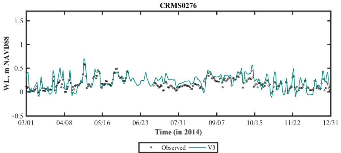
Figure B 1.V3 Basinwide model calibration of daily water level (WL) at CRMS0276 (Myrtle Grove community), in Barataria Basin (2014).
