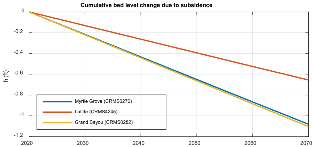
Figure 4: Bed level change applied in the Basinwide model due to subsidence at the three communities where h is ground elevation relative to year 2020.
