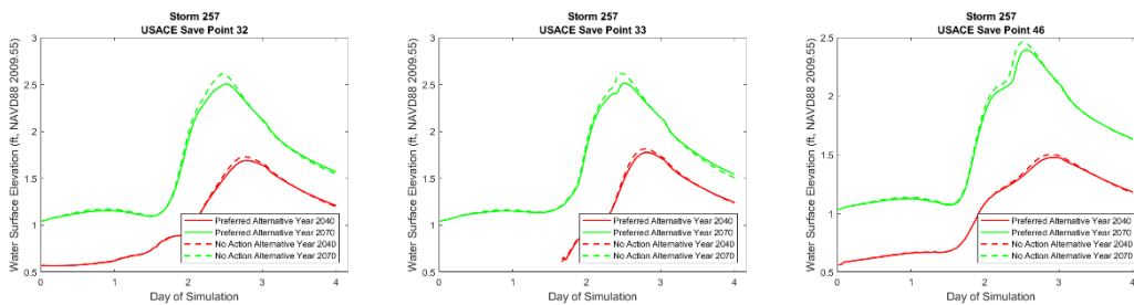
Figure 3-76. Hydrographs at selected save points near Des Allemandes/ Bayou Gauche for storm 257, 4 percent AEP storm, showing water surface elevation the No Action Alternative (red hashed 2040, green hashed 2070) and Applicant’s Preferred Alternative (red solid 2040, green solid 2070).
