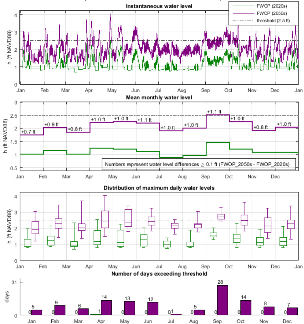
Figure 13: WSE analysis for Lafitte, FWOP for the first decade (2020s, in green) and the fourth decade (2050s, in purple), using the hydrograph of year 2011. The top-most plot shows instantaneous water level (h). The second-from-the-top plot shows mean monthly water level (h). The third-from-the-top plot shows the distribution of maximum daily water levels (h) in box and whiskers plot format. The bottom plot shows the number of days exceeding the WSE threshold used for this community. Water level is referenced to NAVD88 (GEOID12A).
