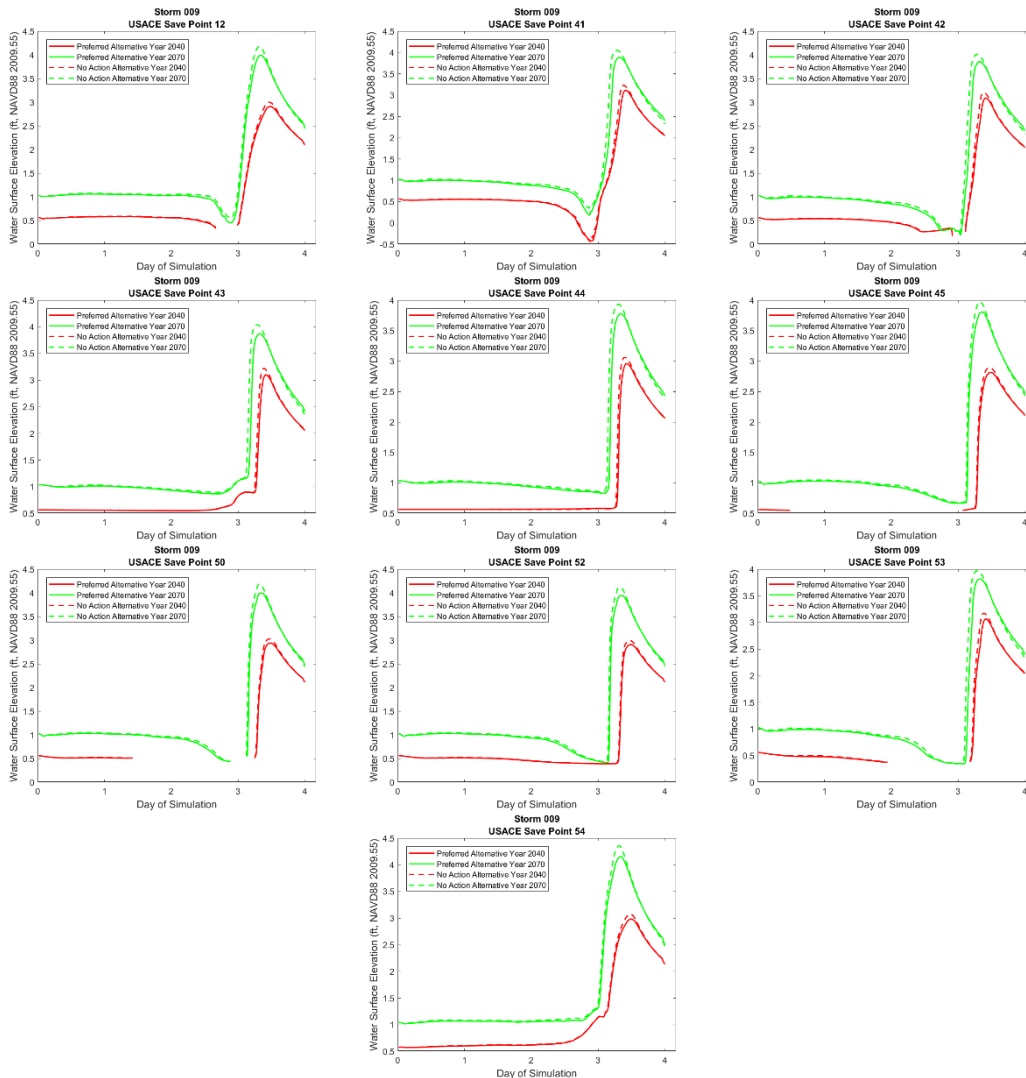
Figure 3-64. Hydrographs at selected save points along the WBV for storm 009, 1 percent AEP storm, showing water surface elevation for the No Action Alternative (red hashed 2040, green hashed 2070) and Applicant’s Preferred Alternative (red solid 2040, green solid 2070).
