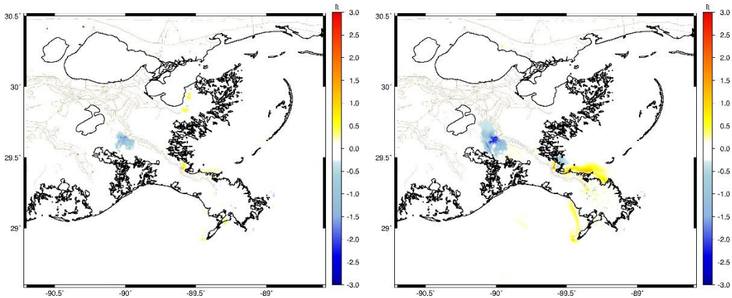
Figure 3-57. Maximum wave height difference between the Applicant's Preferred Alternative and the No Action Alternative for storm 245, 1 percent AEP storm, year 2040 (left), year 2070 (right).
