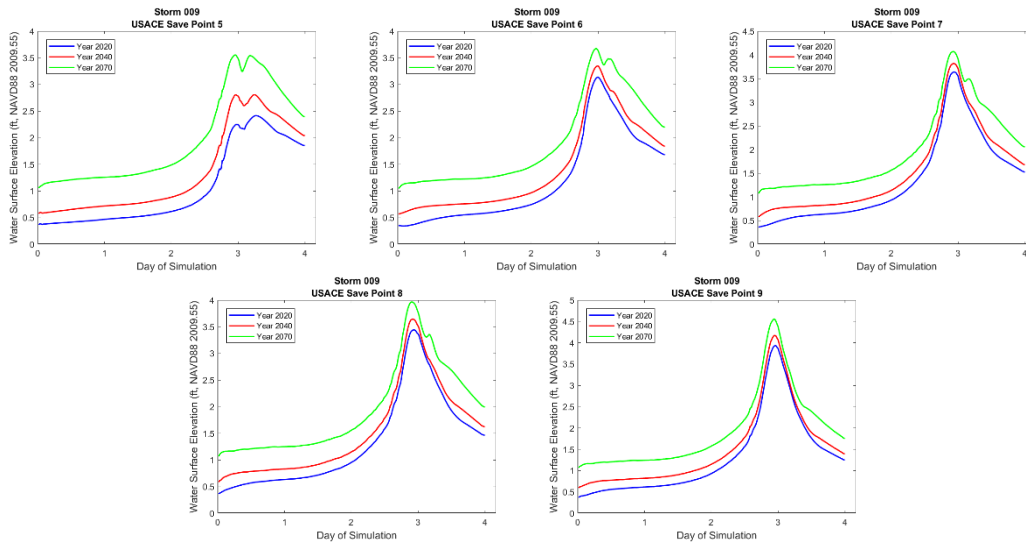
Figure 3-27. No Action Alternative Hydrographs at selected save points near the LGM for storm 009, 1 percent AEP storm, showing water surface elevation for year 2020 (blue), year 2040 (red), year 2070 (green).
