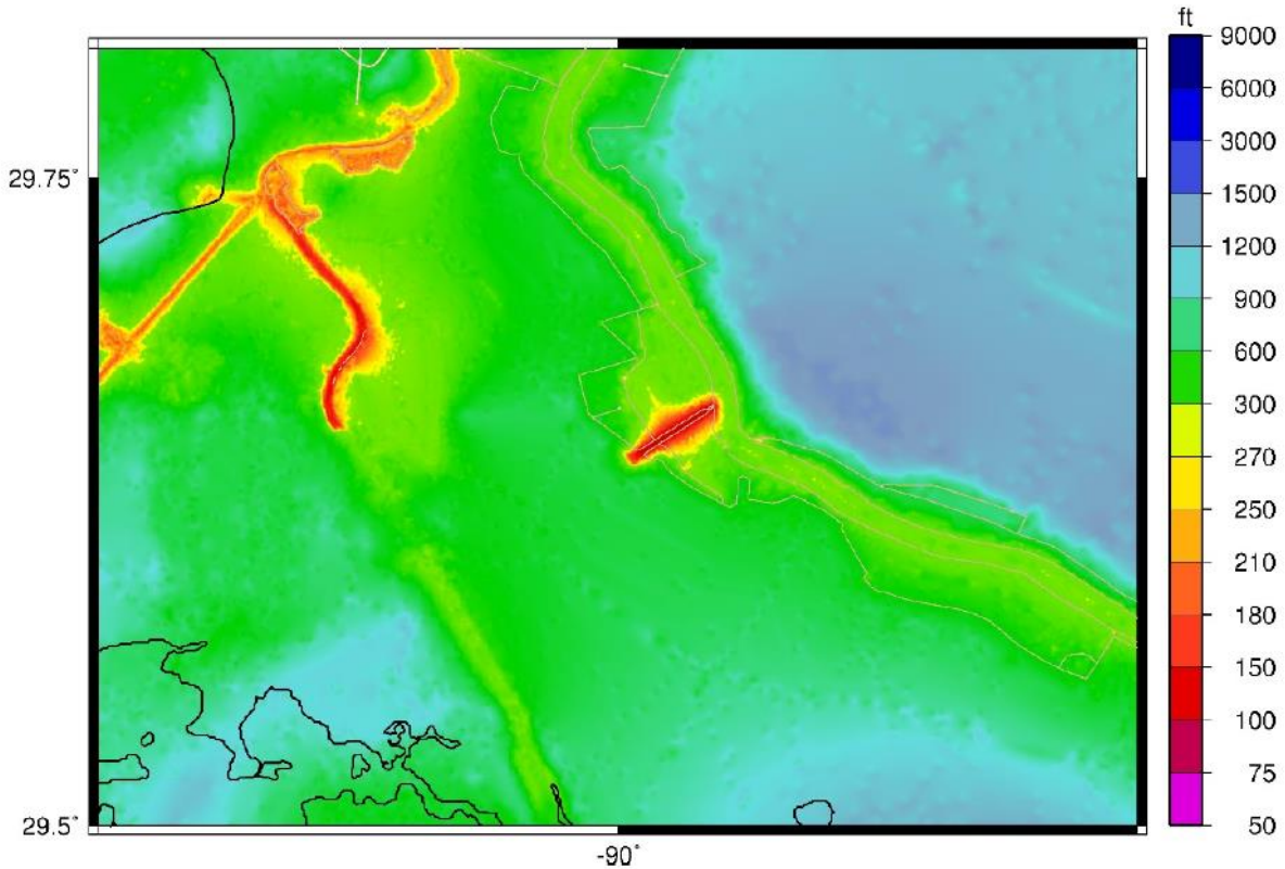
Figure 2-5. Mesh Resolution for the Mid-Barataria Sediment Diversion ADCIRC Model.
