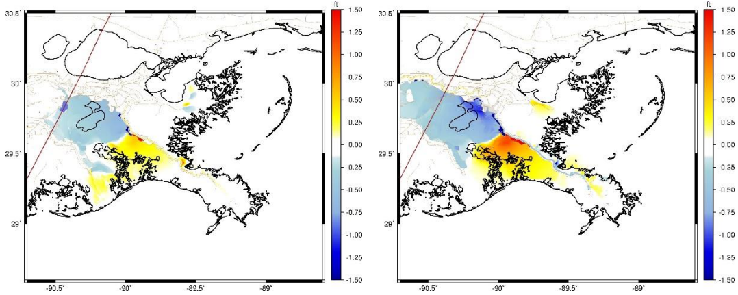
Figure 3-52. Maximum water surface elevation difference between the Applicant's Preferred Alternative and the No Action Alternative storm 160, 1 percent AEP storm, year 2040 (left), year 2070 (right).
