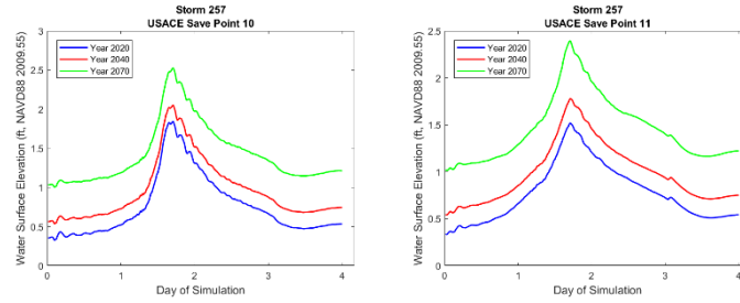
Figure 3-36. No Action Alternative Hydrographs at selected save points near Grand Isle for storm 257, 4 percent AEP storm, showing water surface elevation for year 2020 (blue), year 2040 (red), year 2070 (green).
