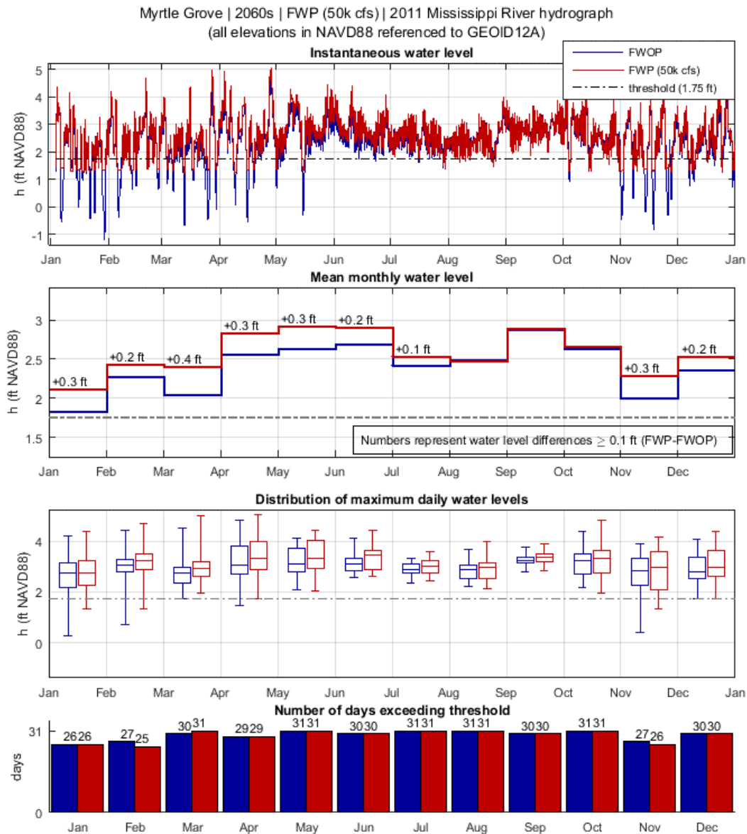
Figure C 7: Analysis of diversion impact on WSEs in Myrtle Grove during the 2060s, FWOP and FWP (50k cfs), using the river hydrograph of year 2011. The top-most plot shows instantaneous water level (h). The second-from-the-top plot shows mean monthly water level (h). The third-from-the-top plot shows the distribution of maximum daily water levels (h) in box and whiskers plot format. The bottom plot shows the number of days exceeding the WSE threshold used for this community. Water level is referenced to NAVD88 (GEOID12A).
