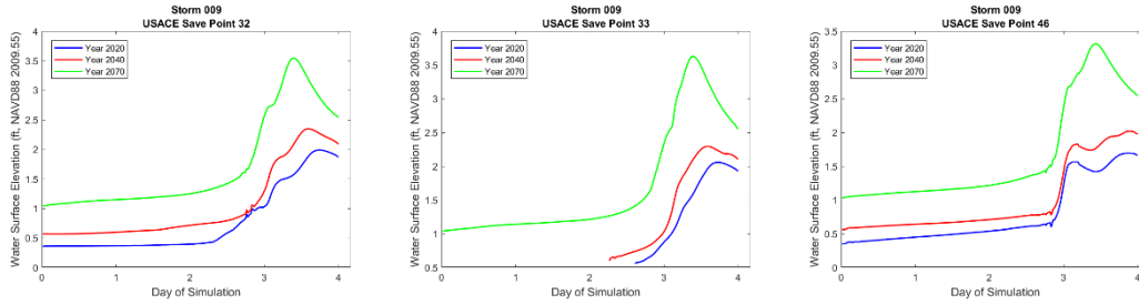
Figure 3-30. No Action Alternative Hydrographs at selected save points near Des Allemandes/ Bayou Grande for storm 009, 1 percent AEP storm, showing water surface elevation for year 2020 (blue), year 2040 (red), year 2070 (green).
