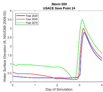
Figure 3-31. No Action Alternative Hydrographs at a save point near Grand Bayou for storm 009, 1 percent AEP storm, showing water surface elevation for year 2020 (blue), year 2040 (red), year 2070 (green).
