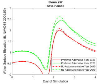
Figure 3-75. Hydrographs at a save point near Lafitte for storm 257, 4 percent AEP storm, showing water surface elevation for the No Action Alternative (red hashed 2040, green hashed 2070) and Applicant’s Preferred Alternative (red solid 2040, green solid 2070).
