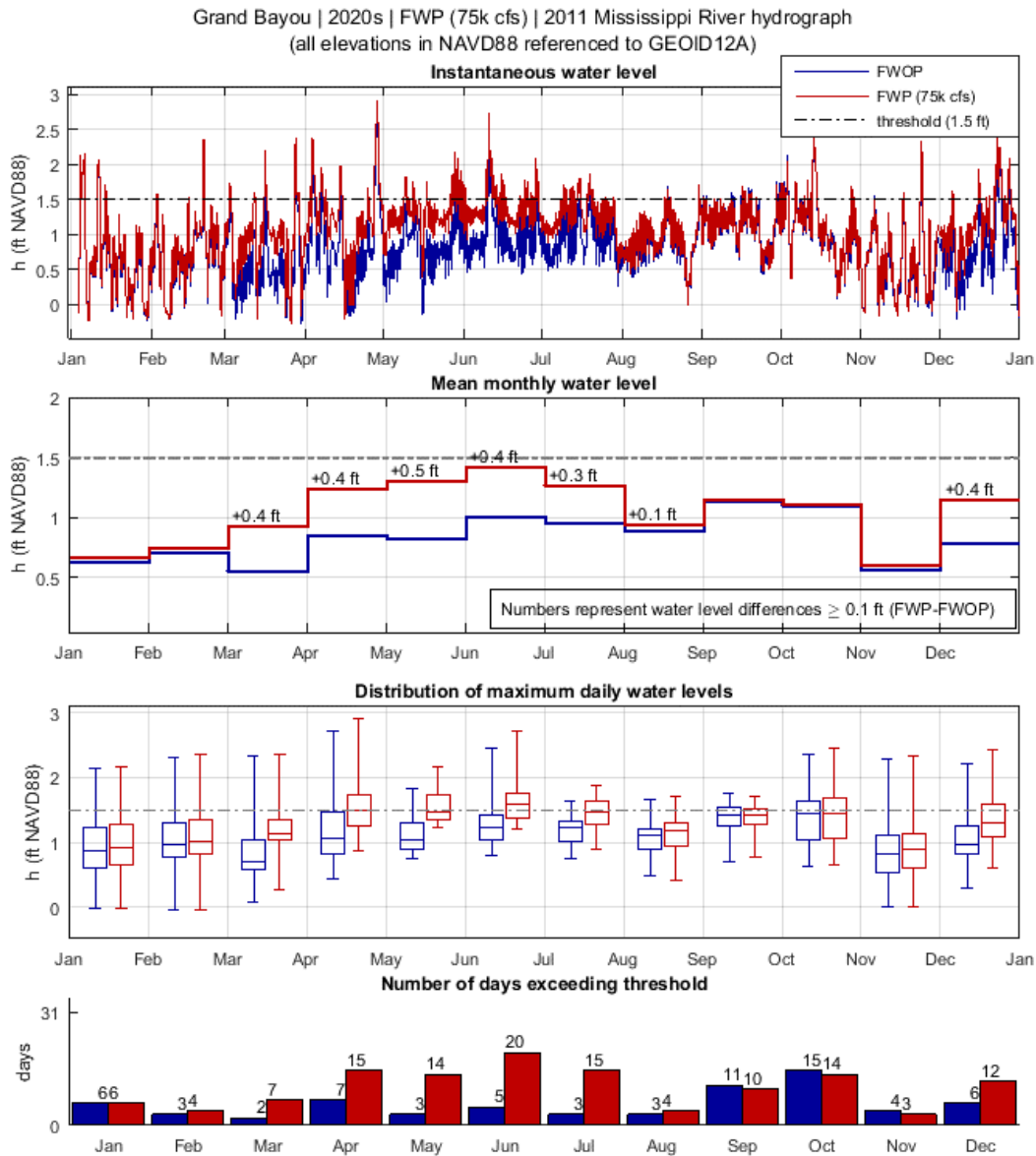
Figure 19: Analysis of diversion impact on WSEs in Grand Bayou during the 2020s, FWOP and FWP (75k cfs), using the river hydrograph of year 2011. The top-most plot shows instantaneous water level (h). The second-from-the-top plot shows mean monthly water level (h). The third-from-the-top plot shows the distribution of maximum daily water levels (h) in box and whiskers plot format. The bottom plot shows the number of days exceeding the WSE threshold used for this community. Water level is referenced to NAVD88 (GEOID12A).
