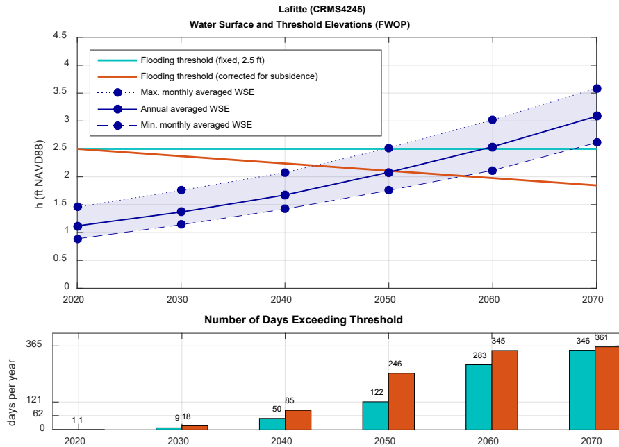
Figure 6: Analysis of the WSE in Lafitte over time, FWOP simulation, 2011 hydrograph. (Top graph) Annual average WSE (blue solid line) and its range of variation (min/max monthly average, blue dotted lines), fixed WSE thresholds (green line) and WSE threshold corrected with subsidence (orange line). (Bottom graph) Annual number of days exceeding the fixed WSE threshold elevation (green) and the corrected threshold elevation (orange). WSE is referenced to NAVD88 (GEOID12A).
