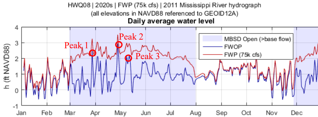
Figure 27: Daily averaged WSE timeseries for FWOP (V3PR1) and FWP (V3PR4) during the 2020s. Three peak events have been identified in red (top graph).
