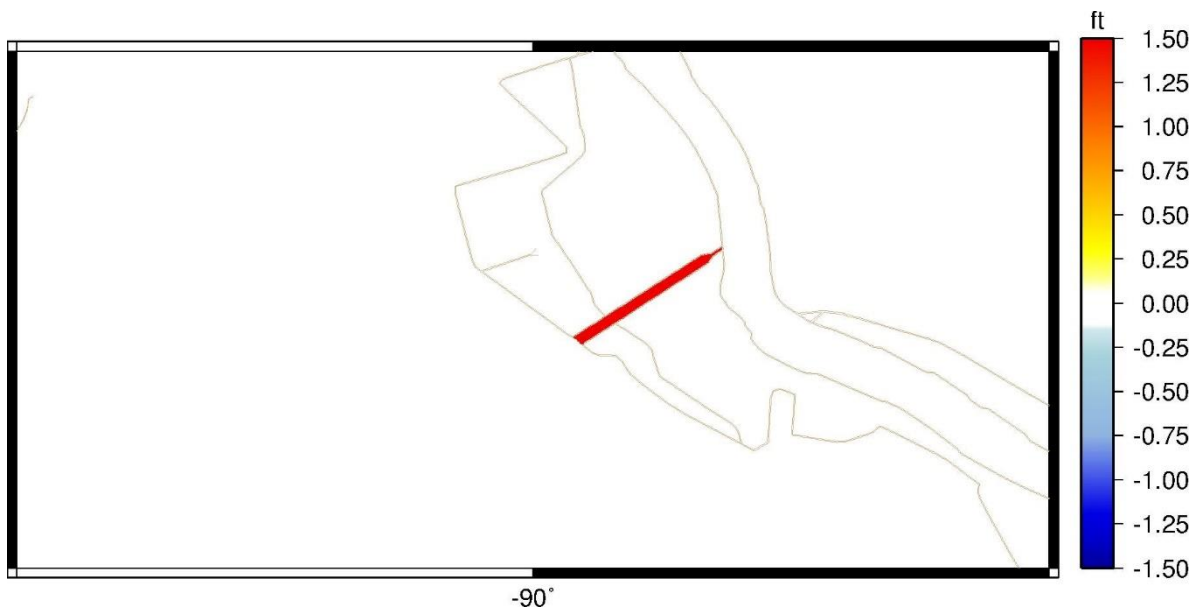
Figure 4-1. Change in Peak Water Levels During 1 Percent AEP Storm (Storm 009): 2070 Applicant's Preferred Alternative + Open Conveyance Channel Less 2070 Applicant's Preferred Alternative.
