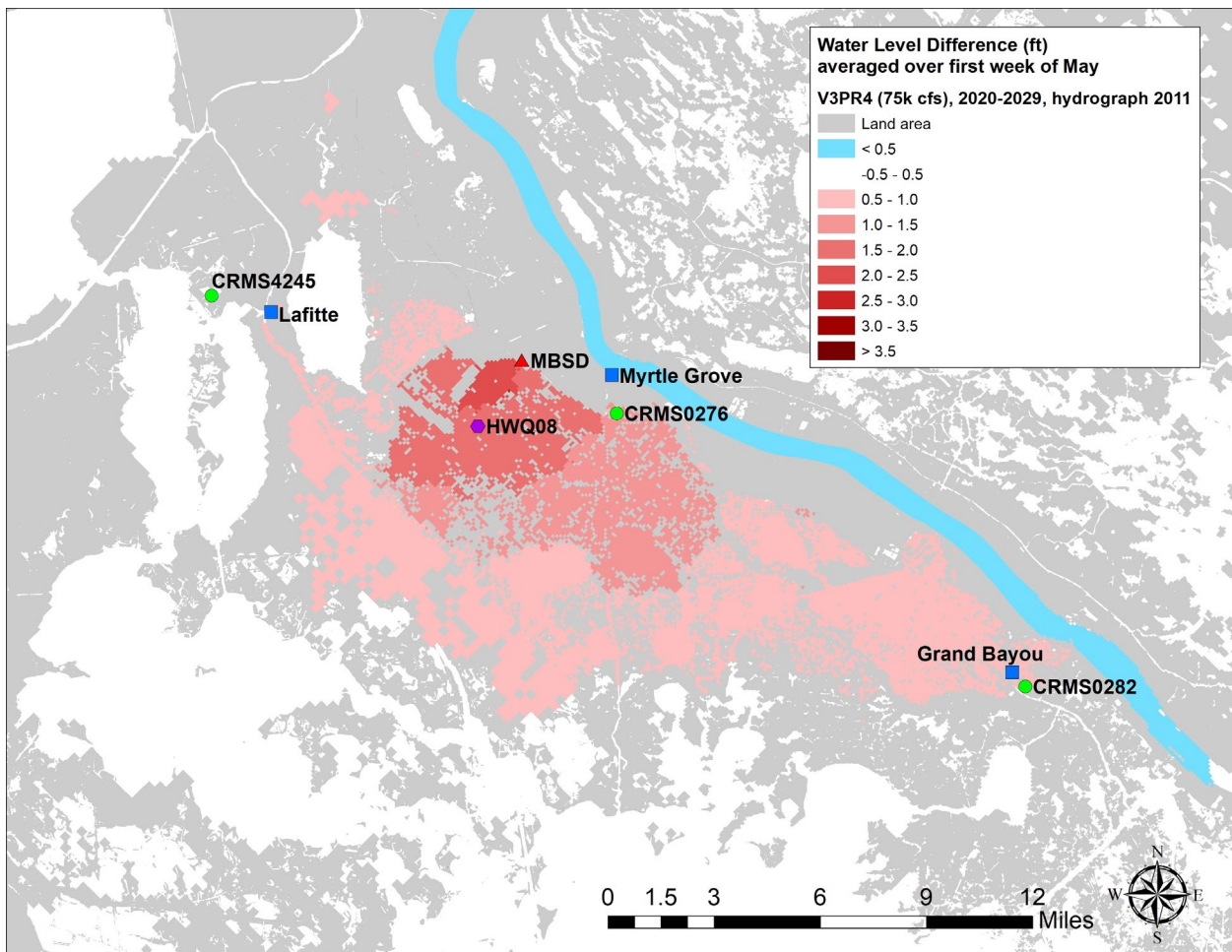
Figure 26: Average water level difference between FWOP (V3PR1) and FWP (V3PR4, 75k cfs) for the first week of May (in the 2020s), when the diversion is at maximum capacity (75k cfs).
