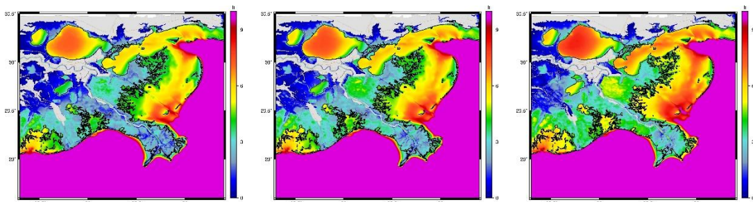
Figure 3-17. No Action Alternative maximum wave height for storm 239, 4 percent AEP storm, year 2020 (left), year 2040 (middle), year 2070 (right).
