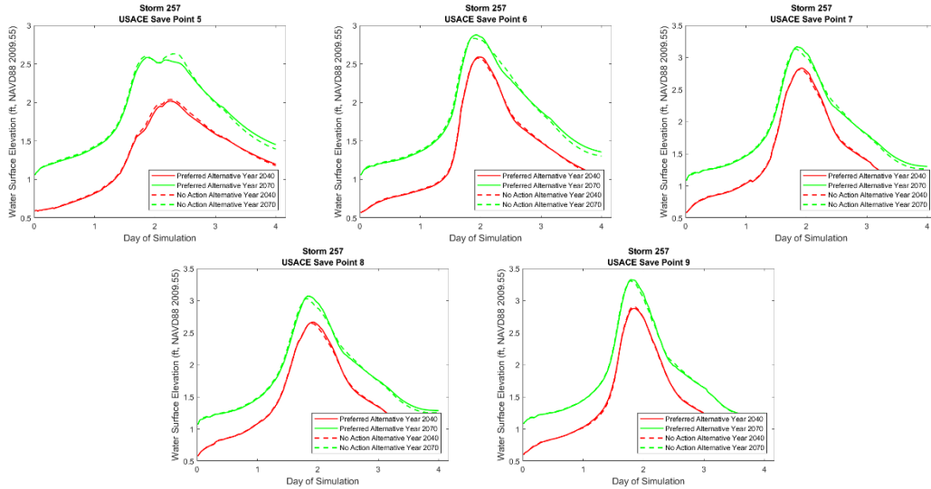
Figure 3-73. Hydrographs at selected save points near the LGM for storm 257, 4 percent AEP storm, showing water surface elevation for the No Action Alternative (red hashed 2040, green hashed 2070) and Applicant’s Preferred Alternative (red solid 2040, green solid 2070).
