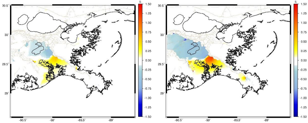
Figure 3-58. Maximum water surface elevation difference between the Applicant's Preferred Alternative and the No Action Alternative storm 257, 4 percent AEP storm, year 2040 (left), year 2070 (right).
