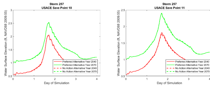
Figure 3-74. Hydrographs at selected save points near Grand Isle for storm 257, 4 percent AEP storm, showing water surface elevation for the No Action Alternative (red hashed 2040, green hashed 2070) and Applicant’s Preferred Alternative (red solid 2040, green solid 2070).
