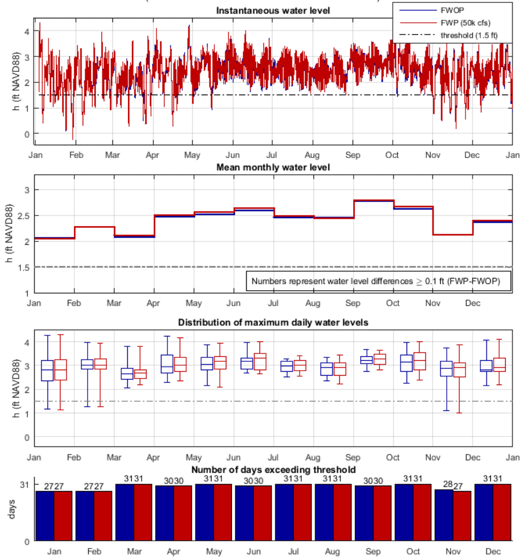
Figure C 9: Analysis of diversion impact on WSEs at Grand Bayou during the 2060s, FWOP and FWP (50k cfs), using the river hydrograph of year 2011. The top-most plot shows instantaneous water level (h). The second-from-the-top plot shows mean monthly water level (h). The third-from-the-top plot shows the distribution of maximum daily water levels (h) in box and whiskers plot format. The bottom plot shows the number of days exceeding the WSE threshold used for this community. Water level is referenced to NAVD88 (GEOID12A).
