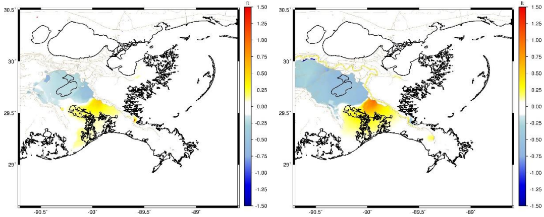
Figure 3-54. Maximum water surface elevation difference between the Applicant's Preferred Alternative and the No Action Alternative storm 239, 4 percent AEP storm, year 2040 (left), year 2070 (right).
