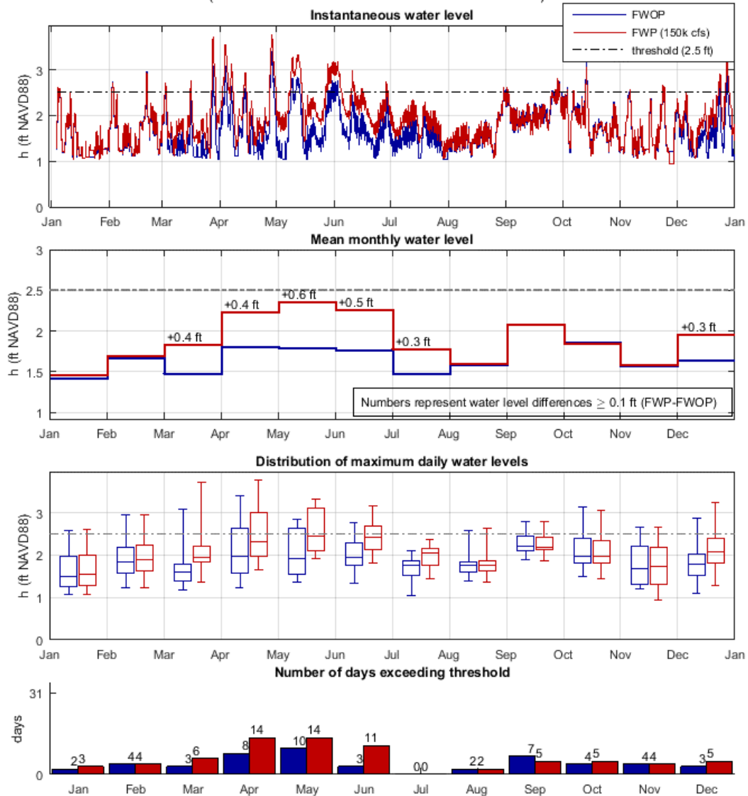
Figure C 15: Analysis of diversion impact on WSEs in Lafitte during the 2040s, FWOP and FWP (150k cfs), using the river hydrograph of year 2011. The top-most plot shows instantaneous water level (h). The second-from-the-top plot shows mean monthly water level (h). The third-from-the-top plot shows the distribution of maximum daily water levels (h) in box and whiskers plot format. The bottom plot shows the number of days exceeding the WSE threshold used for this community. Water level is referenced to NAVD88 (GEOID12A).
