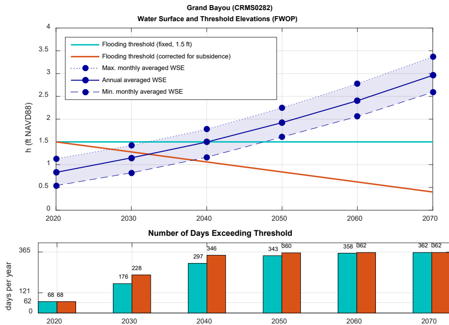
Figure 7: Analysis of the WSE in Grand Bayou over time, FWOP simulation, 2011 hydrograph. (Top graph) Annual average WSE (blue solid line) and its range of variation (min/max monthly average, blue dotted lines), fixed WSE thresholds (green line) and WSE threshold corrected with subsidence (orange line). (Bottom graph) Annual number of days exceeding the fixed WSE threshold elevation (green) and the corrected threshold elevation (orange). WSE is referenced to NAVD88 (GEOID12A).
