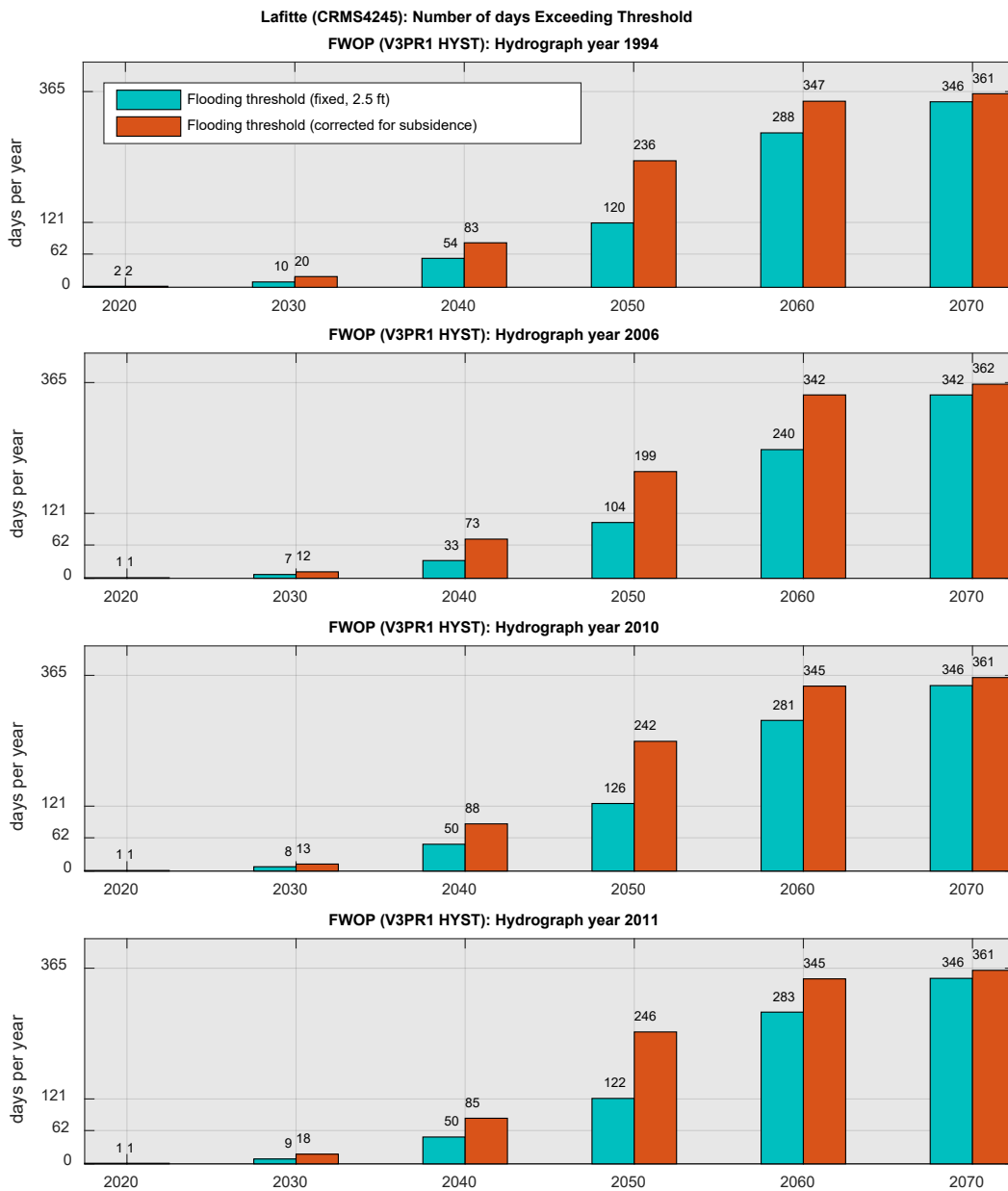
Figure 9: Analysis of the threshold exceedance rates in Lafitte over time, FWOP simulation, all hydrographs. Annual number of days exceeding the fixed WSE threshold elevation (green) and the threshold elevation corrected for subsidence (orange).
