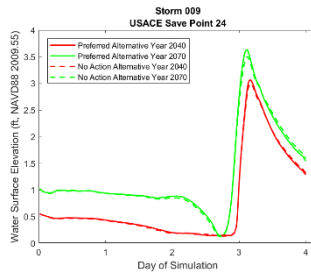
Figure 3-69. Hydrographs at a save point near Grand Bayou for storm 009, 1 percent AEP storm, showing water surface elevation for the No Action Alternative (red hashed 2040, green hashed 2070) and Applicant’s Preferred Alternative (red solid 2040, green solid 2070).
