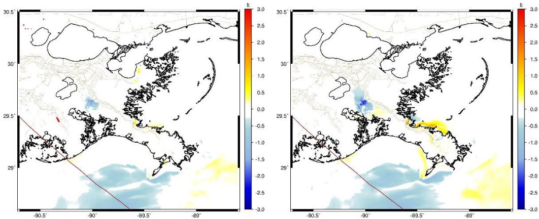
Figure 3-49. Maximum wave height difference between the Applicant's Preferred Alternative and the No Action Alternative for storm 093, 1 percent AEP storm, year 2040 (left), year 2070 (right).
