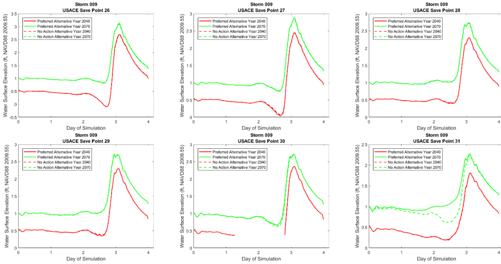
Figure 3-63. Hydrographs at selected save points along the NOV for storm 009, 1 percent AEP storm, showing water surface elevation for the No Action Alternative (red hashed 2040, green hashed 2070) and Applicant’s Preferred Alternative (red solid 2040, green solid 2070).
