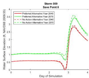
Figure 3-67. Hydrographs at a save point near Lafitte for storm 009, 1 percent AEP storm, showing water surface elevation for the No Action Alternative (red hashed 2040, green hashed 2070) and Applicant’s Preferred Alternative (red solid 2040, green solid 2070).
