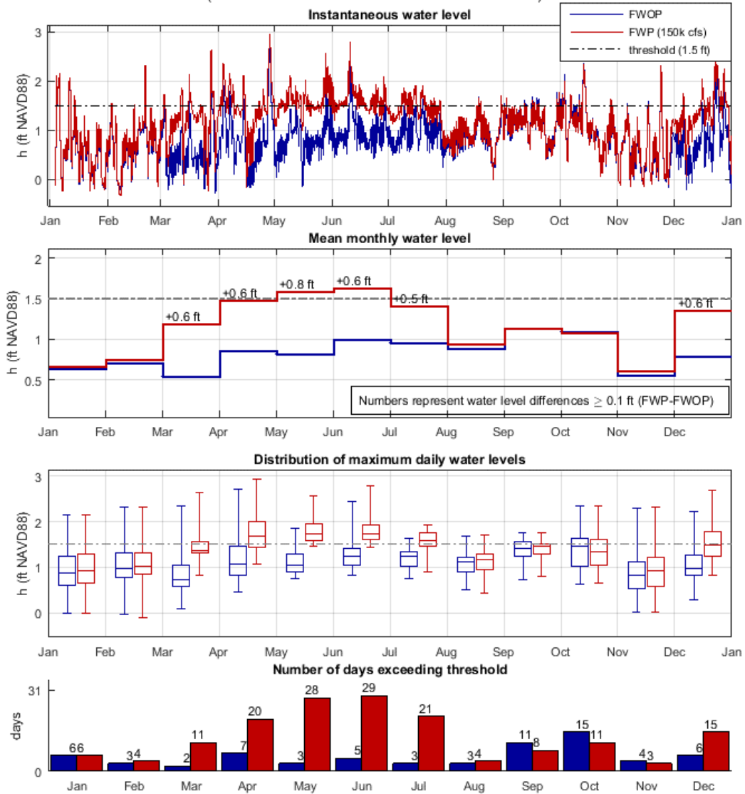
Figure C 13: Analysis of diversion impact on WSEs in Grand Bayou during the 2020s, FWOP and FWP (150k cfs), using the river hydrograph of year 2011. The top-most plot shows instantaneous water level (h). The second-from-the-top plot shows mean monthly water level (h). The third-from-the-top plot shows the distribution of maximum daily water levels (h) in box and whiskers plot format. The bottom plot shows the number of days exceeding the WSE threshold used for this community. Water level is referenced to NAVD88 (GEOID12A).
