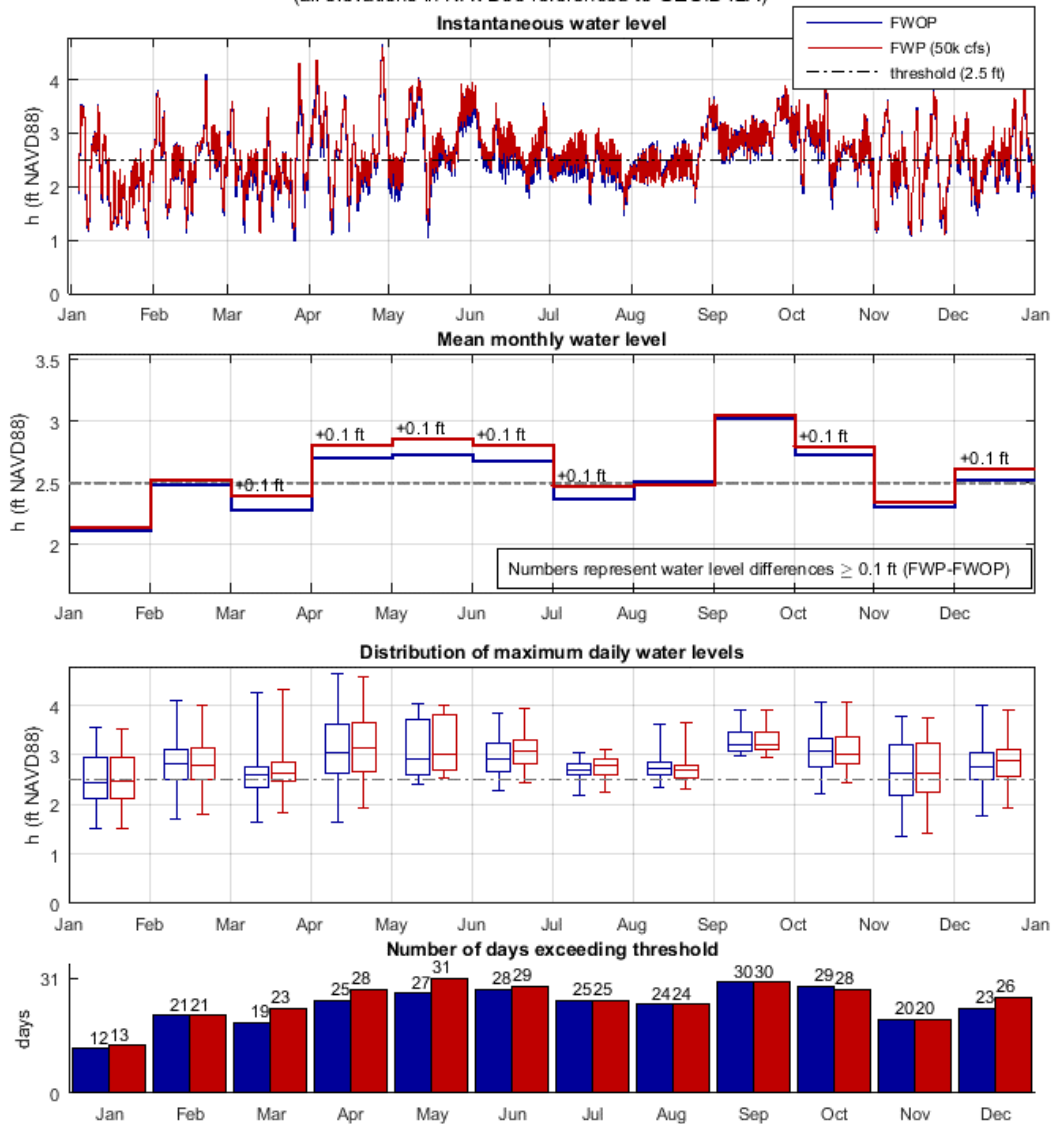
Figure C 8: Analysis of diversion impact on WSEs at Lafitte during the 2060s, FWOP and FWP (50k cfs), using the river hydrograph of year 2011. The top-most plot shows instantaneous water level (h). The second-from-the-top plot shows mean monthly water level (h). The third-from-the-top plot shows the distribution of maximum daily water levels (h) in box and whiskers plot format. The bottom plot shows the number of days exceeding the WSE threshold used for this community. Water level is referenced to NAVD88 (GEOID12A).
