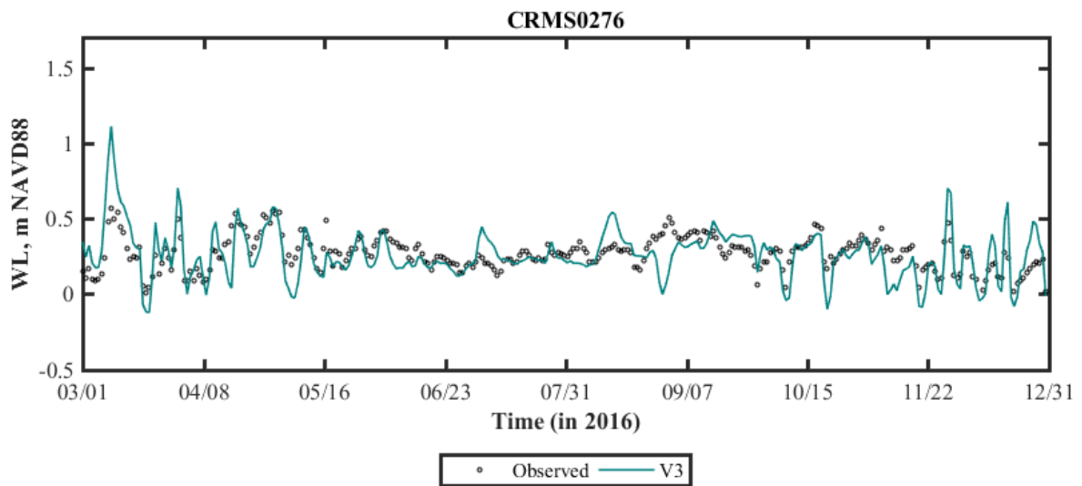
Figure B 4.V3 Basinwide model validation of daily water level (WL) at CRMS0276 (Myrtle Grove community), in Barataria Basin (2016).
