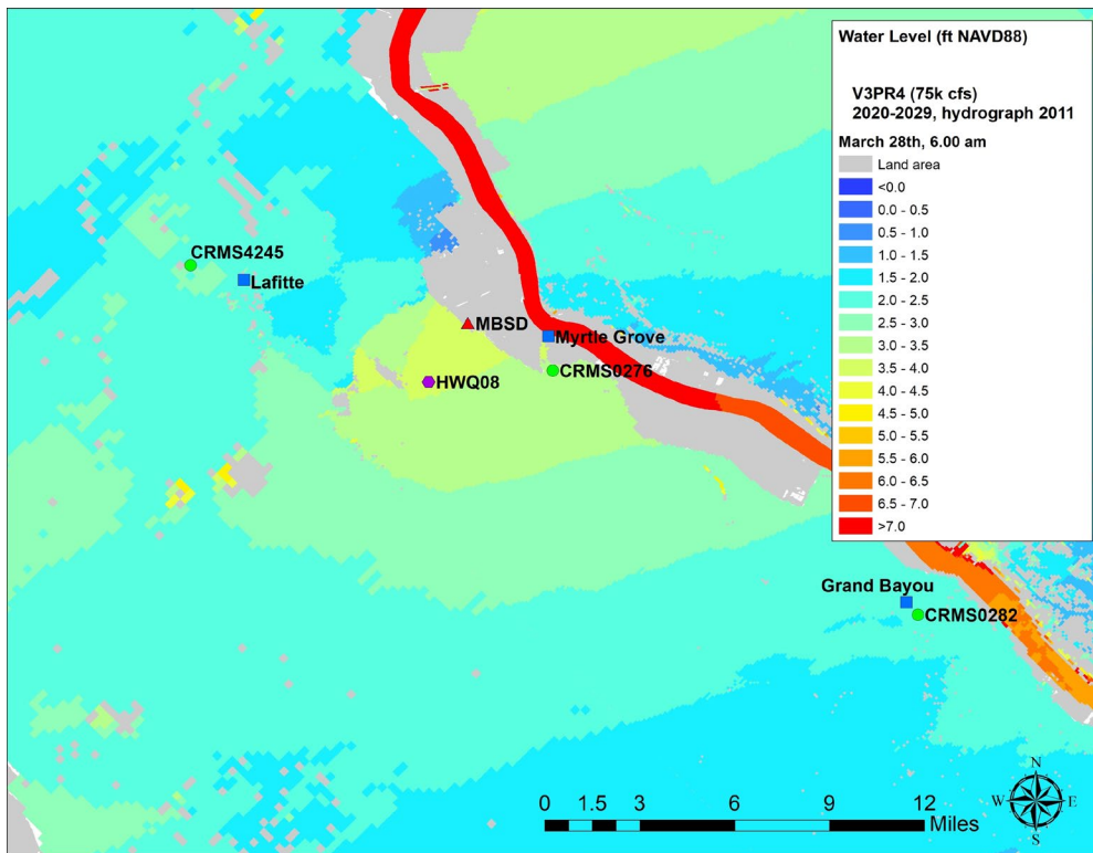
Figure 29: Instantaneous WSE for FWOP (V3PR1) during a wind driven peak event (Peak 1), during the 2020s.
