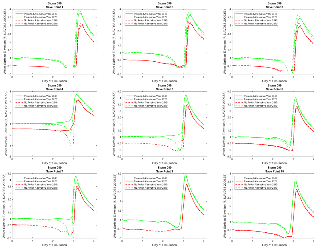
Figure 3-62. Hydrographs at selected save points along the NOV-NFL for storm 009, 1 percent AEP storm, showing water surface elevation for the No Action Alternative (red hashed 2040, green hashed 2070) and Applicant’s Preferred Alternative (red solid 2040, green solid 2070).
