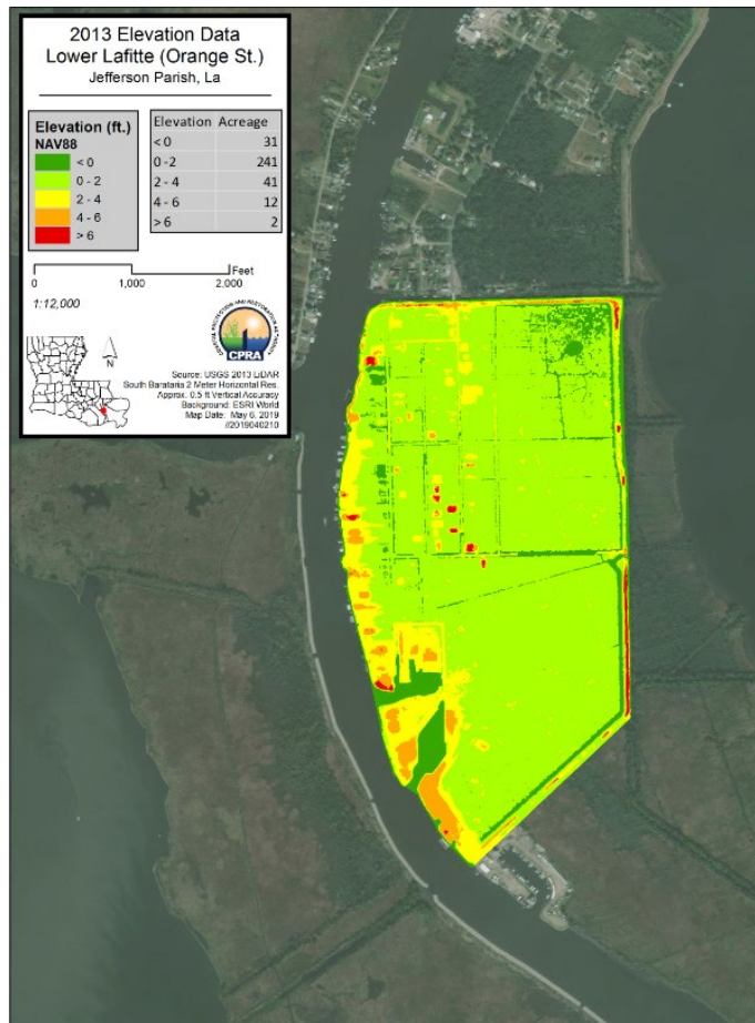
Figure A 5.2 USGS 2013 LiDAR (DEM) showing ground elevations at the Lower Lafitte basin. The ground elevations within the basin are largely in the range +0-2 ft NAVD88.
