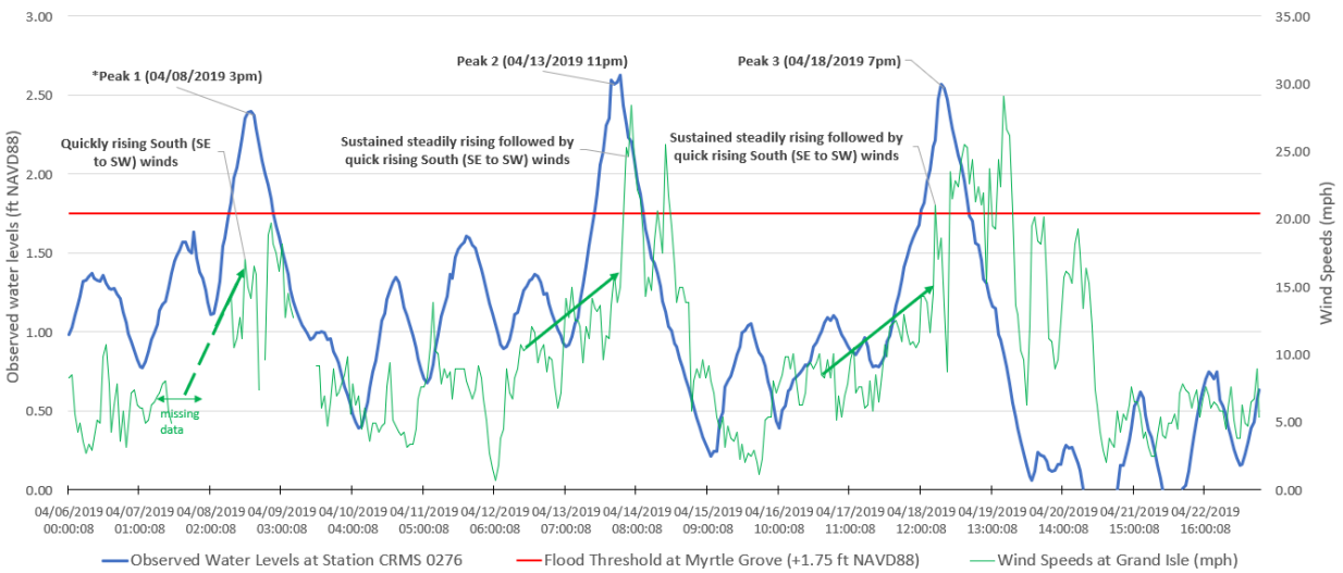
Figure A 3. Recent water level data at Myrtle Grove (Station CRMS0276) and wind speeds recorded at Grand Isle (Source NOAA) showing three wind tide peaks. *The first peak (April 8 th ) was a verification event when water levels were reported by the surveyor and CPRA personnel on site confirming +1.8-2.0 ft NAVD88. Site observation confirmed that flood threshold at +1.75 ft NAVD88 is appropriate to indicate initial flood event in this area.
