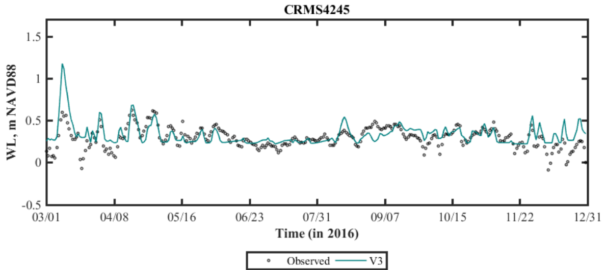
Figure B 5.V3 Basinwide model validation of daily water level (WL) at CRMS4245 (Lafitte community), in Barataria Basin (2016).
