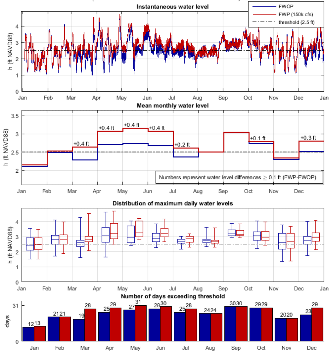
Figure C 18: Analysis of diversion impact on WSEs in Lafitte during the 2060s, FWOP and FWP (150k cfs), using the river hydrograph of year 2011. The top-most plot shows instantaneous water level (h). The second-from-the-top plot shows mean monthly water level (h). The third-from-the-top plot shows the distribution of maximum daily water levels (h) in box and whiskers plot format. The bottom plot shows the number of days exceeding the WSE threshold used for this community. Water level is referenced to NAVD88 (GEOID12A).
