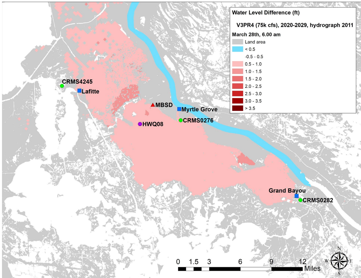
Figure 30: Difference in instantaneous WSEs for FWOP (V3PR1) and FWP (V3PR4, 75k cfs) during a wind driven peak event during the 2020s, on March 28 th , 2011 at 6 am.
