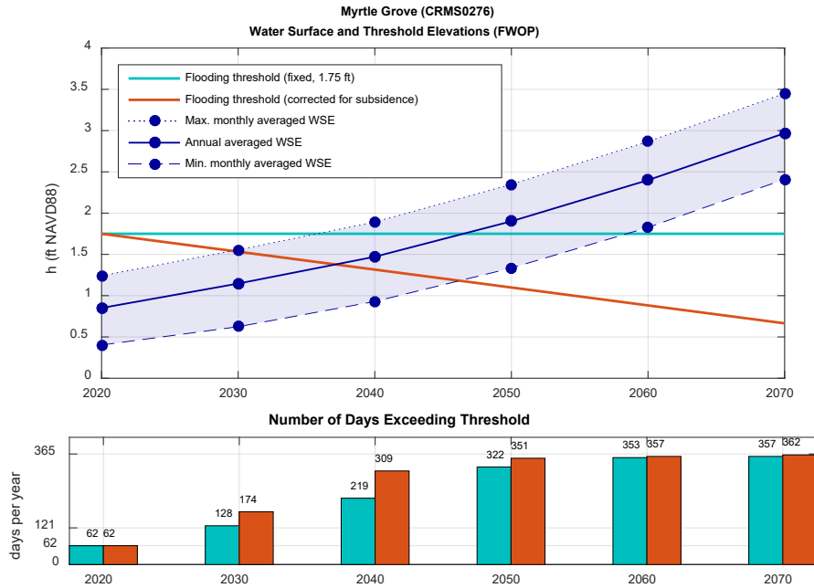
Figure 5: Analysis of the WSE in Myrtle Grove over time, FWOP simulation, 2011 hydrograph. (Top graph) Annual average WSE (blue solid line) and its range of variation (min/max monthly average, blue dotted lines), fixed WSE thresholds (green line) and WSE threshold corrected with subsidence (orange line). (Bottom graph) Annual number of days exceeding the fixed WSE threshold elevation (green) and the corrected threshold elevation (orange). WSE is referenced to NAVD88 (GEOID12A).
