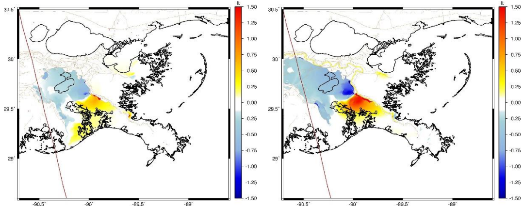
Figure 3-46. Maximum water surface elevation difference between the Applicant's Preferred Alternative and the No Action Alternative storm 014, 1 percent AEP storm, year 2040 (left), year 2070 (right).
