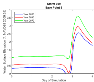
Figure 3-29. No Action Alternative Hydrographs at a save point near Lafitte for storm 009, 1 percent AEP storm, showing water surface elevation for year 2020 (blue), year 2040 (red), year 2070 (green).
