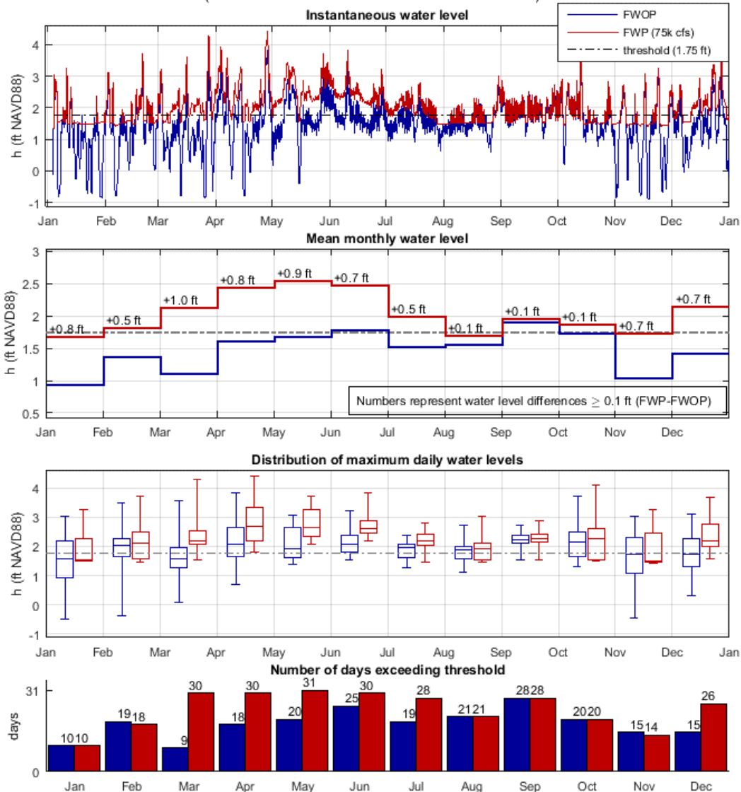
Figure 20: Analysis of diversion impact on WSEs in Myrtle Grove during the 2040s, FWOP and FWP (75k cfs), using the river hydrograph of year 2011. The top-most plot shows instantaneous water level (h). The second-from-the-top plot shows mean monthly water level (h). The third-from-the-top plot shows the distribution of maximum daily water levels (h) in box and whiskers plot format. The bottom plot shows the number of days exceeding the WSE threshold used for this community. Water level is referenced to NAVD88 (GEOID12A).
