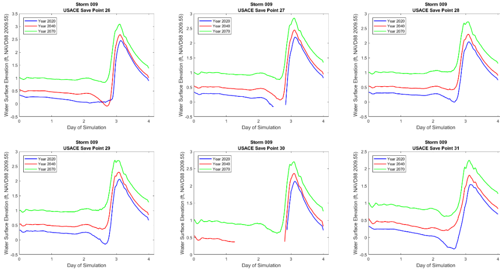
Figure 3-25. No Action Alternative Hydrographs at selected save points along the NOV for storm 009, 1 percent AEP storm, showing water surface elevation for year 2020 (blue), year 2040 (red), year 2070 (green).
