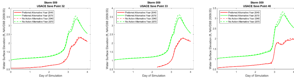
Figure 3-68. Hydrographs at selected save points near Des Allemandes/ Bayou Gauche for storm 009, 1 percent AEP storm, showing water surface elevation for the No Action Alternative (red hashed 2040, green hashed 2070) and Applicant’s Preferred Alternative (red solid 2040, green solid 2070).
