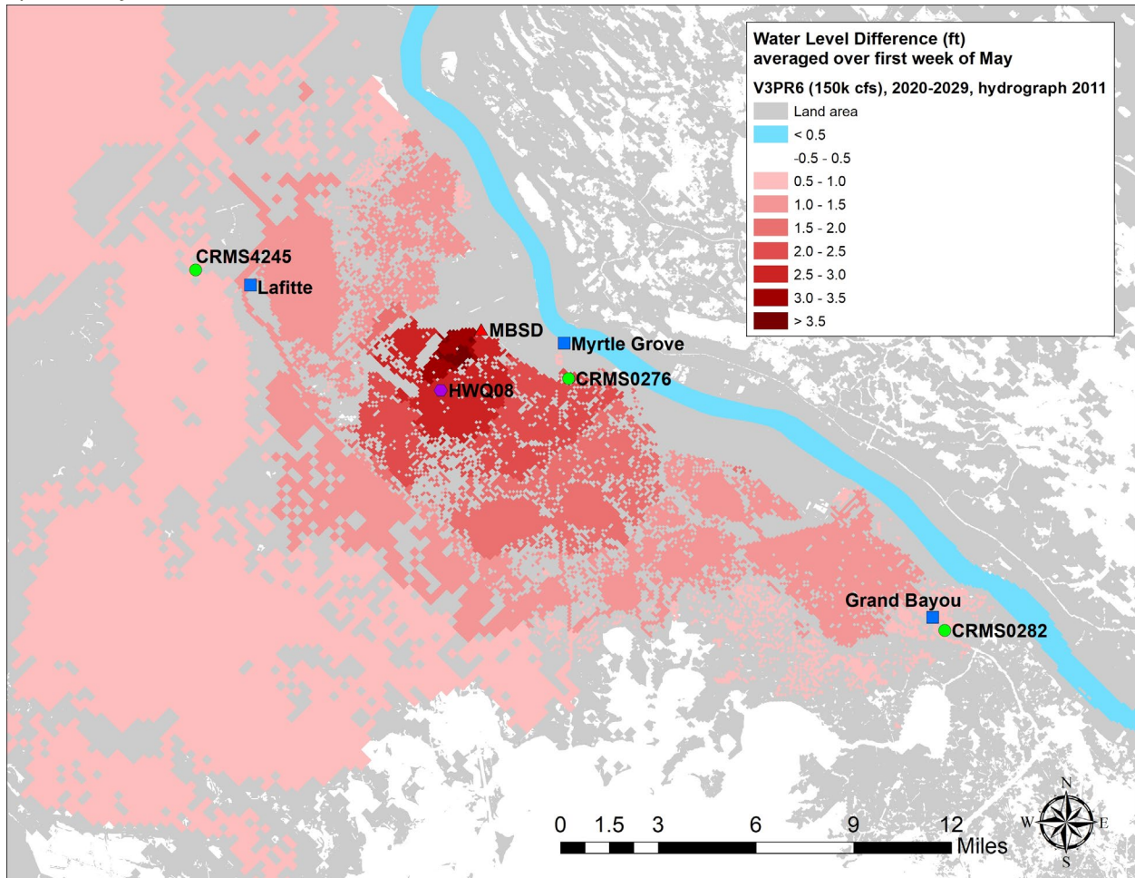
Figure C 20: Average water level difference between FWOP (V3PR1) and FWP (V3PR6, 150k cfs) for the first week of May (in the 2020s), when the diversion is at maximum capacity (150k cfs). 2011 hydrograph.
