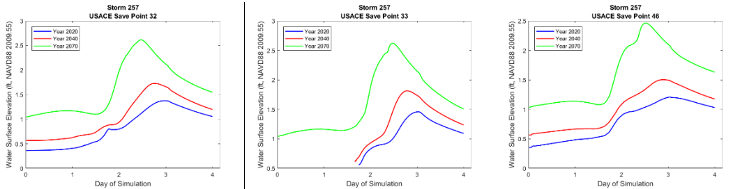
Figure 3-38. No Action Alternative Hydrographs at selected save points near Des Allemandes/ Bayou Gauche for storm 257, 4 percent AEP storm, showing water surface elevation for year 2020 (blue), year 2040 (red), year 2070 (green).
