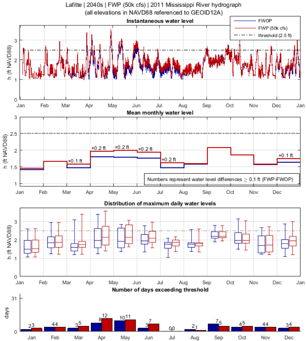
Figure C 5: Analysis of diversion impact on WSEs at Lafitte during the 2040s, FWOP and FWP (50k cfs), using the river hydrograph of year 2011. The top-most plot shows instantaneous water level (h). The second-from-the-top plot shows mean monthly water level (h). The third-from-the-top plot shows the distribution of maximum daily water levels (h) in box and whiskers plot format. The bottom plot shows the number of days exceeding the WSE threshold used for this community. Water level is referenced to NAVD88 (GEOID12A).
