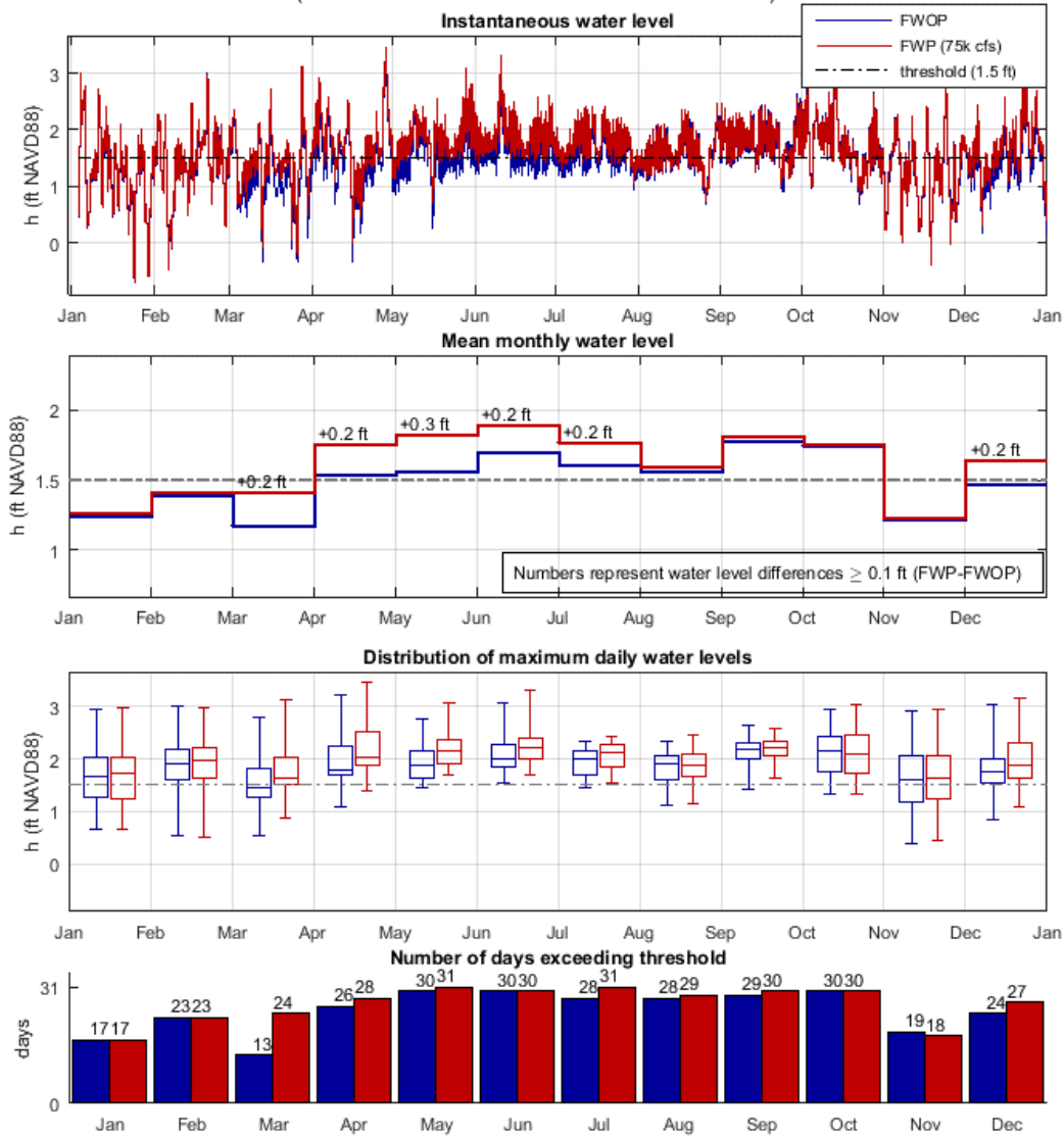
Figure 22: Analysis of diversion impact on WSEs in Grand Bayou during the 2040s, FWOP and FWP (75k cfs), using the river hydrograph of year 2011. The top-most plot shows instantaneous water level (h). The second-from-the-top plot shows mean monthly water level (h). The third-from-the-top plot shows the distribution of maximum daily water levels (h) in box and whiskers plot format. The bottom plot shows the number of days exceeding the WSE threshold used for this community. Water level is referenced to NAVD88 (GEOID12A).
