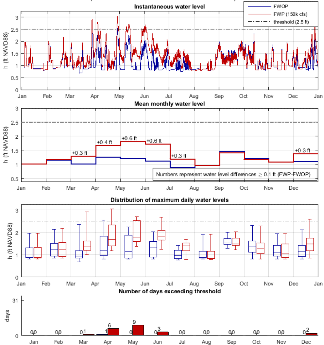
Figure C 12: Analysis of diversion impact on WSEs in Lafitte during the 2020s, FWOP and FWP (150k cfs), using the river hydrograph of year 2011. The top-most plot shows instantaneous water level (h). The second-from-the-top plot shows mean monthly water level (h). The third-from-the-top plot shows the distribution of maximum daily water levels (h) in box and whiskers plot format. The bottom plot shows the number of days exceeding the WSE threshold used for this community. Water level is referenced to NAVD88 (GEOID12A).
