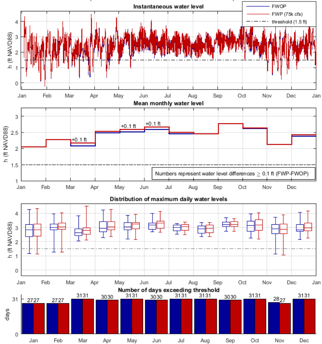
Figure 25. Analysis of diversion impact on WSEs in Grand Bayou during the 2060s, FWOP and FWP (75k cfs), using the river hydrograph of year 2011. The top-most plot shows instantaneous water level (h). The second-from-the-top plot shows mean monthly water level (h). The third-from-the-top plot shows the distribution of maximum daily water levels (h) in box and whiskers plot format. The bottom plot shows the number of days exceeding the WSE threshold used for this community. Water level is referenced to NAVD88 (GEOID12A).
