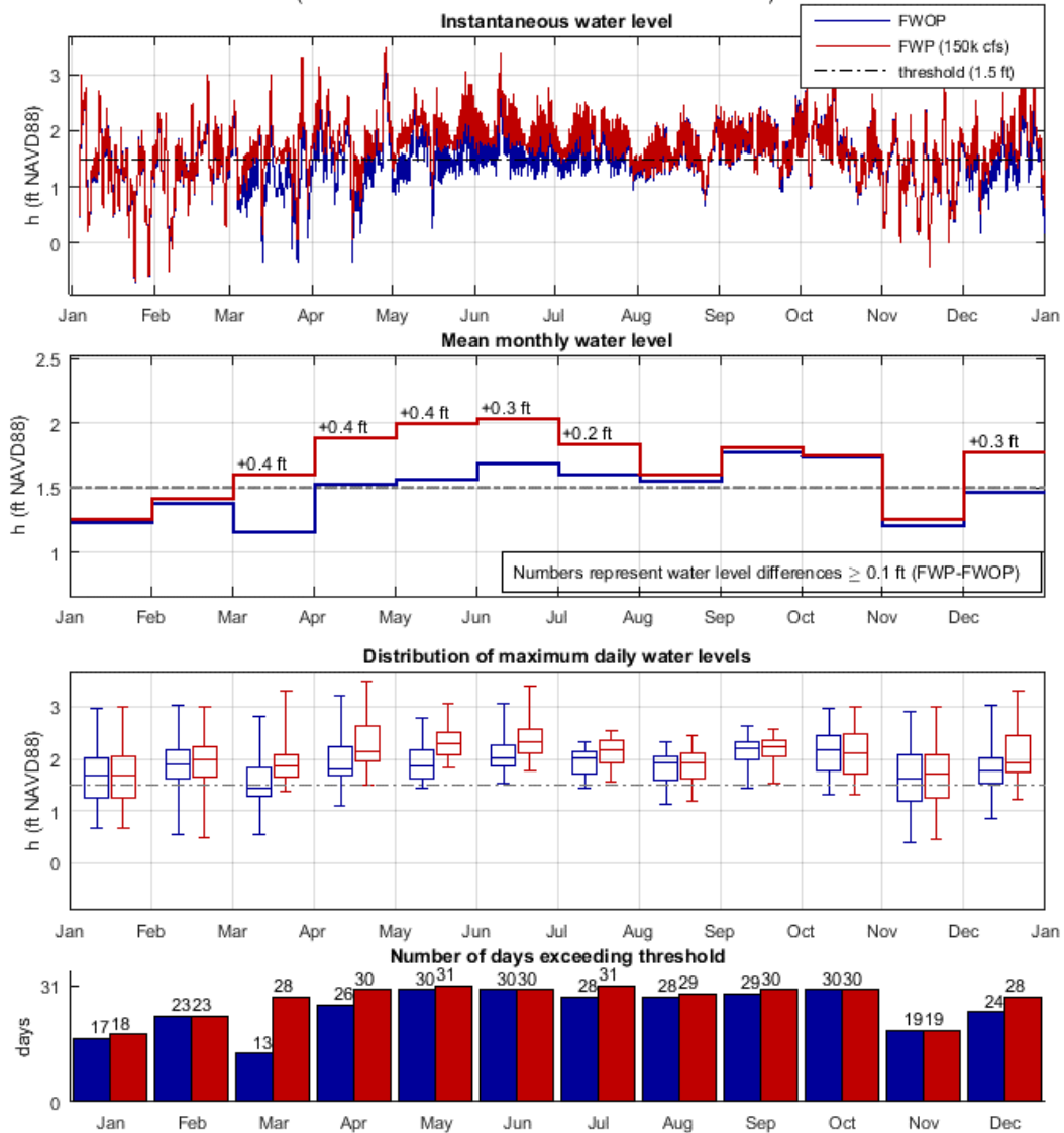
Figure C 16: Analysis of diversion impact on WSEs in Grand Bayou during the 2040s, FWOP and FWP (150k cfs), using the river hydrograph of year 2011. The top-most plot shows instantaneous water level (h). The second-from-the-top plot shows mean monthly water level (h). The third-from-the-top plot shows the distribution of maximum daily water levels (h) in box and whiskers plot format. The bottom plot shows the number of days exceeding the WSE threshold used for this community. Water level is referenced to NAVD88 (GEOID12A).
