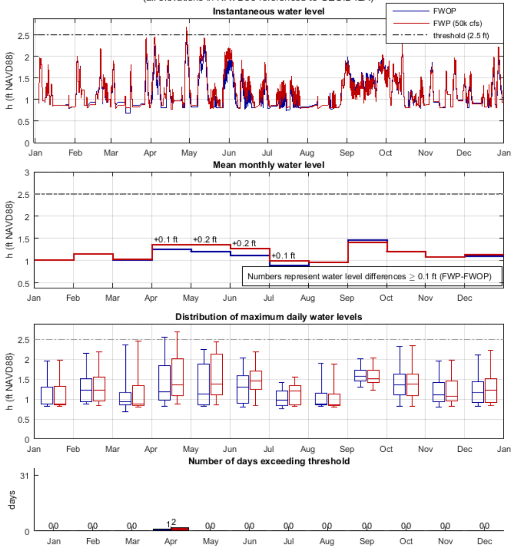
Figure C 2: Analysis of diversion impact on WSEs at Lafitte during the 2020s, FWOP and FWP (50k cfs), using the river hydrograph of year 2011. The top-most plot shows instantaneous water level (h). The second-from-the-top plot shows mean monthly water level (h). The third-from-the-top plot shows the distribution of maximum daily water levels (h) in box and whiskers plot format. The bottom plot shows the number of days exceeding the WSE threshold used for this community. Water level is referenced to NAVD88 (GEOID12A).
