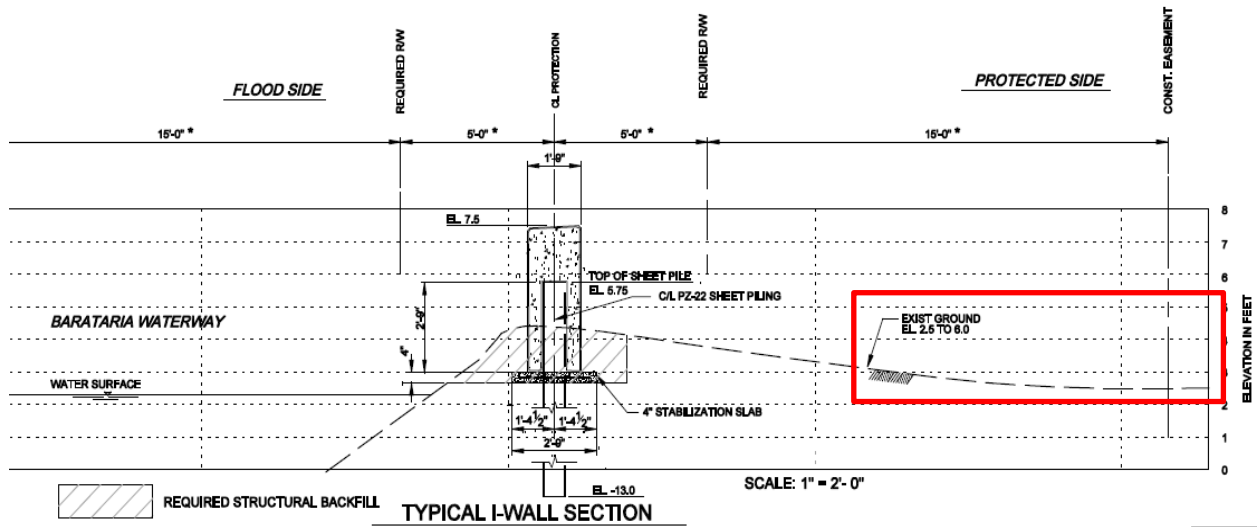
Figure A 5.1 Representative ground elevation of the Jean Lafitte tidal protection basin, indicating lower elevations subject to the onset of nuisance flooding, which correspond with approximately 2.5 ft (red frame).
