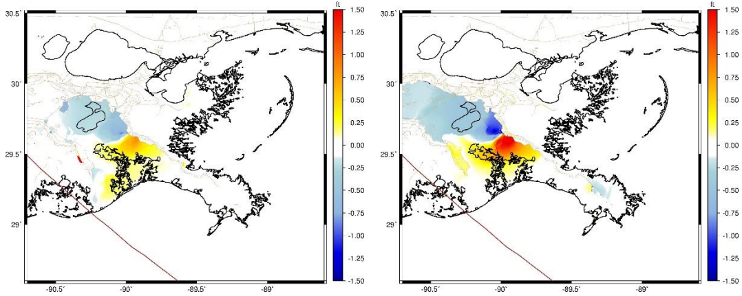
Figure 3-48. Maximum water surface elevation difference between the Applicant's Preferred Alternative and the No Action Alternative storm 093, 1 percent AEP storm, year 2040 (left), year 2070 (right).
