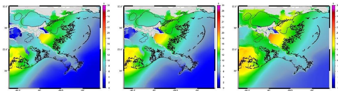
Figure 3-2. No Action Alternative maximum water surface elevation for storm 009, 1 percent AEP storm, year 2020 (left), year 2040 (middle), year 2070 (right).
