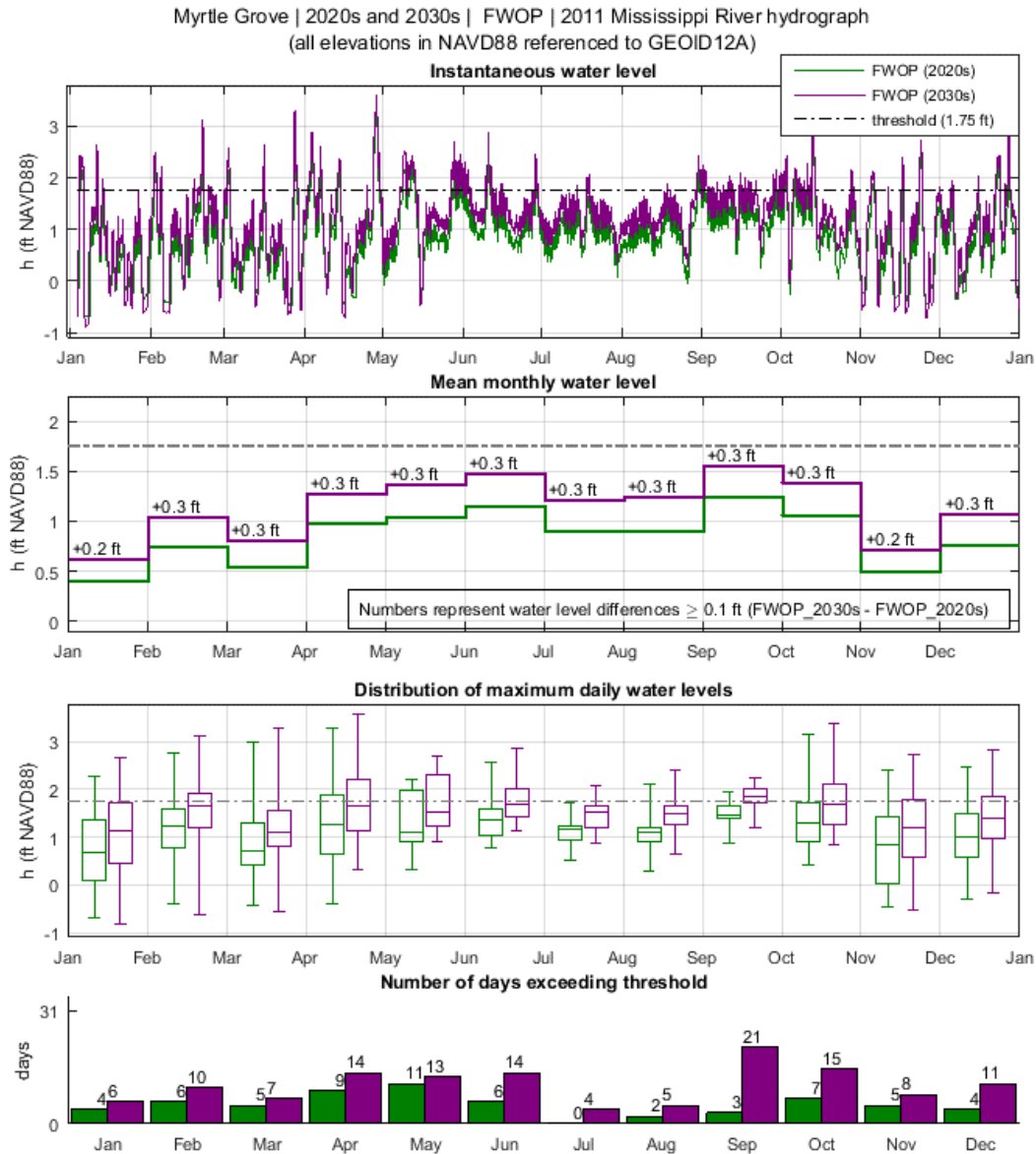
Figure 11: WSE analysis for Myrtle Grove, FWOP for the first decade (2020s, in green) and the second decade (2030s, in purple), using the hydrograph of year 2011. The top-most plot shows instantaneous water level (h). The second-from-the-top plot shows mean monthly water level (h). The third-from-the-top plot shows the distribution of maximum daily water levels (h) in box and whiskers plot format. The bottom plot shows the number of days exceeding the WSE threshold used for this community. Water level is referenced to NAVD88 (GEOID12A).
