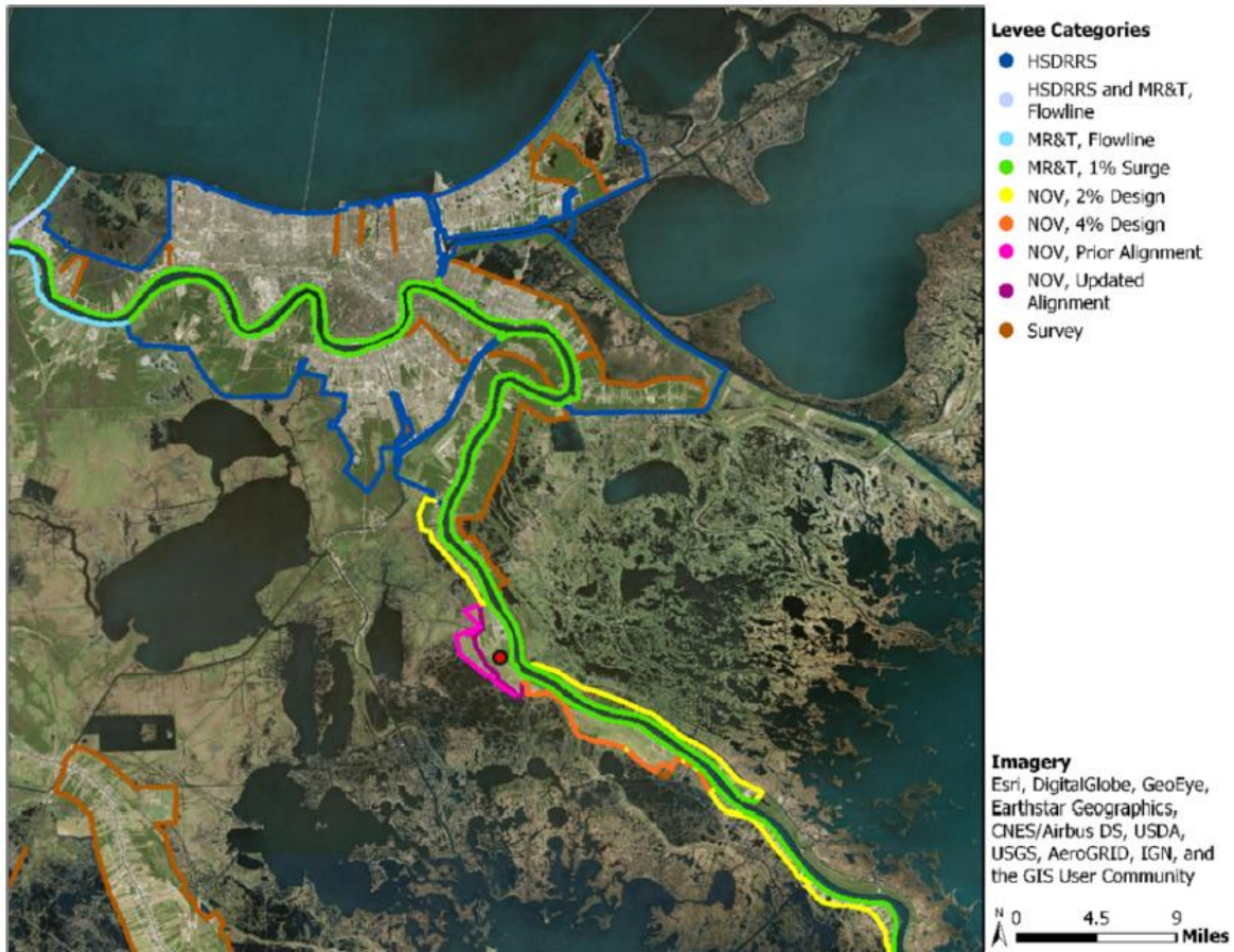
Figure 2-6. Levee Data Sources Used in ADCIRC+SWAN Model.
