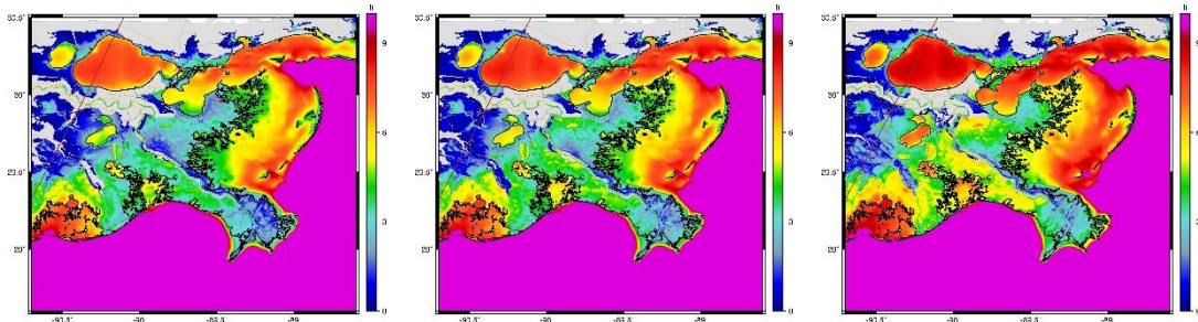
Figure 3-15. No Action Alternative maximum wave height for storm 160, 1 percent AEP storm, year 2020 (left), year 2040 (middle), year 2070 (right).
