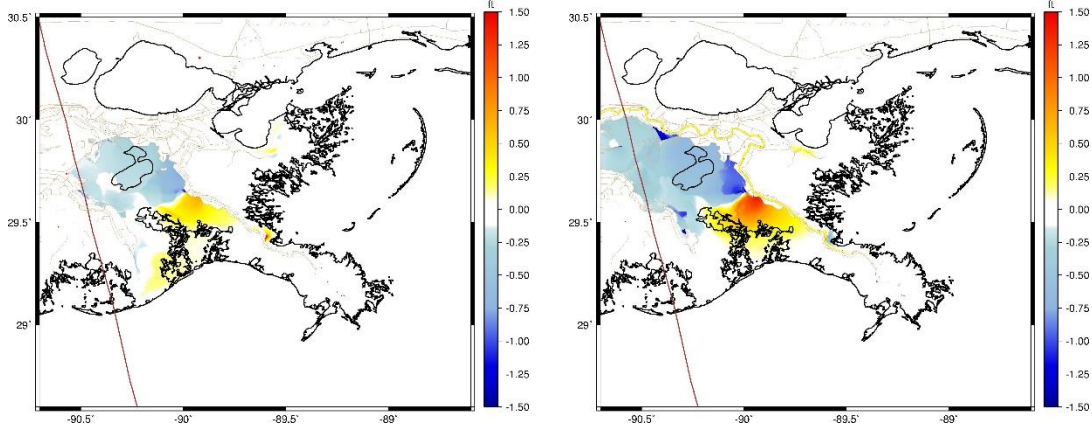
Figure 3-42. Maximum water surface elevation difference between the Applicant's Preferred Alternative and the No Action Alternative storm 011, 4 percent AEP storm, year 2040 (left), year 2070 (right).
