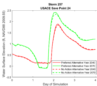
Figure 3-77. Hydrographs at a save point near Grand Bayou for storm 257, 4 percent AEP storm, showing water surface elevation for the No Action Alternative (red hashed 2040, green hashed 2070) and Applicant’s Preferred Alternative (red solid 2040, green solid 2070).
