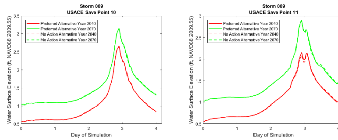
Figure 3-66. Hydrographs at selected save points near Grand Isle for storm 009, 1 percent AEP storm, showing water surface elevation for the No Action Alternative (red hashed 2040, green hashed 2070) and Applicant’s Preferred Alternative (red solid 2040, green solid 2070).
