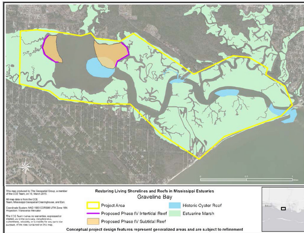
Figure 3. Graveline Bay Project Component and Submerged Aquatic Vegetation, National Wetland Inventory, and Oyster Locations
