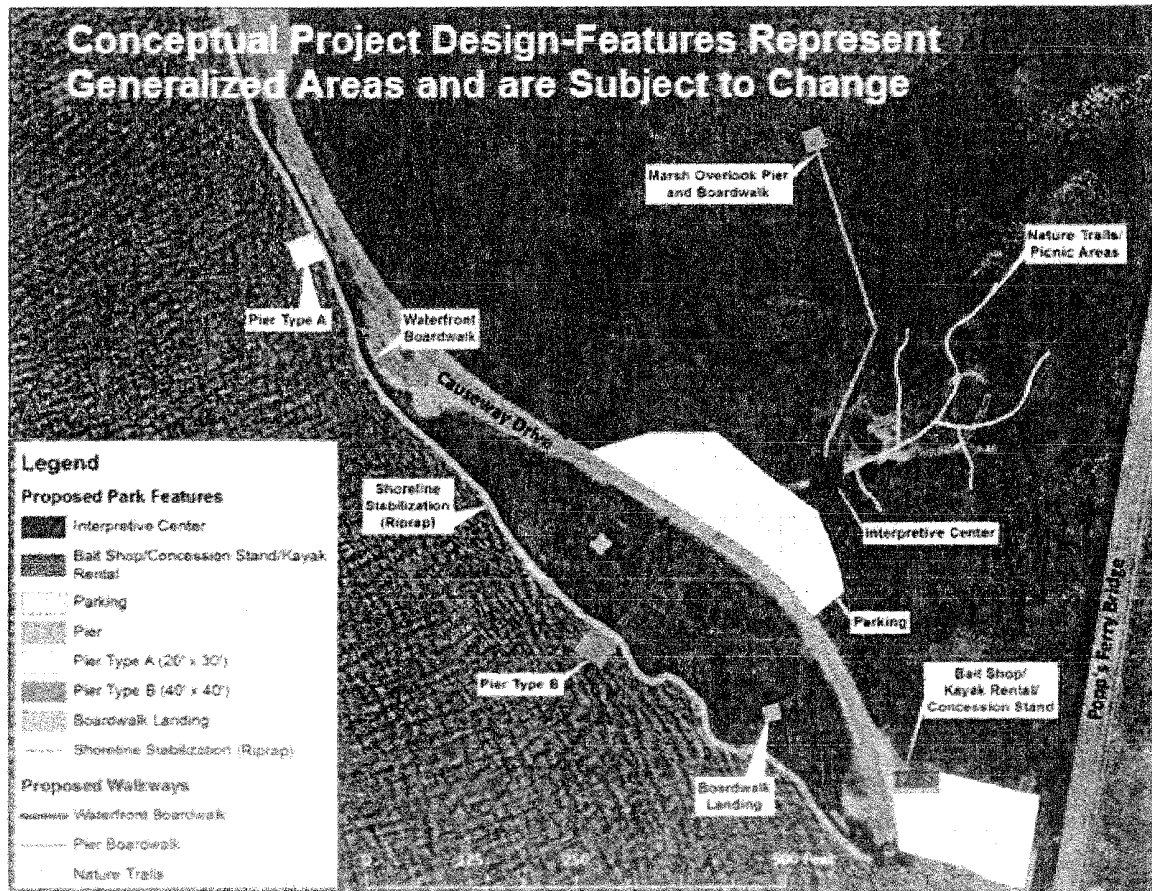
Figure 3- 2 - Popp's Ferry Causeway Park project features-Conceptual Plan.
