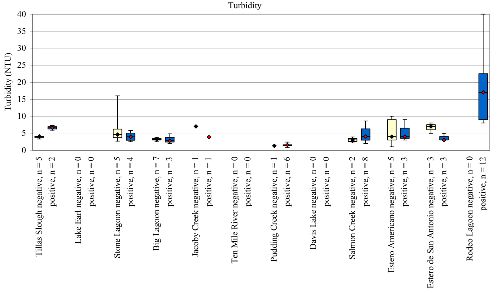
Figure A-17. Turbidity measured during sampling conducted 1996 for all waters with confirmed detection of tidewater goby. Boxes represent first and third quartiles, diamond markers represent median, and whiskers indicate the range. Negative detection sites are represented by a light box and black median marker; sites with positive detection are represented by dark blue box and red median marker.
