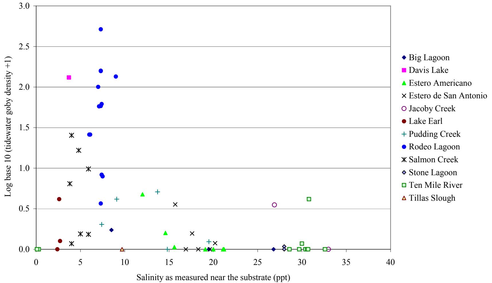
Figure 3. Tidewater goby density for 1996 seine samples transformed by \text{Log}_{10}(\text{density} + 1) and plotted against bottom salinity.
