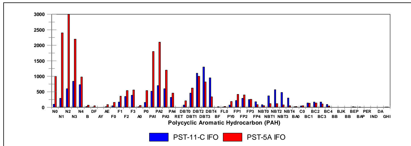
Figure 1. PAH distributions of the two primary fuel oils released from the M/V Selendang Ayu .
